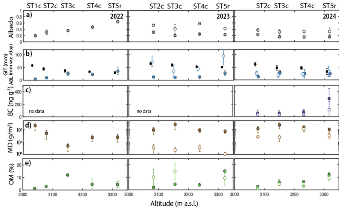
Figure 5. Altitudinal distribution of BB albedo a), granular ice thickness (GIT), ablation rate (ABL) b), black carbon (BC) c), mineral dust (MD) d), organic matter ratio (OM%) e). Open circle represents the clean area, while a filled circle indicates the dark area in 2023 and 2024. In panel b), black circles indicate ABL, and blue open circles and blue filled circles denote GIT in the clean and dark areas, respectively. The vertical axis of MD d) is logarithmic. Vertical error bars indicate the standard deviations of each multiple measurement. In 2022, sampling was not conducted separately in dark and clean areas. For 2023 and 2024, filled circles represent data from dark surface areas, whereas open circles represent data from clean surface areas.
