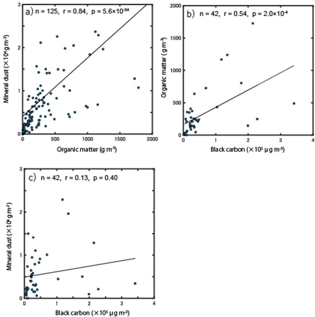
Figure 10. Relationships among the concentrations of the three major light-absorbing particles on the glacier surface: a) mineral particles and organic matter; b) black carbon and organic matter; c) black carbon and mineral particles. Note that black carbon was sampled only in 2024, so there are only 42 samples.
