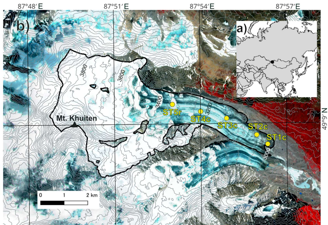
Figure 1. Location map of the Potanin Glacier a) and observed stake location at the Potanin Glacier b). The edges of the Potanin glacier are outlined in black. Contour lines are drawn at 50 m intervals. Yellow numbers indicate the location of stake, sampling site. The back satellite imagery is Sentinel 2 (False color) acquired on 15 July 2023.
