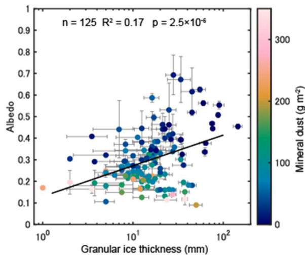
Figure 8. Relation between BB albedo and granular ice thickness (GIT). The circle colour indicates the amount of mineral dust per area.
