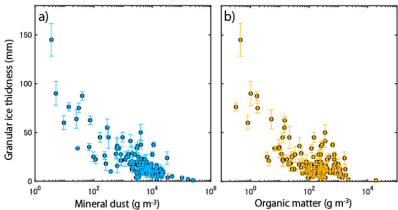
Figure 9. Relation between granular ice thickness and mineral dust concentration a) and organic matter
