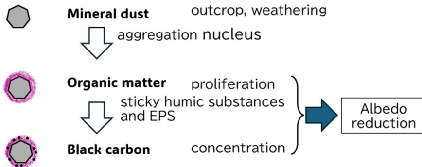
Figure 11. Schematic diagram showing the relationship between the three major LAIAPs (MD, OM, BC).
