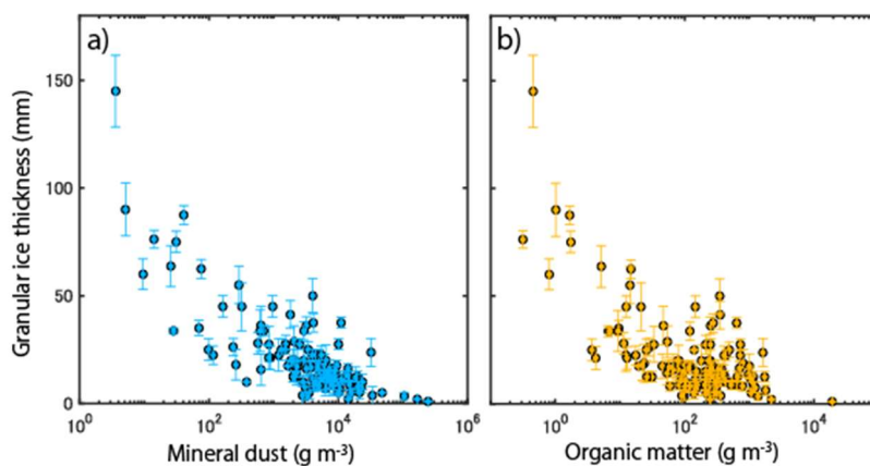
Figure 9. Relation between granular ice thickness and mineral dust concentration a) and organic matter concentration b).
