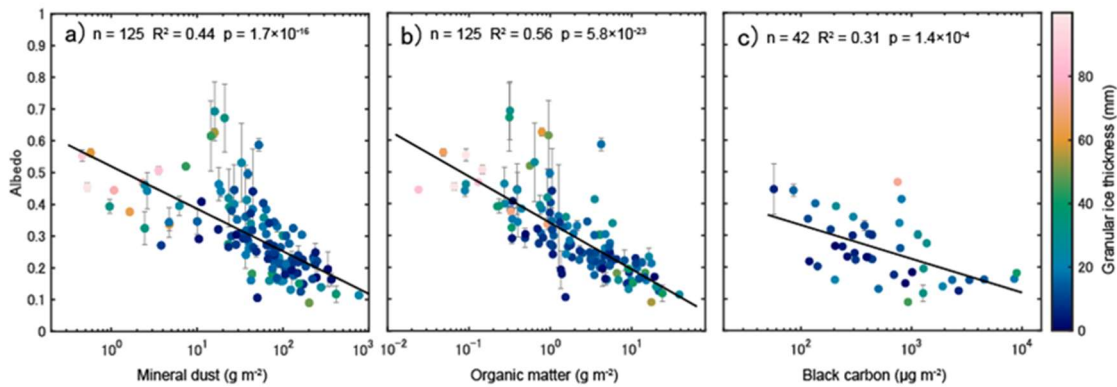
Figure 7. Relation between BB albedo and impuritiesparticles (MD, OM, BC) a)-c). The colour of the circle indicates surface granular ice thickness. All horizontal axes are logarithmic.
