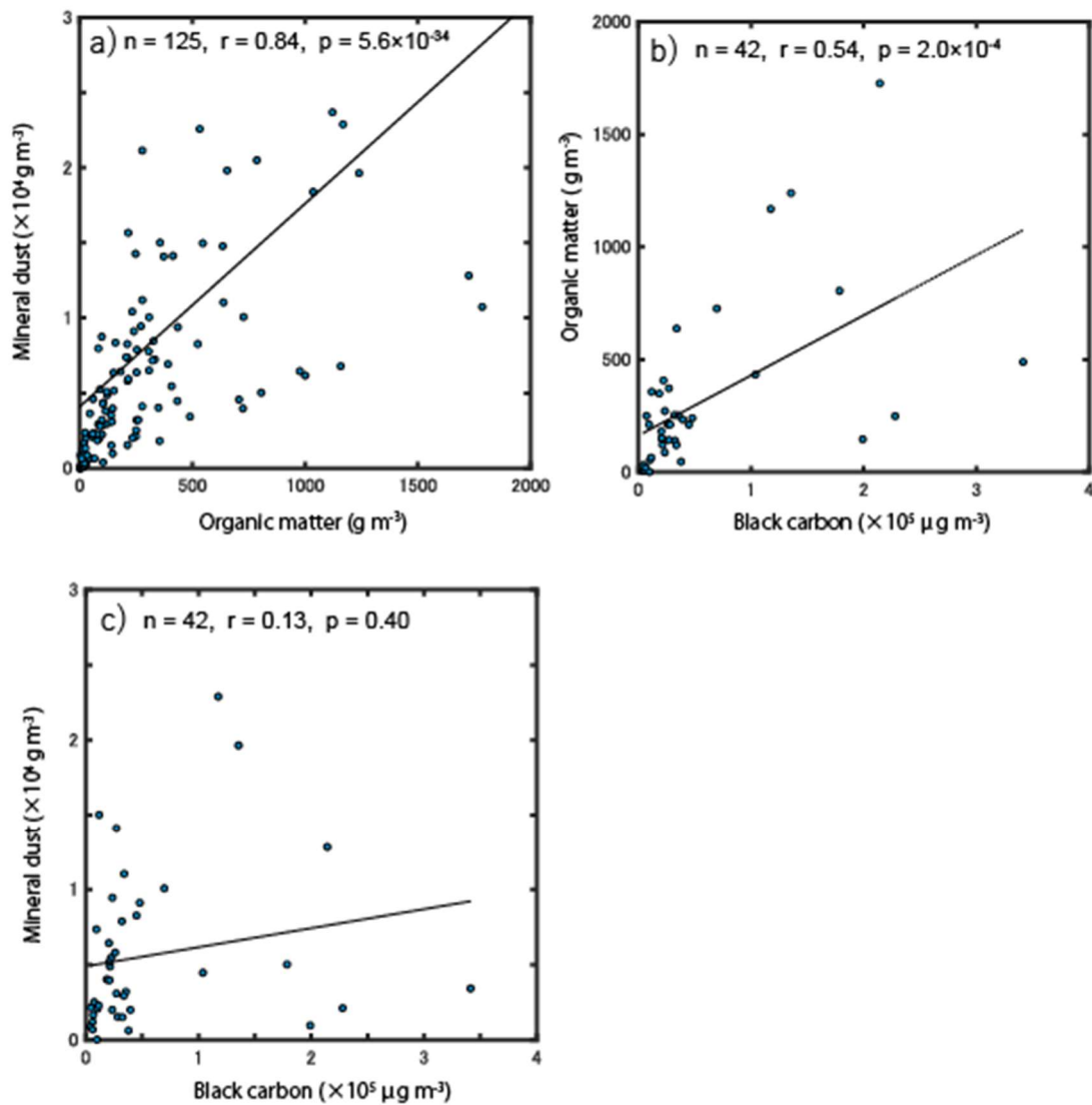
Figure 10. Relationships among the concentrations of the three major light-absorbing impurities on the glacier surface: a) mineral particles and organic matter; b) black carbon and organic matter; c) black carbon and mineral particles. Note that black carbon was sampled only in 2024, so there are only 42 samples.
