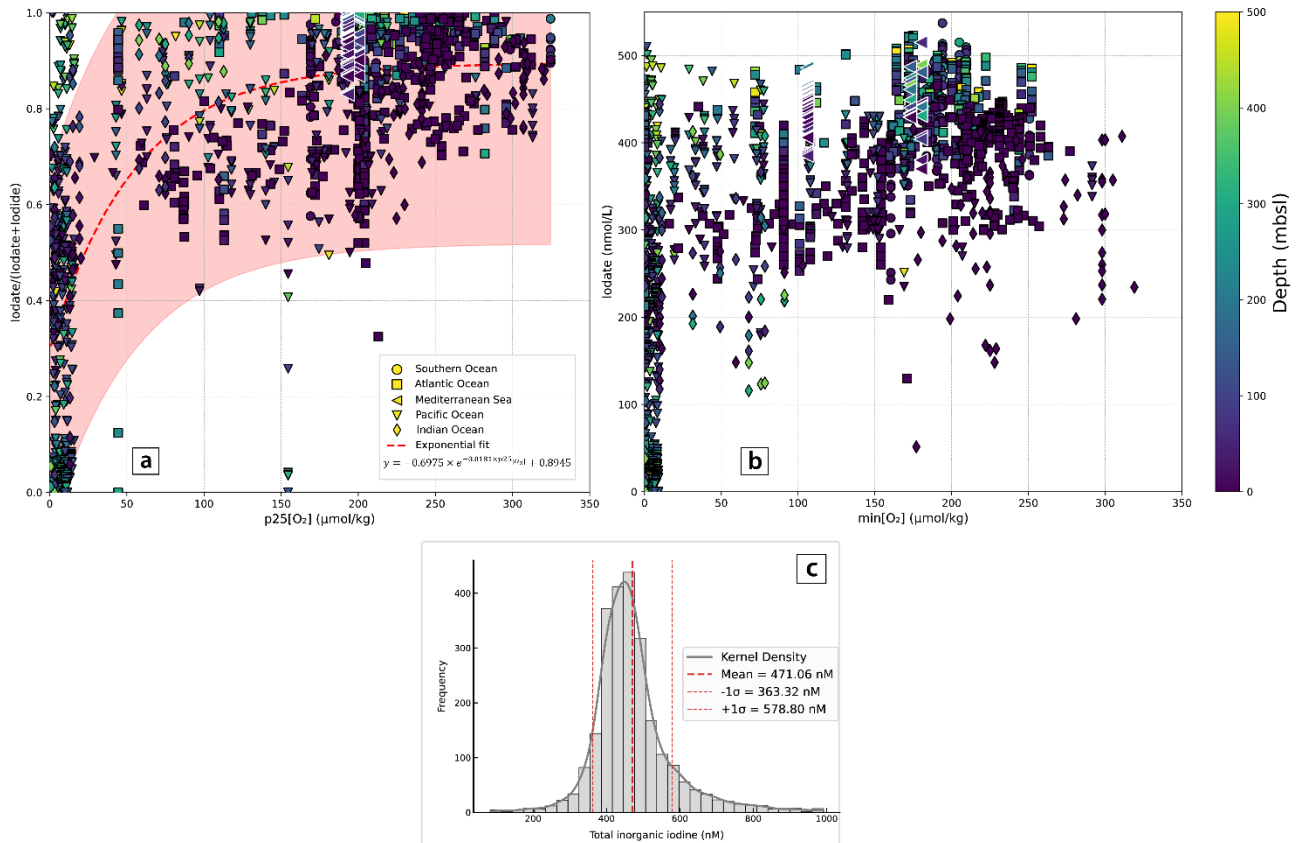
283 Figure 3: Iodate proportion in total inorganic iodine, iodate/(iodate+iodide) in 0–500 m as a function of p25 (a) 284 (Spearman \rho = 0.625 , Kendall \tau = 0.447 , p-values <0.01) and iodate concentration as a function of minimum (b) 285 (Spearman \rho = 0.650 , Kendall \tau = 0.470 , p-values <0.01) [O 2 ] (µmol/kg) at 0–500 m. The proportion of iodate in 286 inorganic iodine was obtained from Winkelbauer et al. (2023) and are classified by ocean. Mediterranean sites are 287 highlighted with white contour. Red dotted line is the exponential fit of this relation ( y = -0.6975 \cdot \exp(-0.0181 \cdot x) + 0.8945 for p25), with the 95% prediction interval filled in red. Total inorganic iodine distribution with mean and 288 \pm 1\sigma values (c). 289
