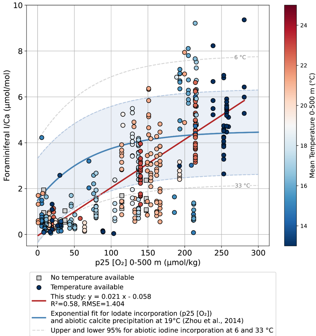
Figure 6: Foraminiferal I/Ca < 2 ka BP as a function of p25 [ \text{O}_2 ] in 0–500 m. The red line is the linear model proposed in this study. Blue curve represents the abiotic incorporation of iodine following iodate proportion in total inorganic iodine determined in Figure 3 and assuming a mean concentration of total inorganic iodine of 471 nM (Fig. 3c). The abiotic incorporation was determined following Zhou et al. (2014). Blue area corresponds to 95% prediction interval also determined in Figure 4 for a temperature of 19 °C. 61% of the data fall in this prediction interval. Temperature from 6 to 33 °C are considered for the maximum and minimum 95% prediction interval (grey dashed lines).
