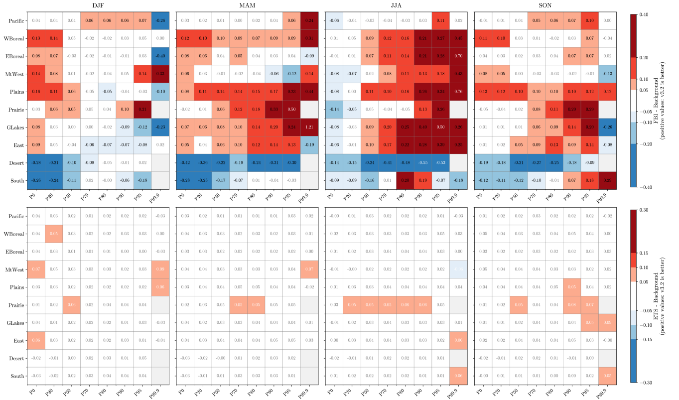
Figure 5. Improvement (red) or degradation (blue) in the Frequency Bias Index (FBI, top row) and Equitable Threat Score (ETS, bottom row) of the precipitation background field from CaSR v3.2 relative to CaSR v2.1, across Bukovsky regions and percentile-based precipitation thresholds. The top panels show |FBI_{v2.1} - 1| - |FBI_{v3.2} - 1| , where positive values indicate a reduction in the frequency bias in v3.2, while the bottom panels show ETS_{v3.2} - ETS_{v2.1} . Each column corresponds to a season (DJF, MAM, JJA, SON). Gray cells indicate insufficient data to compute the scores.
