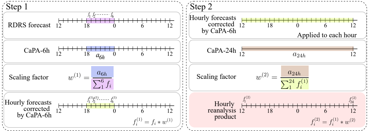
Figure 3. Step 1 (left) illustrates the temporal disaggregation of CaPA-6h using RDRS hourly forecasts. Step 2 (right) shows how the CaPA-24h analysis is further disaggregated using the Step 1 output to generate the hourly reanalysis distributed to the public. Here, a_{6h} and a_{24h} denote the 6-hour and 24-hour CaPA analyses, respectively, and f_i represents the RDRS hourly forecasts.
