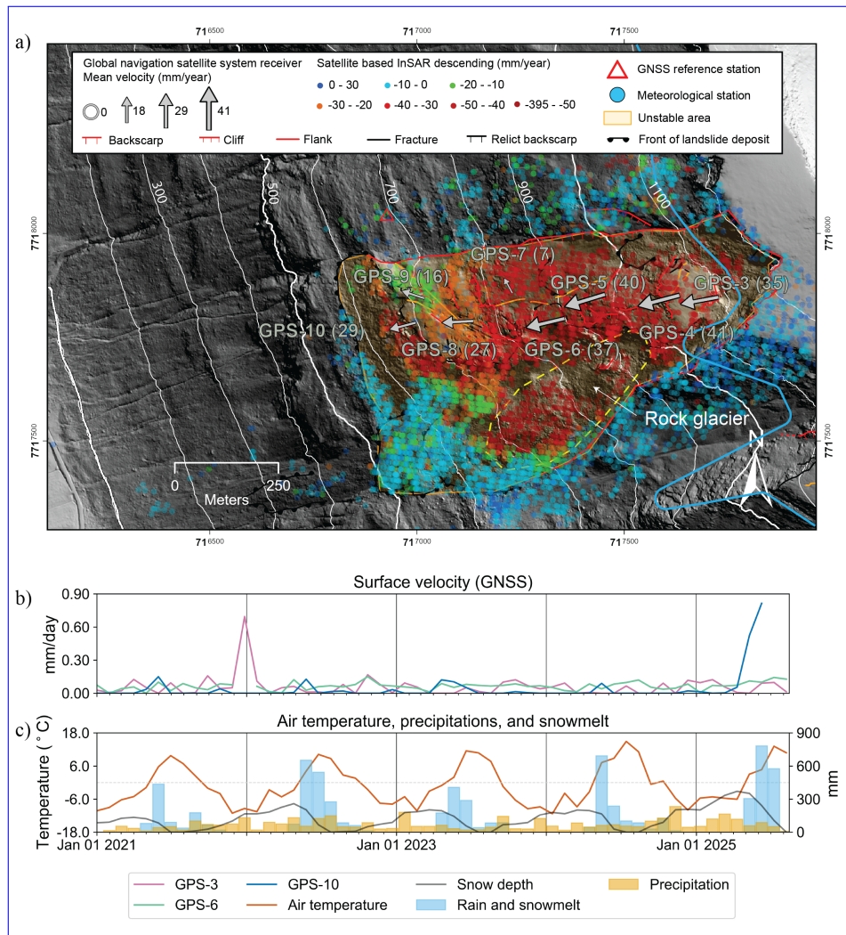
Figure 3. Map-Overview of the Gámanjunni landslide. a) Map illustrating key morphological features and instrument locations. Gray arrows denote mean GNSS-derived surface velocities (mm/yr) calculated for the period from 01.01.2021 to 12.08.2025, with arrow size scaled to velocity magnitude and annotated values in parentheses. The blue solid line indicates the elevation above which permafrost is highly probable (Etzelmüller et al., 2022). The yellow dashed outline delineates the active rock glacier extent. Elevation contours are shown in white at 100-meter intervals Hillshade based on Høydedata (Kartverket) . Accompanying plots display b) GNSS velocity and c) meteorological time series over the past five years. The GNSS velocity is calculated by a linear regression over one day and smoothed using-by down-sampling to 30-day median for GNSS-intervals, while the rainfall, snowmelt, and total precipitation is down-sampled to 30-day cumulative sums-for-rainfall and snowmelt-intervals.
