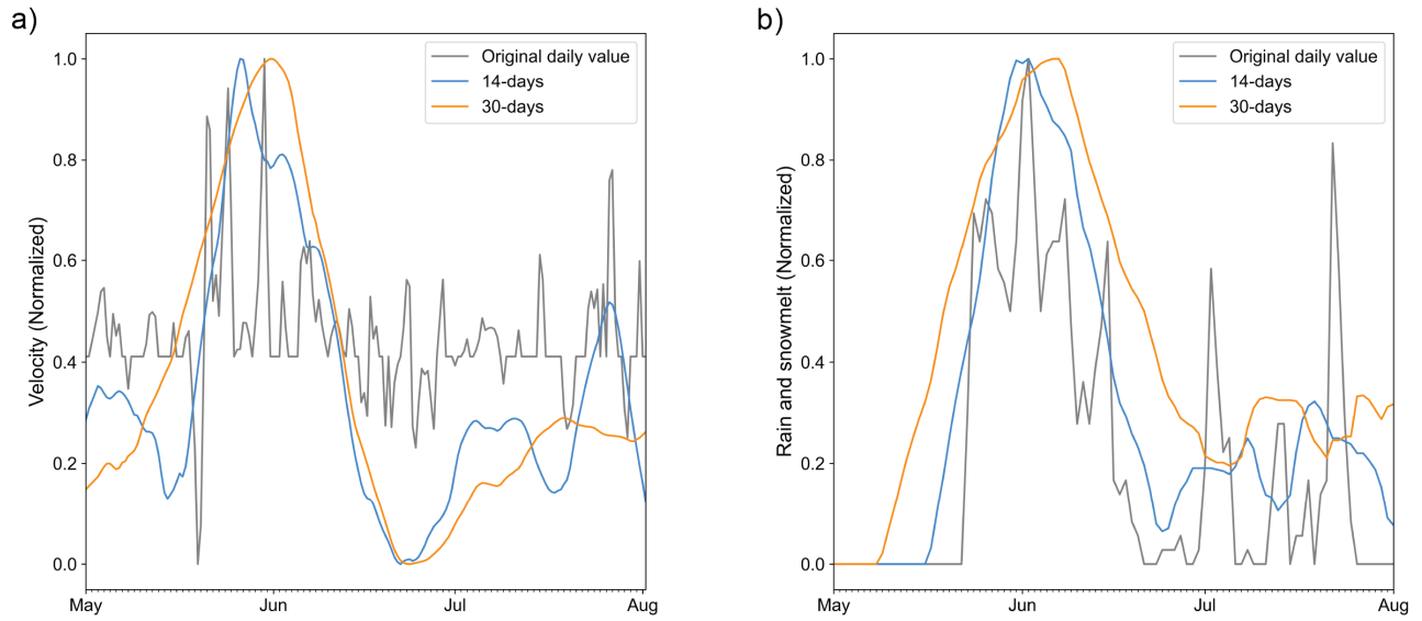
Figure A1. Verification of zero lag created by the window lengths by the rolling functions. a) Normalized velocity from GPS-4 on Jettan with 1-day, 14-days, and 30-days velocity calculated by the centered rolling linear regression function (see Section Integration of Data). b) Normalized rain and snowmelt summed over 1-day, 14-days, and 30-days by the centered running sum function.
