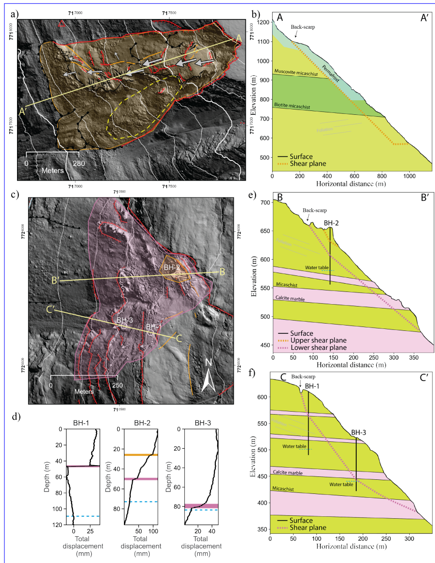
Figure 5. Schematic representation of the Gámanjuni and Jettan landslides based on identified shear zones detected in the boreholes. The two profiles a) Map of Gámanjuni with profile A-A' and c) Map of Jettan with profiles B-B' and their C-C' , and associated associated boreholes (BH-1 to BH-3) are shown on the map. The displacement in the three b, e, and f) Geologic cross-sections showing lithology, foliation, interpreted shear zones, permafrost extent, boreholes indicates the presence of, and hydraulic head. d) Borehole displacement data indicating one or two distinct shear zones . The scale of the axes differs between each plot. The displacement is measured Displacements are shown in the slip direction and represents the maximum displacement recorded in each borehole values. The orange Axis scales differ among plots . Orange and pink lines represent denote the interpreted upper and lower shear zone locations , and respectively, while the dashed blue line represents indicates the maximum water level hydraulic head . We interpreted the shear Shear zones by plotting the boreholes on the profiles were inferred from borehole observations and extrapolating the shear zones to mapped morphological structures/features . Proposed sliding scenarios are represented spatially on the map with transparent Semi-transparent orange and pink polygons indicate the proposed sliding scenarios .
