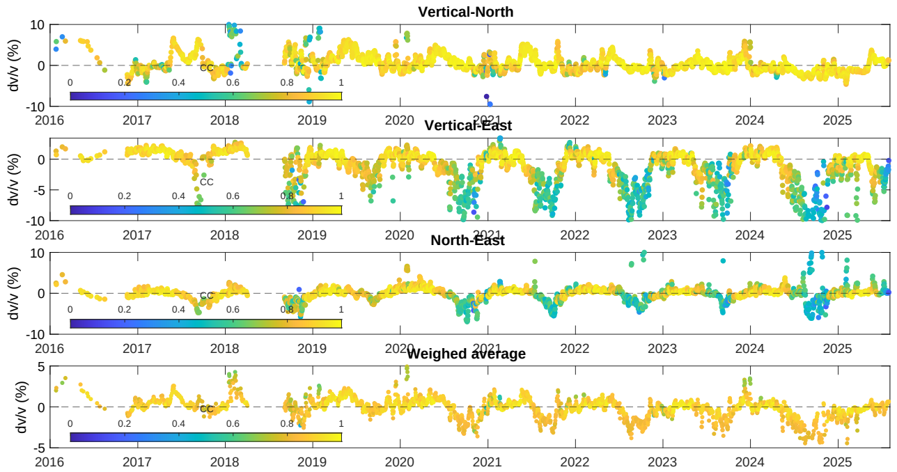
Figure A11. Time series of dv/v at seismic station JETT on Jettan landslide . The first three graphs show individual time series for the three possible pairs of components Vertical-North (Z-N), Vertical-East (Z-E) and North-East (N-E). The graph at the bottom shows the average dv/v time series where each dv/v value is weighed by its coefficient of correlation.
