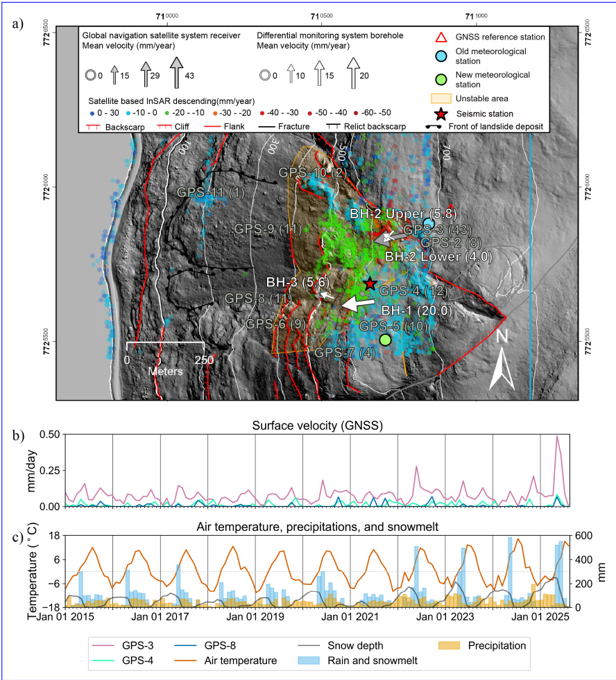
Figure 2. Map-Overview of the Jettan landslide. a) Map showing key morphological features and instrument locations (Credit: Kartverket). Gray arrows represent mean surface velocities (mm/yr) derived from GNSS data, while white arrows indicate borehole shear zone displacements from the differential monitoring system (BH), both averaged over the period from 01.01.2021 to 12.08.2025. Arrow dimensions are scaled proportionally to velocity magnitude, with values annotated in parentheses. Borehole BH-2 displays two arrows corresponding to distinct shear zones. The blue solid line indicates the elevation above which permafrost is highly probable (Magnin et al., 2019). White contour lines denote 100-meter elevation intervals. Hillshade based on Høydedata (Kartverket). Time series plots include GNSS-derived surface velocities display b) GNSS velocity and c) meteorological parameters-time series over the past decade, smoothed using . The GNSS velocity is calculated by a linear regression over one day and smoothed by down-sampling to 30-day median for GNSS intervals, while the rainfall, snowmelt, and total precipitation is down-sampled to 30-day cumulative sums for rainfall and snowmelt intervals.
