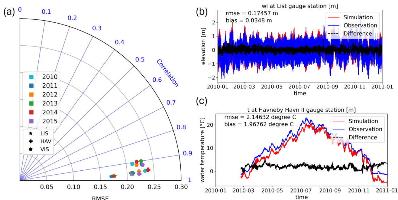
635 Figure C1: Comparison of observed and simulated water level and temperature: (a) the plot of correlation and RMSE includes the different stations for each year, using hourly data. The time series on the right show (b) the observed and simulated water level at List gauge station for 2010 and their difference and (c) the observed and simulated water temperature at Havneby Havn gauge station for 2010 and their difference, as an example for all simulated years. From Mohr et al. (2025) Mohr et al. (2025) Mohr et al. (2025).
