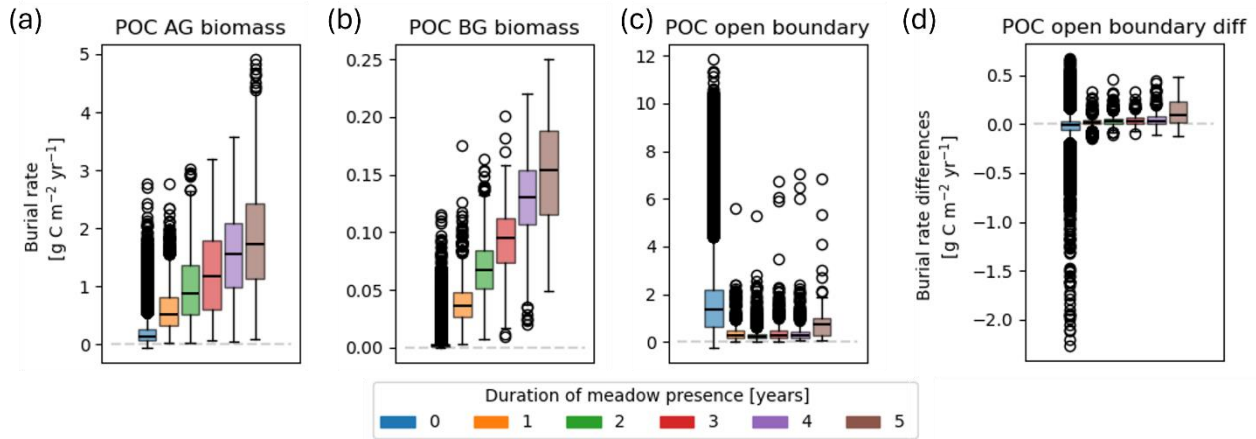
Figure 5: Boxplots of (a-c) mean -annual burial rates on tidal flats for different POC sources, averaged over five years of simulation time and -sorted by years with seagrass cover, and (d) difference in the mean -annual burial rates compared to simulations without seagrass, for allochthonous POC from the open boundary. The boxplots show the median and quartiles for the sequestration-burial rates on the model grid ; dots denote outliers from the spread.
