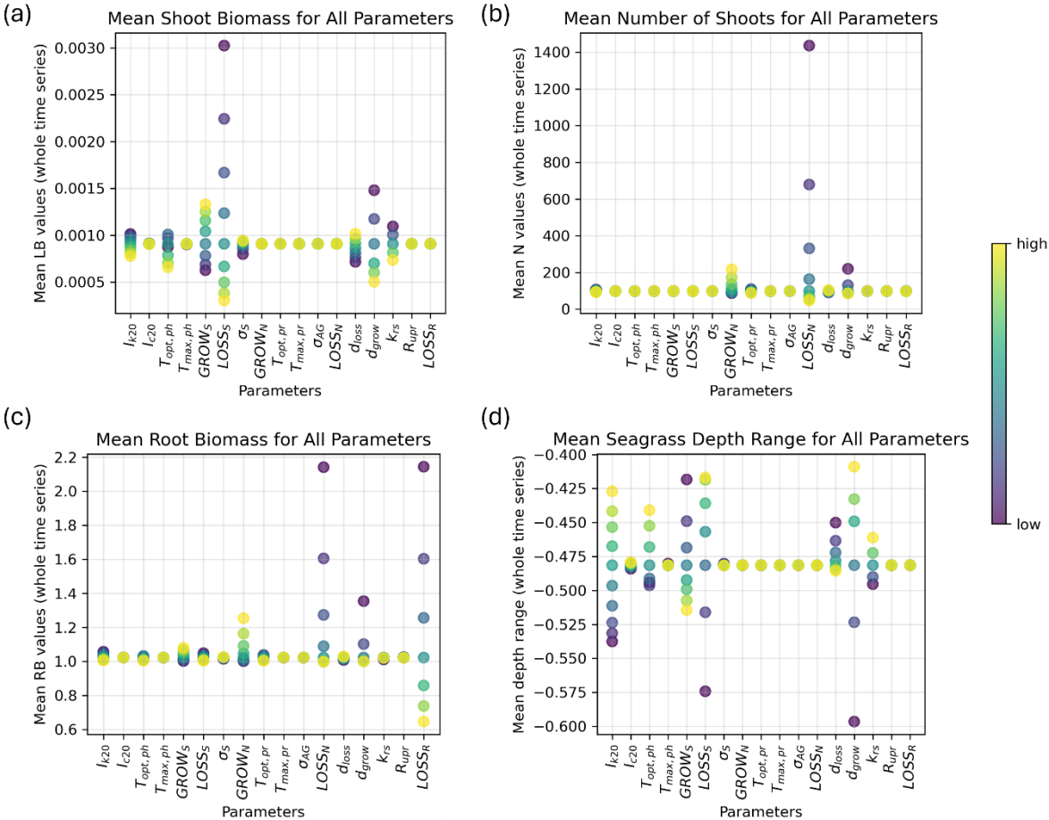
Figure A1: Impact of different parameter settings on seagrass growth, shown as the changes to mean (a) canopy height single shoot biomass, (b) number of shoots, (c) root biomass, and (d) mean depth of the distribution. Each parameter was changed over its scope defined in Table A1 while the other parameters were kept constant. For comparison purposes, the parameter values are marked high to low instead of the actual values. The range for each parameter is listed in Table A1. Growth of seagrass in the model is driven by weekly averaged values of temperature, solar radiation, mean inundation time, and wind speed, which are calculated based on the simulation results of the hydrodynamic model. The weekly averaged temperature represents the mean value for both water temperature when the seagrass meadow is inundated and air temperature otherwise:
