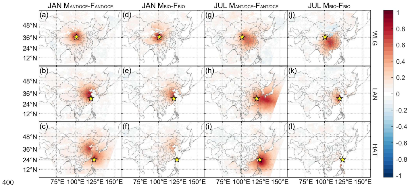
Figure 4. Spatial patterns of the tracer-flux correlations in different cases. Each row represents a site, labeled at right. (a)–(c) M_{ANT} - F_{ANT} and M_{OCE} - F_{OCE} in January; (d)–(f) M_{BIO} - F_{BIO} in January; (g)–(l) July.
