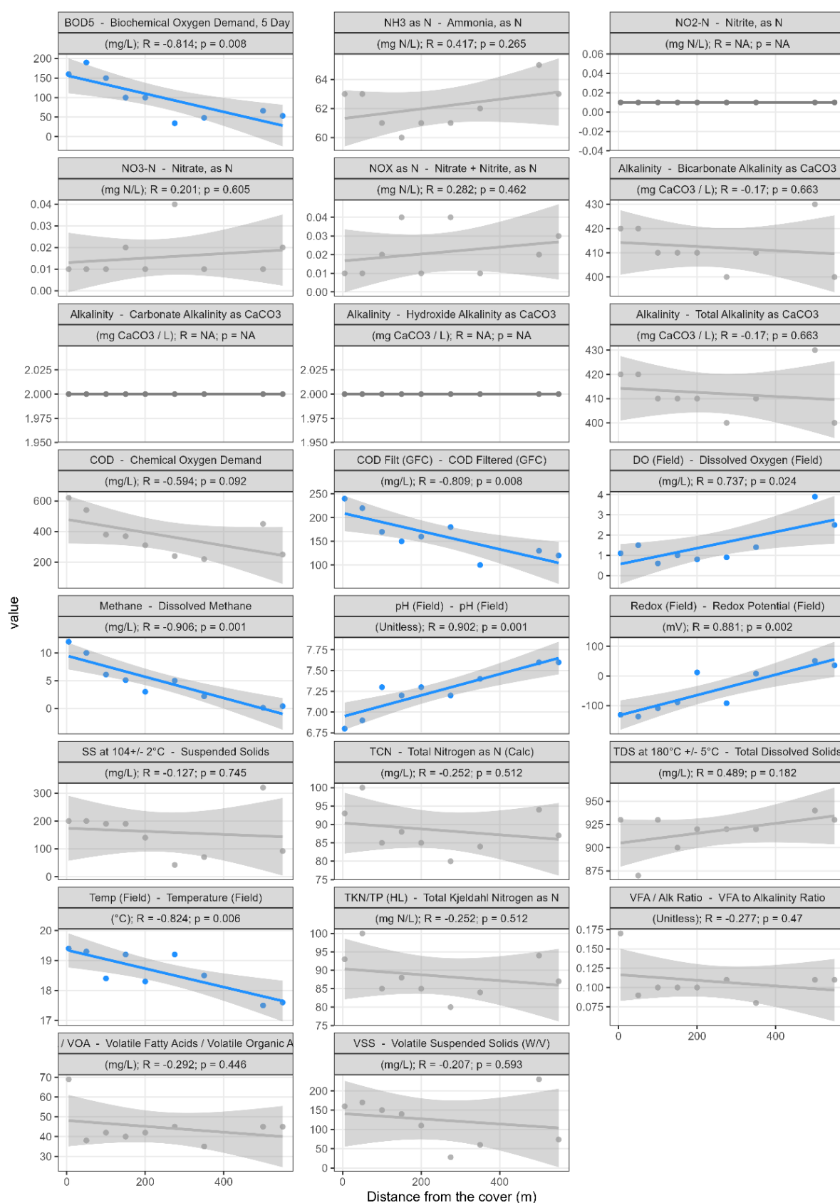
582 Figure 4. Correlations between wastewater sample contents including dissolved methane, BOD, COD, SS, VSS, 583 N-NH 3 , TCN, VFA, pH, and dissolved oxygen and the distance from the anaerobic cover. Samples were collected
