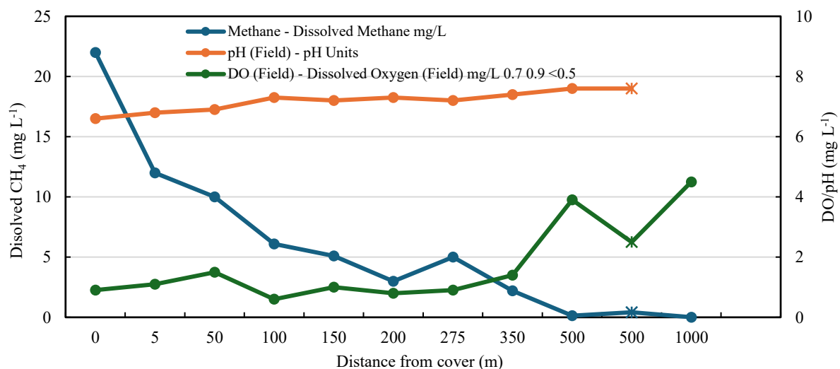
Figure 3. Variations of dissolved methane, BOD, COD, SS, VSS, NH 3 , TCN, VFA, pH, and dissolved oxygen shown with increasing distance from the cover area. Wastewater samples were collected by drone along the middle part of Pond 1 between 10:00–12:30 on the 10 September 2024 at 5, 50, 100, 150, 200, 275, 350, and 500 m from the cover, and extra samples were also collected at the PotCod, the jetty area (marked with an “ж”) and Pond 1 outlet (0, 500, and 1000 m from the cover, respectively) on the same day.
