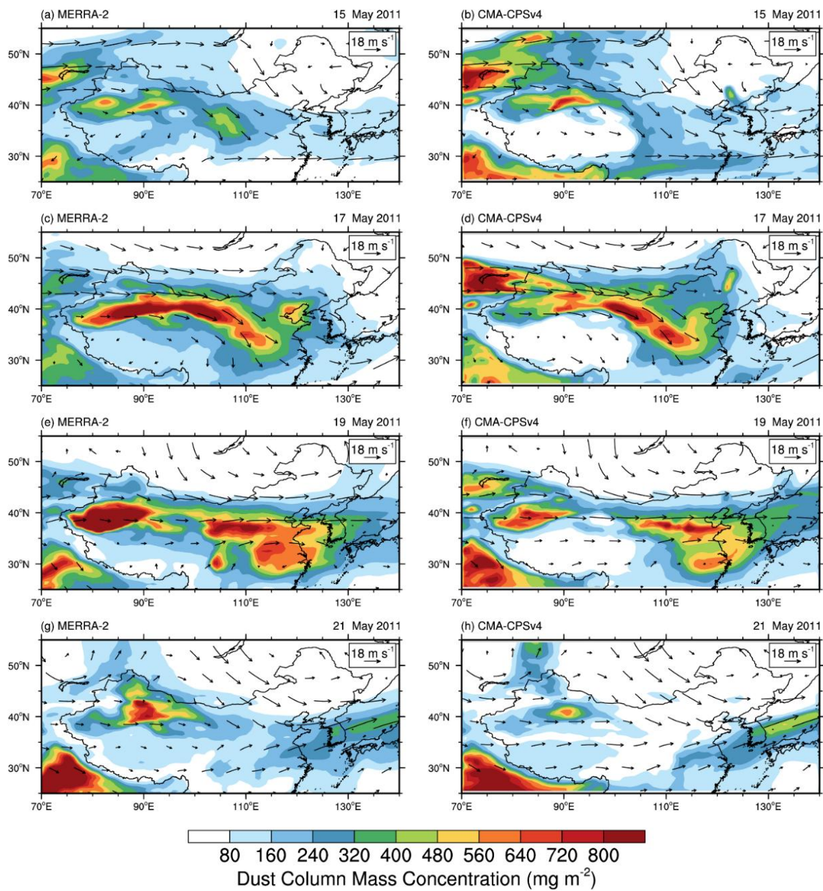
Figure 12.14. Spatial distribution of dust column mass concentrations (units: \text{mg m}^{-2} ) overlaid with 500 hPa wind vectors (units: \text{m s}^{-1} ) in China for the dust event from May 15 to 21, 2011, derived from MERRA-2 (left column) and CMA-CPSv4 (right column).
