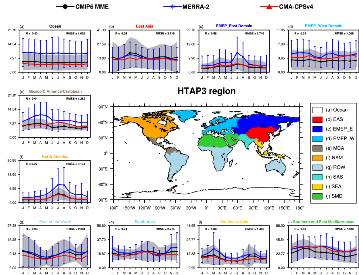
Figure 4. The monthly variations of surface \text{PM}_{2.5} concentrations (units: \mu\text{g m}^{-3} ) from MERRA-2 (blue line), CMIP6 MME (black line) and CMA-CPSv4 (red line) across for different world regions over of the world during 2001–2020 period. The gray shading and blue error bars show the regional variability in the values of the multi-model ensemble mean and MERRA-2 across the region, respectively. The upper-left and upper-right corners of each panel show the correlation coefficient (R) and root mean square error (RMSE) between CMA-CPSv4 and CMIP6 MME. The middle panel shows the nine regions (EAS, EMEP_E, EMEP_W, MCA, NAM, ROW, SAS, SEA, SMD) of the globe as defined by the Task Force on Hemispheric Transport of Air Pollutants (TF HTAP3), as well as the ocean.
