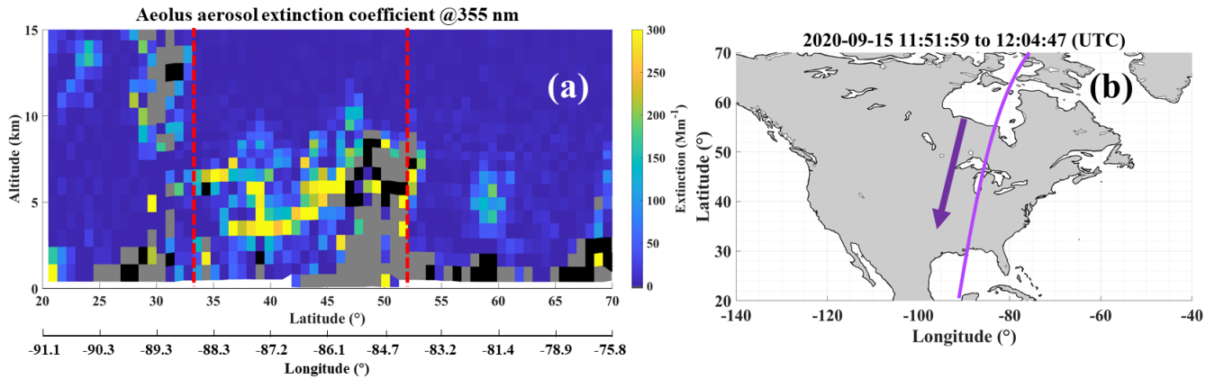
310 Figure 4. (a) One cross-section example of Aeolus aerosol extinction coefficient crossing the smoke plume, on 15 September 2020, starting at 11:51:59 (UTC) on 70.0°N, 75.8°W and ending at 12:04:47 (UTC) on 20.5°N, 91.1°W. (b) The corresponding descending orbit indicated by the purple curve (Aeolus orbit) and the purple arrow (Aeolus flight direction). The data in panel (a) has been processed to derive smoke data from Aeolus by the steps introduced in the section “Derivation of the smoke dataset from ALADIN observations”. The black bins indicate the invalid values, while the grey ones indicate the cloud contaminated bins. The profiles 315 inside two red dashed lines are the “smoke profiles”.
