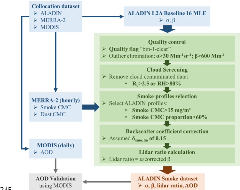
Figure 3. Methodology flowchart for development and validation of the Aeolus-based smoke dataset. \alpha and \beta represent ALADIN observed extinction and backscatter coefficients. R_b and RH represent backscattering ratio and relative humidity. CMC is column mass concentration and \delta_{smo, lin} is smoke linear depolarization ratio.
