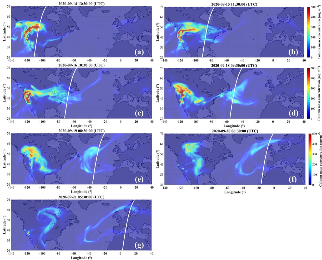
Figure 6. Smoke column mass concentration map in the spatial range of 140°W to 40°E, 20°N to 70°N, on (a) 14, (b) 15, (c) 16, (d) 18, (e) 19, (f) 20, (g) 21 September 2020, respectively. The white curves indicate the selected Aeolus orbits on the same days.
