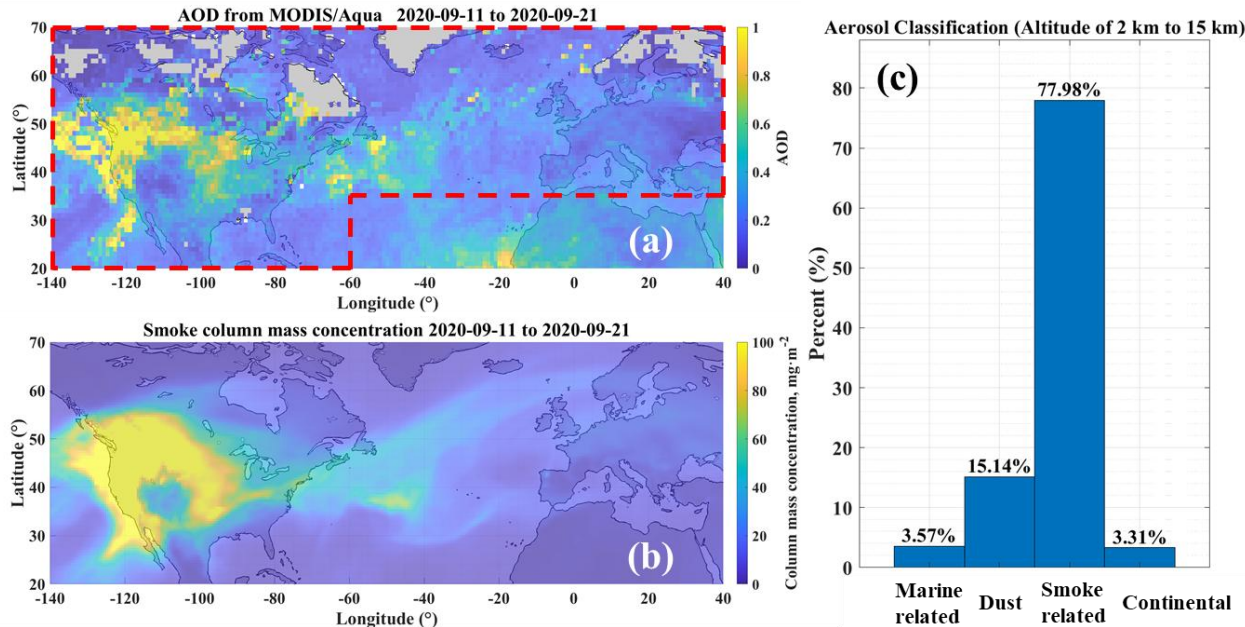
210 Figure 2. (a) Average AOD by MODIS onboard Aqua; (b) Average smoke column mass concentration (CMC) by MERRA-2; (c) Statistical result of aerosol classification from CALIOP VFM products, taking the data in the region indicated by the red dashed box of panel (a). The temporal range is 11 to 21 September 2020. In panel (c), “Marine related” indicates “marine” and “dusty marine” from CALIOP VFM products, and “Smoke related” includes “elevated smoke”, “polluted continental/smoke”, “polluted dust”.
