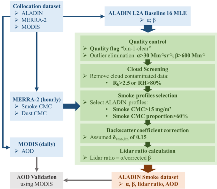
Figure 3. Methodology flowchart for development and validation of the Aeolus-based smoke dataset. \alpha and \beta represent ALADIN observed extinction and backscatter coefficients. R_b and RH represent backscattering ratio and relative humidity. CMC is column mass concentration and \delta_{\text{smo, lin}} is smoke linear depolarization ratio.
