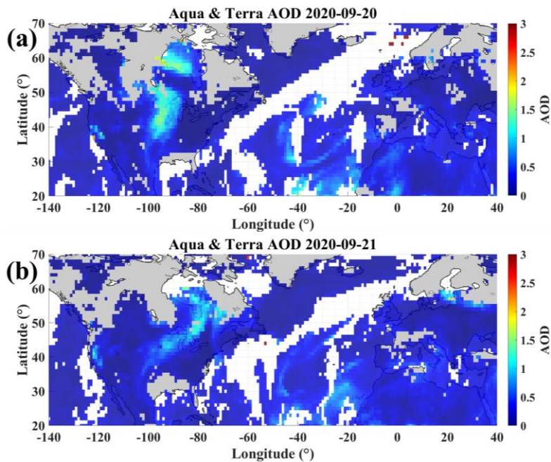
Figure A1. Average AOD from both Aqua and Terra on (a) 20 and (b) 21 September 2020.
