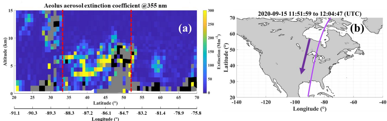
Figure 4. (a) One cross-section example of Aeolus aerosol extinction coefficient crossing the smoke plume, on 15 September 2020, starting at 11:51:59 (UTC) on 70.0°N, 75.8°W and ending at 12:04:47 (UTC) on 20.5°N, 91.1°W. (b) The corresponding descending orbit indicated by the purple curve (Aeolus orbit) and the purple arrow (Aeolus flight direction). The data in panel (a) has been processed to derive smoke data from Aeolus by the steps introduced in the section “Derivation of the smoke dataset from ALADIN observations”. The black bins indicate the invalid values, while the grey ones indicate the cloud contaminated bins. The profiles inside two red dashed lines are the “smoke profiles”.
