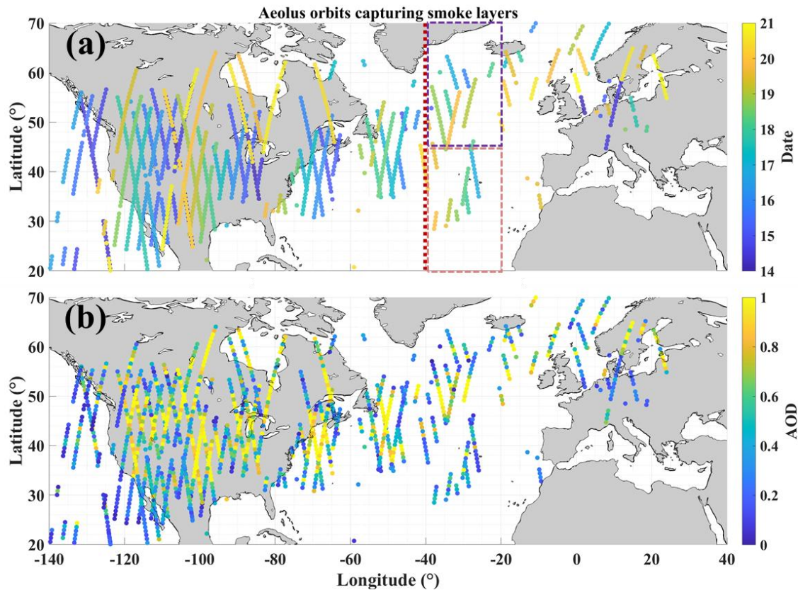
Figure 9. Smoke layers captured by ALADIN along the Aeolus orbits, with the color of the tracks representing (a) observational time and (b) AOD. In panel (a), the red dotted line divides the layers at earlier and later transport stage, while the purple and pink dotted boxes highlight the layers of the northern and southern branches following the plume separation.
