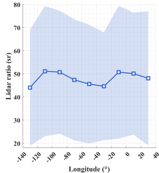
Figure 12. Statistical results (means and standard deviations) of smoke lidar ratio along longitude. The statistics were calculated by using the Aeolus smoke dataset (within the altitude range of 2 km to 12 km) in the period of 14 to 21 September 2020, in the smoke plume transport region of 140°W to 40°E and 20°N to 70N, and with the longitude grid of 20°.
