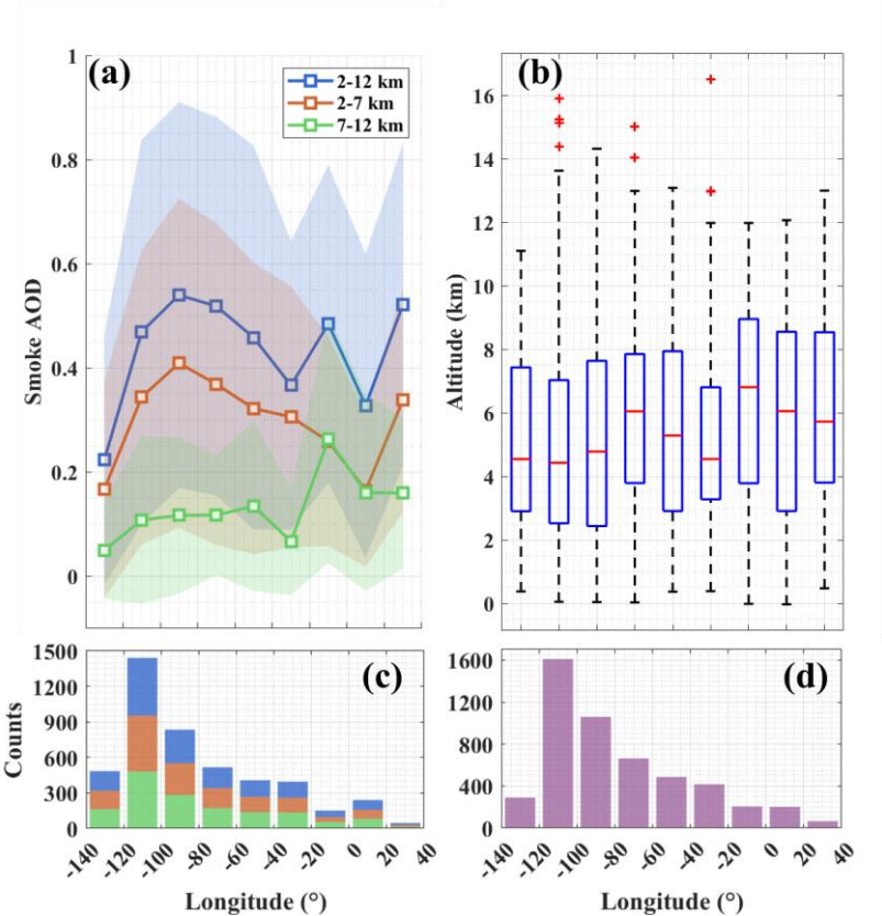
565 Figure 10. Statistical results (a) smoke AOD (means and standard deviations), (b) smoke bins altitude (boxplot) along longitude. (c)(d) The corresponding data counts of the statistics. The statistics were calculated using the Aeolus smoke dataset in the period of 14 to 21 September 2020, in the smoke plume transport region of 140°W to 40°E and 20°N to 70N, and with the longitude grid of 20°. Smoke AOD includes total AOD (2 km to 12 km), AOD within 2 to 7 km (AOD M ), and AOD within 7 to 12 km (AOD U ), indicated by the blue, red and green curves, respectively. In panel (c), the corresponding data counts are also presented by the stacked bars in the same color with the AOD curves.
