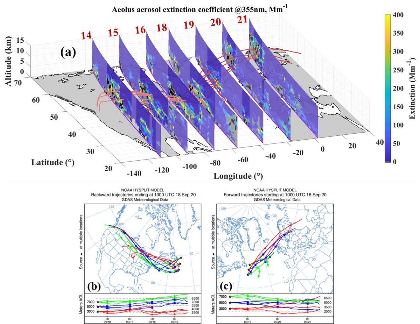
420 Figure 7. (a) The selected cross-sections of Aeolus aerosol extinction coefficient at 355 nm on 14, 15, 16, 18, 19, 20, 21 September 2020, with the HYSPLIT trajectories starting from 18 September. In the cross-sections, the black and grey bins indicate invalid data and cloud contaminated data separately, while the pink curves present the backward trajectories and the red curves are the forward trajectories. The dark parts of the curtains indicate smoke profiles identified by the step (3) in Section 4.2. Details of the (b) backward and (c) forward trajectories originating from the middle of the transport pathway (acquired by https://www.ready.noaa.gov/HYSPLIT_traj.php , last access: 7 September 2025).
