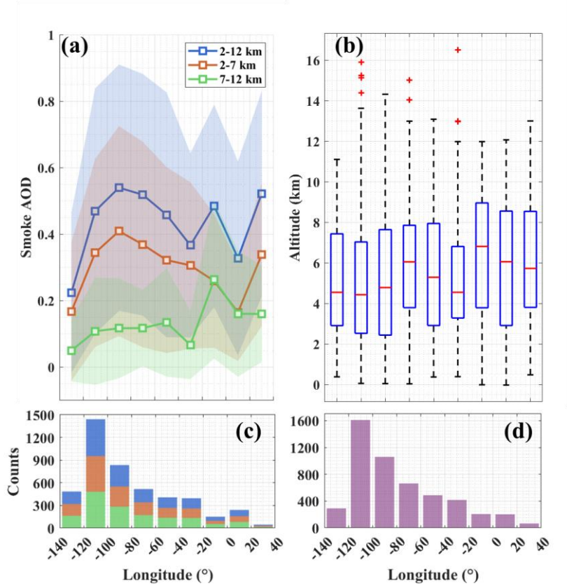
555 Figure 10. Statistical results (a) smoke AOD (means and standard deviations), (b) smoke bins altitude (boxplot) along longitude. (c)(d) The corresponding data counts of the statistics. The statistics were calculated using the Aeolus smoke dataset in the period of 14 to 21 September 2020, in the smoke plume transport region of 140°W to 40°E and 20°N to 70N, and with the longitude grid of 20°. Smoke AOD includes total AOD (2 km to 12 km), AOD within 2 to 7 km ( AOD_M ), and AOD within 7 to 12 km ( AOD_U ), indicated by the blue, red and green curves, respectively. In panel (c), the corresponding data counts are also presented by the stacked bars in the same color with the AOD curves.
