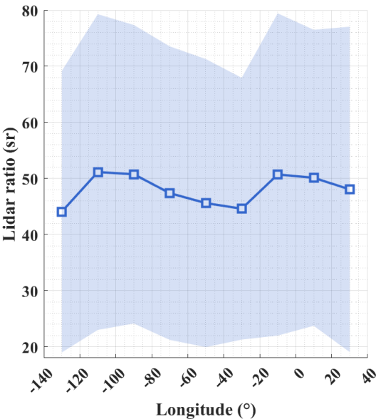
625 Figure 12. Statistical results (means and standard deviations) of smoke lidar ratio along longitude. The statistics were calculated by using the Aeolus smoke dataset (within the altitude range of 2 km to 12 km) in the period of 14 to 21 September 2020, in the smoke plume transport region of 140°W to 40°E and 20°N to 70N, and with the longitude grid of 20°.
