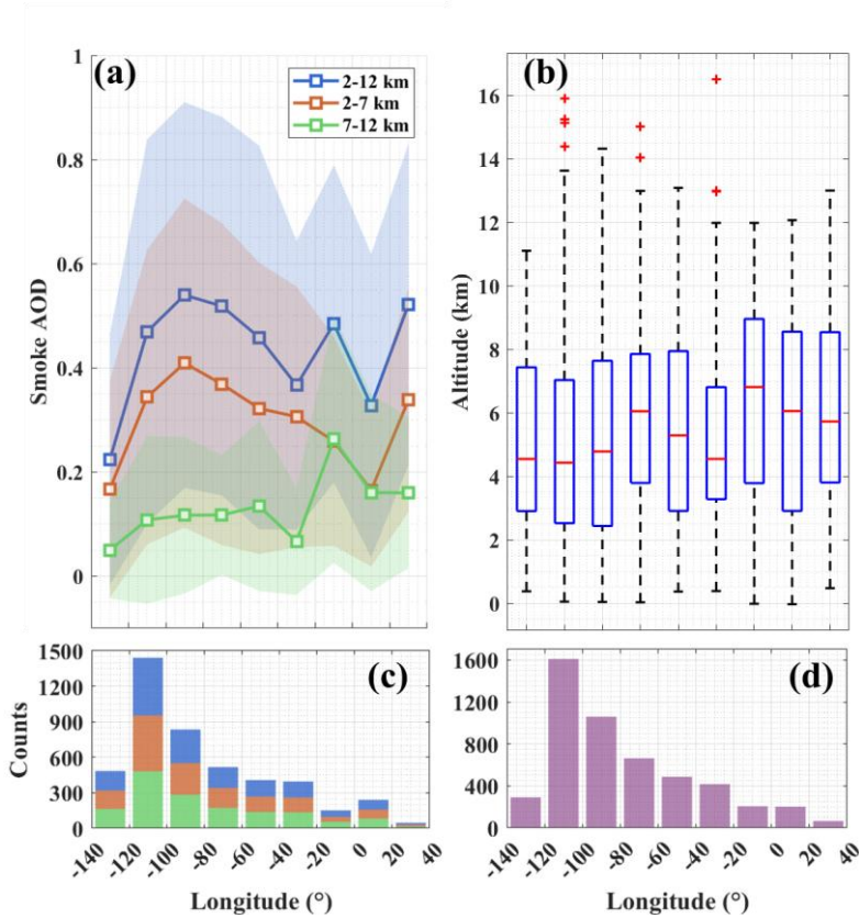
Figure 10. Statistical results (a) smoke AOD (means and standard deviations), (b) smoke bins altitude (boxplot) along longitude. (c)(d) The corresponding data counts of the statistics. The statistics were calculated using the Aeolus smoke dataset in the period of 14 to 21 September 2020, in the smoke plume transport region of 140°W to 40°E and 20°N to 70N, and with the longitude grid of 20°. Smoke AOD includes total AOD (2 km to 12 km), AOD within 2 to 7 km ( AOD_M ), and AOD within 7 to 12 km ( AOD_U ), indicated by the blue, red and green curves, respectively. In panel (c), the corresponding data counts are also presented by the stacked bars in the same color with the AOD curves.
