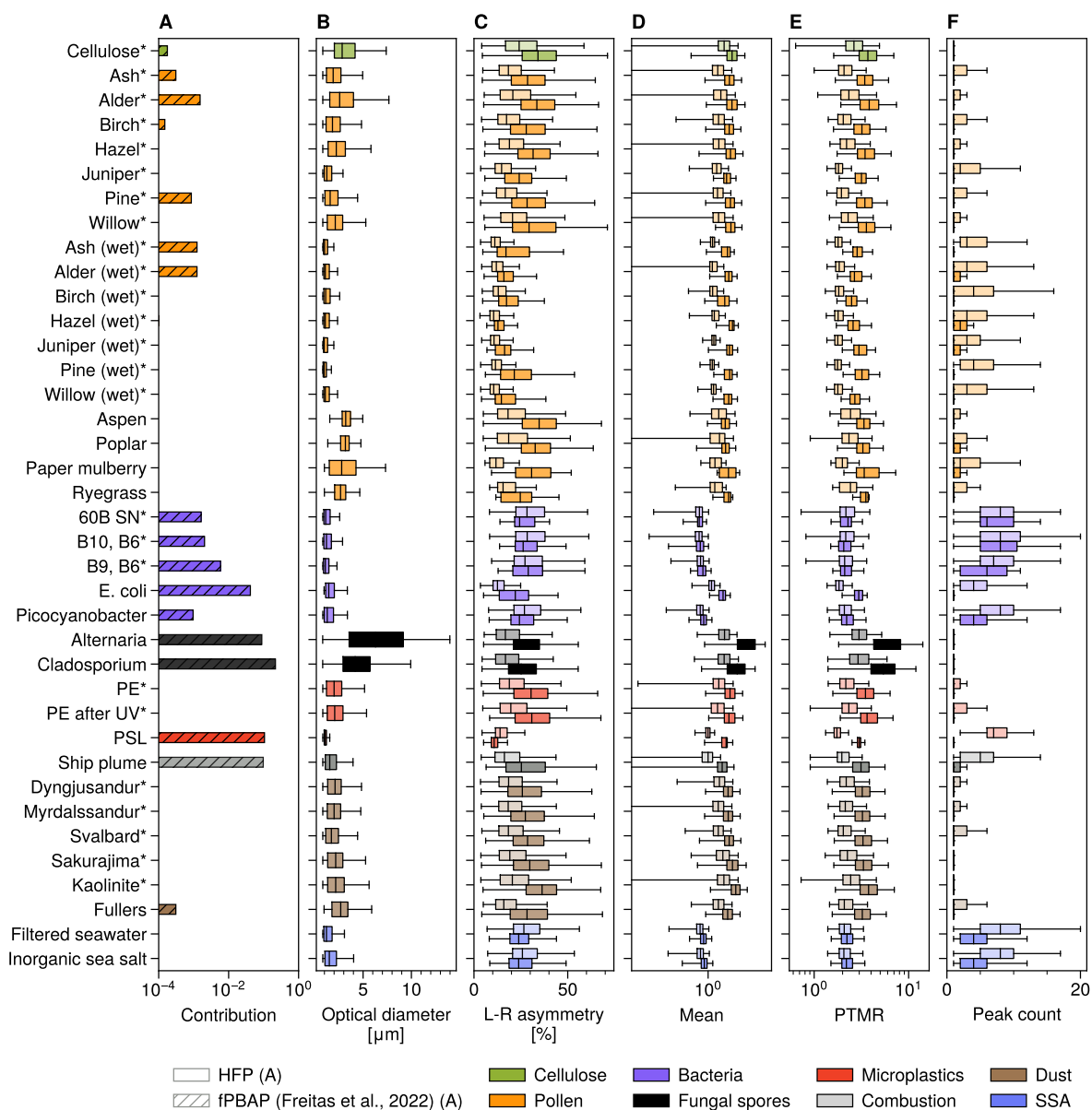
Figure 4. Comparison of particle property distributions for all source data. (a): Contributions to total particles measured in the samples by highly fluorescent particles (HFPs, solid bars ) and fluorescent primary biological aerosol particles (fPBAPs, hatched bars ) as identified by the decision tree method of Freitas et al. (2022). For the ship plume, only HFPs are displayed. (b-f): Size (b) and morphology parameters (c-f) of particles in the samples. In (c-f), dark (light) boxes indicate < (\geq) 3 \mu\text{m} particles. The right array is shown for single-array morphology parameters (d-f). The color denotes the source group the sample belongs to (see legend).
