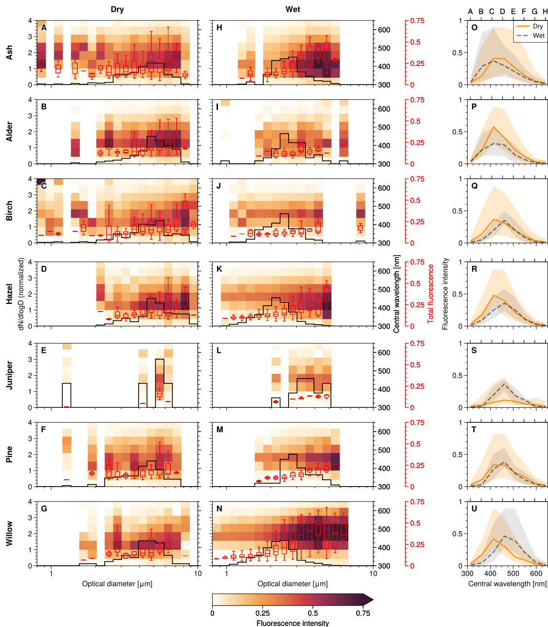
Figure 1. Pollen - Pollen-derived particle fluorescence properties and size distributions measured in our characterization experiments. Size distributions (left axis, black step trace) and fluorescence emission spectra (right axis, color map) for highly fluorescent particles (HFPs) with > 9\sigma fluorescence signal, binned by size, in (a-g) dry and (h-n) wet pollen characterization experiments. Box plots (red axes) depict the range of total fluorescence in each size bin. Fluorescence intensities are given as a fraction of detector maxima at saturation. (o-u): The median fluorescence emission spectra of HFPs in dry (solid) and wet (dashed) pollen experiments at all sizes; shaded areas represent 10-90% quantile ranges. Upper axes show fluorescence detection channel names corresponding to their central detection wavelengths in the lower axes.
