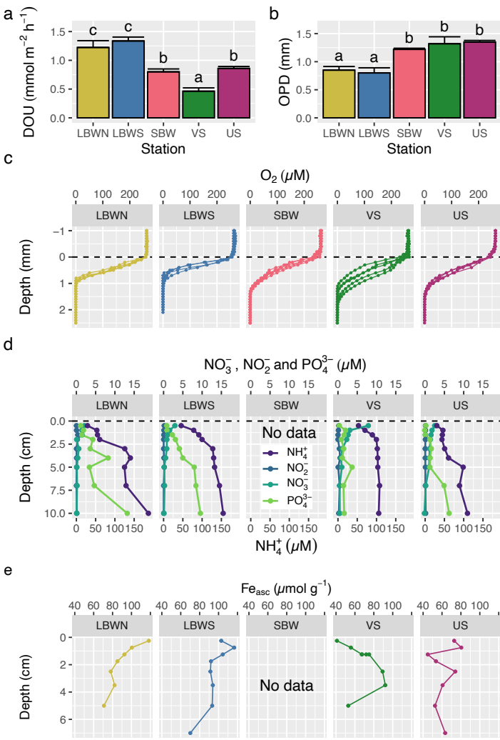
Figure 2: Porewater solute concentrations. (a) Diffusive O 2 uptake (DOU) by the sediment and (b) O 2 penetration depth (OPD). (c) O 2 concentration microprofile. (d) porewater \text{NO}_3^- , \text{NO}_2^- , \text{NH}_4^+ and \text{PO}_4^{3-} concentrations at each site (n = 1 with 5 pseudo replicates for DOU and OPD). (e) Solid-phase iron oxyhydroxide concentration at each site. Different letters indicate significant (p < 0.05, Tuckey contrast) differences among the different levels of Site (a and b)
