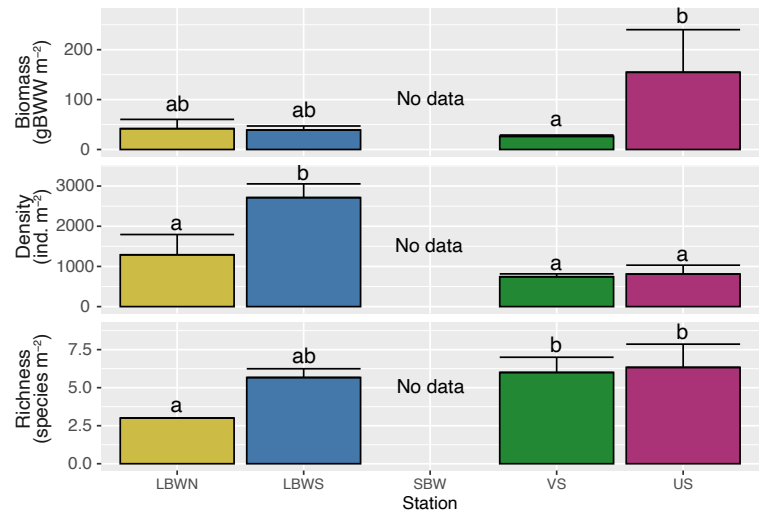
Figure 3: Univariate descriptors of macrofauna communities. Total biomass, density and species richness at the sampled sites (n = 3 per site). Different letters indicate significant (p < 0.05, Tuckey contrast) differences among the different levels of Site .
