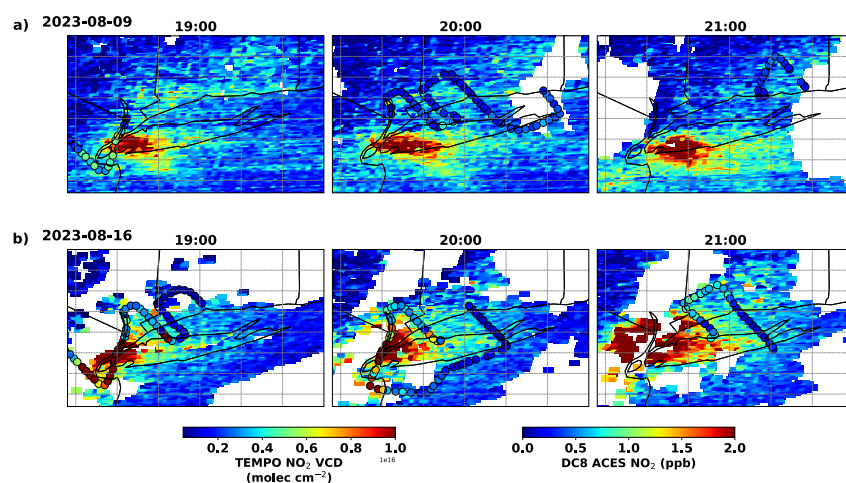
300 Figure 4: Hourly average TEMPO NO 2 VCDs (molec/cm 2 ) overlaid with hourly ACES measured NO 2 (ppb) for the two DC-8 flight days: August 9 and 16, 2023.
