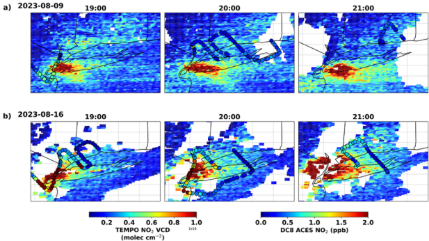
Figure 4: Hourly average TEMPO NO 2 VCDs (molec/cm 2 ) overlaid with hourly ACES measured NO 2 (ppb) for the two DC-8 flight days: August 9 and 16, 2023.
