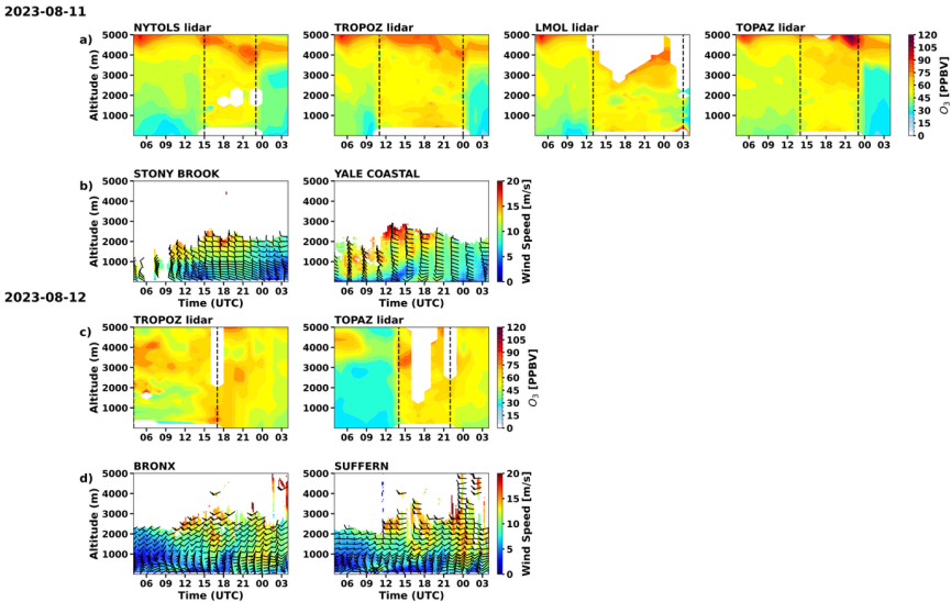
Figure 9: TOLNet lidar multidimensional O 3 (ppb) observations (outlined in black dotted lines) with WRF-Chem model simulated spatiotemporal O 3 filling missing data (a, c) and Doppler lidar (b, d) multidimensional wind profiles (m s -1 ) observations at sites around NYC/LIS on August 11 and 12, 2023.
