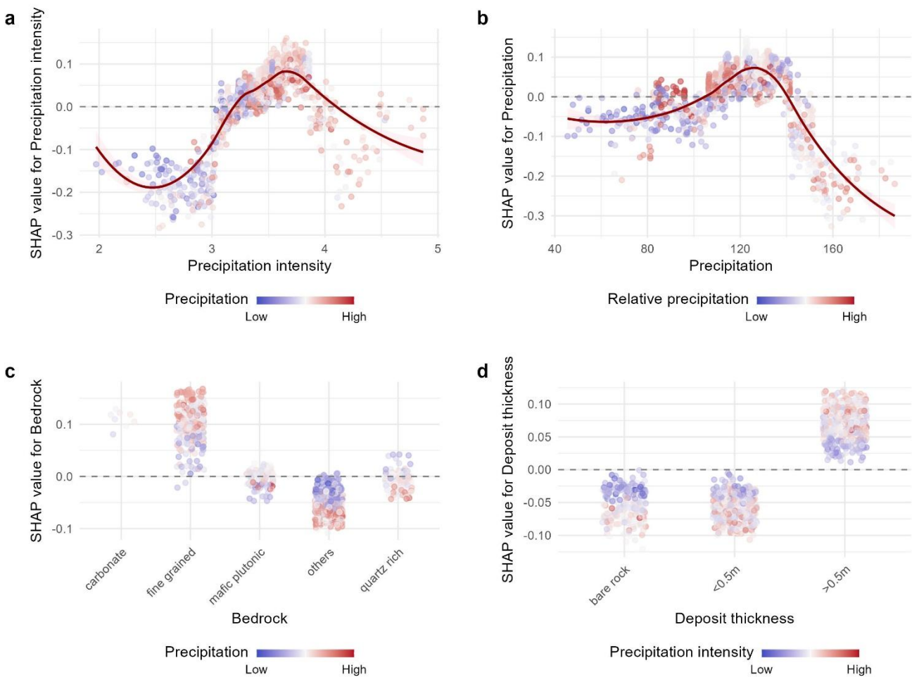
1025 Figure E1 a-d Partial dependence plots for the top four variables of full model 2a (non-spatial model with spatially clustered CV). Precipitation intensity in (a) is square root transformed. Each point represents an observation and is plotted with its feature value on the x-axis and SHAP value (contribution to model output) on the y-axis. SHAP values above 0 indicate that a feature value is likely to make a positive contribution to the probability of a landslide. Points are coloured by a second feature chosen to minimise the variance of the SHAP value given both features and represents the strongest interaction. Solid red lines are LOESS smoothed lines and shading represents 95% confidence intervals. 1030
