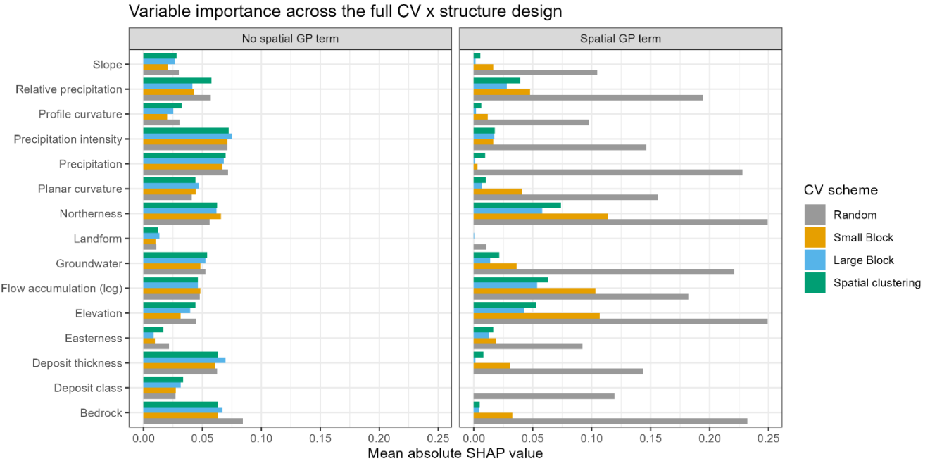
Figure 4 Full factorial comparison of variable importance scores for the full dataset, comparing non-spatial (No spatial GP term) with spatial (Spatial GP term) models built with all four cross-validation (CV) schemes. Variable importance was quantified using mean absolute SHAP (SHapley Additive exPlanations) values.
