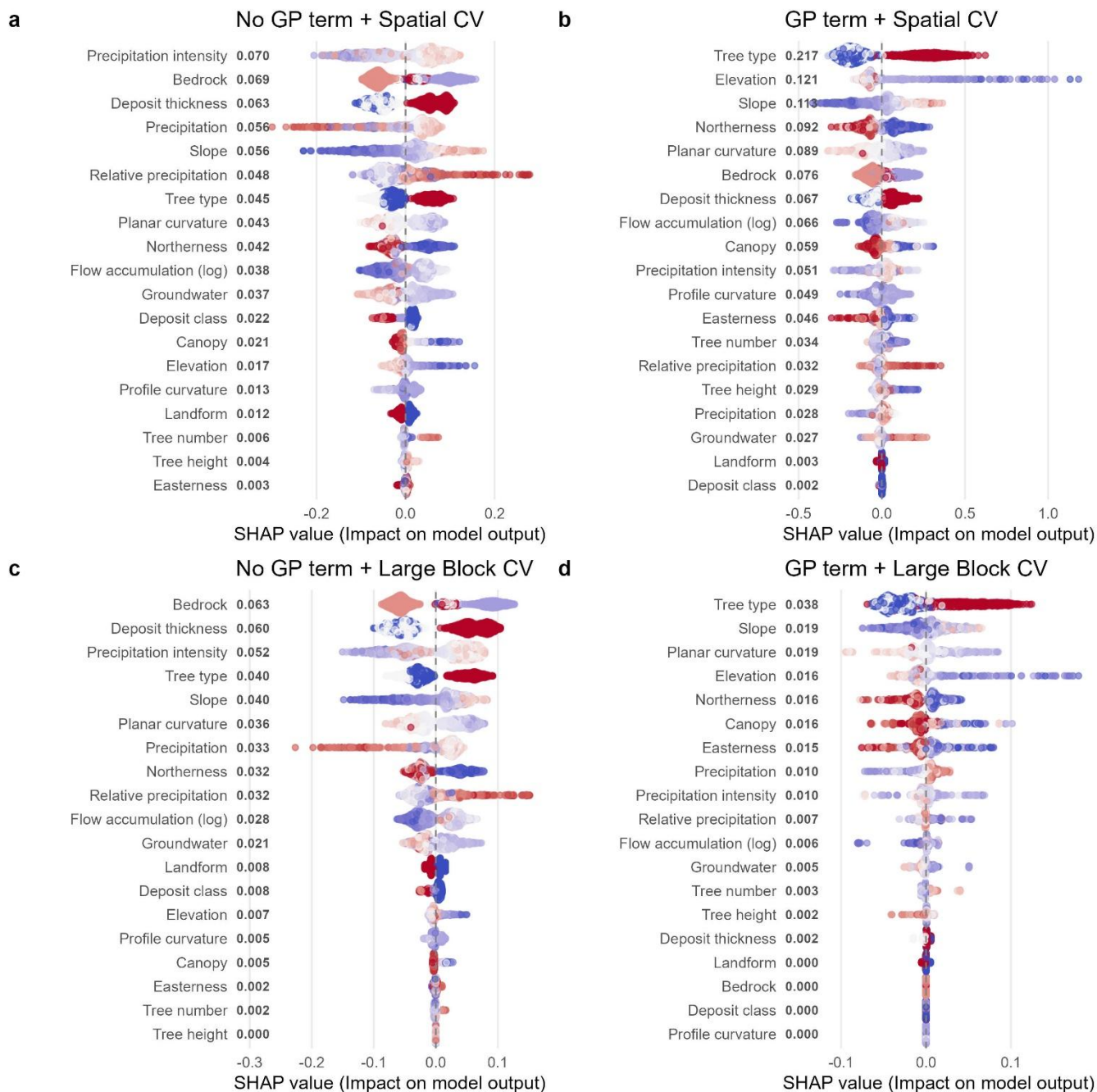
Figure E6 Shapley value summary plots for models on the forest-only dataset: a) spatially clustered CV without a spatial term (model 4a), b) spatially clustered CV with a spatial term (model 3a), c) large block CV without a spatial term (model 4b) and d) large block CV with a spatial term (model 3b) The numbers after variable names are mean absolute SHAP values, representing relative importance. Points are coloured by normalised feature value.
