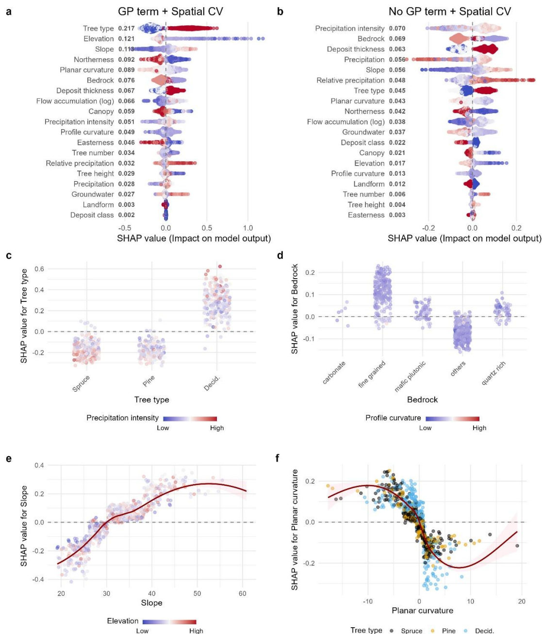
Figure 7 a)-b) Shapley value summary plots for forest-only model 3a (spatial model with spatially clustered CV) and model 4a (non-spatial model with spatially clustered CV). Note the dynamic SHAP value ranges on the x-axes. The numbers after variable names are mean absolute SHAP values, representing relative importance. Points are coloured by normalised feature value. c)-f) Partial dependence plots for four important variables of model 3a. Each point represents an observation and is plotted with its feature value on the x-axis and SHAP value (contribution to model output) on the y-axis. SHAP values above 0 indicate that a feature value is likely to make a positive contribution to the probability of a landslide. Points are coloured by a second feature chosen to minimise the variance of the SHAP value given both features and represents the strongest interaction. Solid red lines are LOESS smoothed lines and shading represents 95% confidence intervals.
