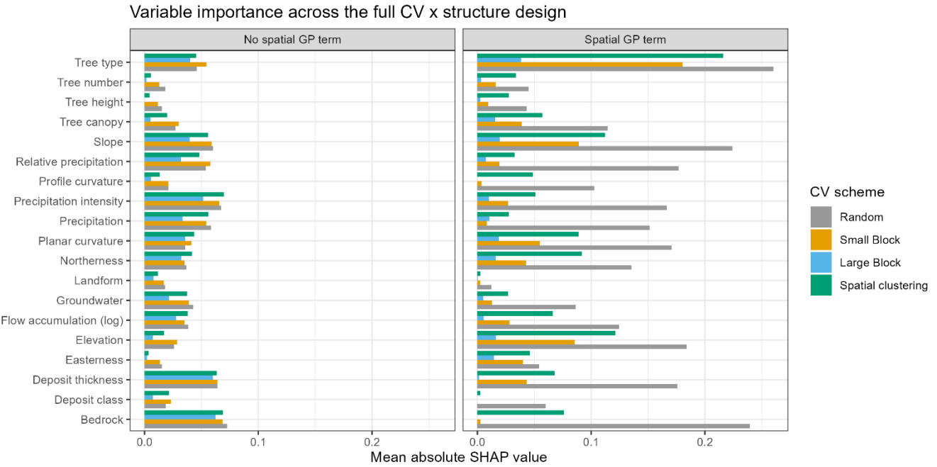
Figure 6 Full factorial comparison of variable importance scores for the forest dataset, comparing non-spatial (No spatial GP term) with spatial (Spatial GP term) models built with all four cross-validation (CV) schemes. Variable importance was quantified using mean absolute SHAP (SHapley Additive exPlanations) values.
