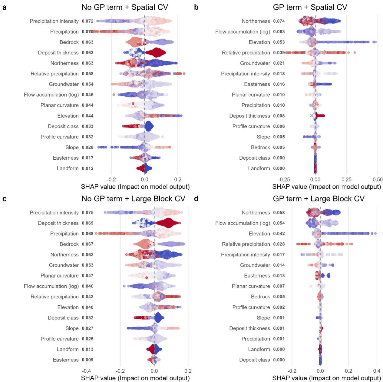
Figure E4 Shapley value summary plots for models on the full dataset a) spatially clustered CV without a spatial term (model 2a), b) spatially clustered CV with a spatial term (model 1a), c) large block CV without a spatial term (model 2b) and d) large block CV with a spatial term (model 1b) The numbers after variable names are mean absolute SHAP values, representing relative importance. Points are coloured by normalised feature value.
