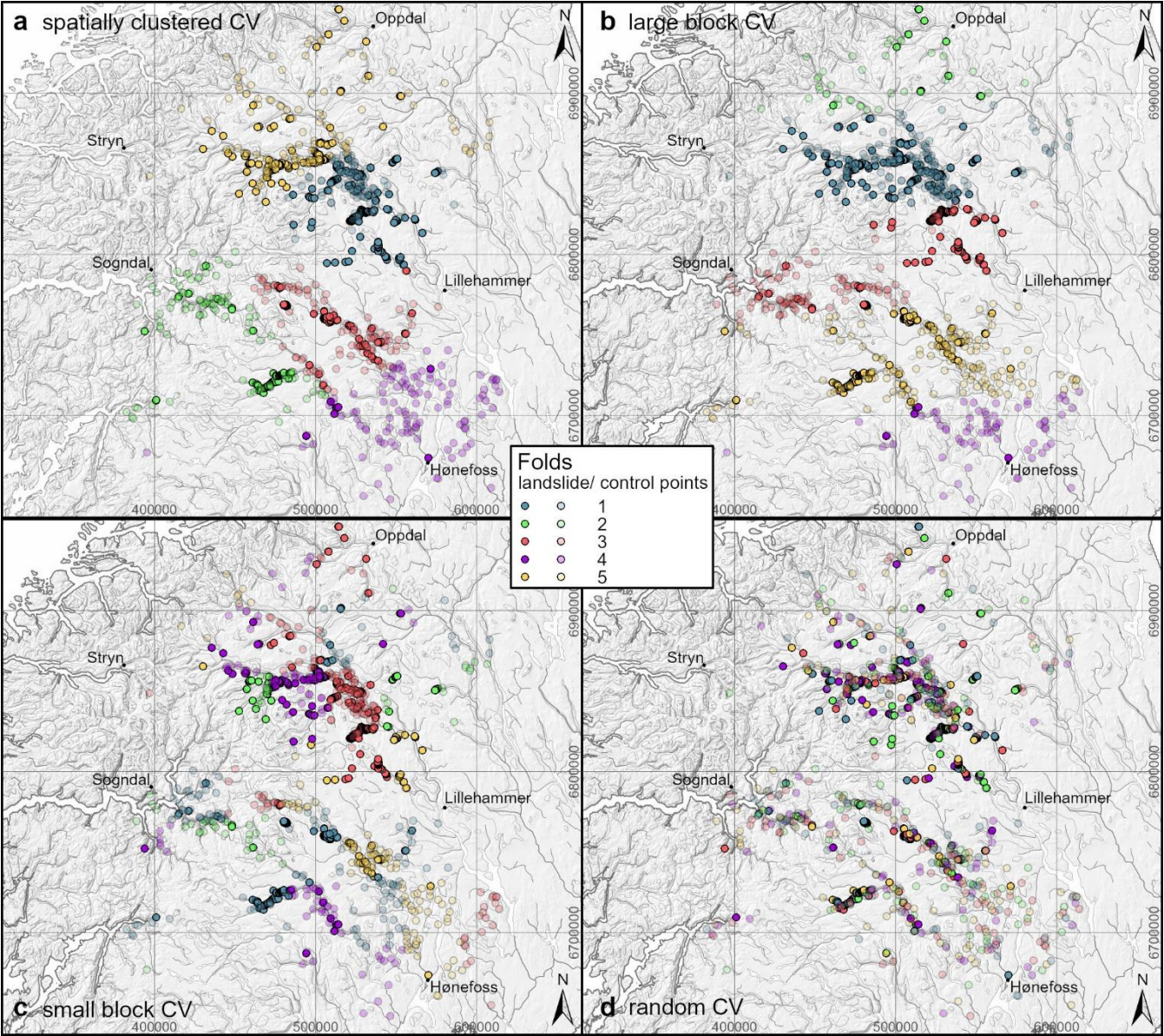
Figure C1 Spatial distribution of the folds assigned for the full models during a) spatially clustered cross-validation, b) large block cross-validation, c) small block cross-validation and d) random cross-validation.
