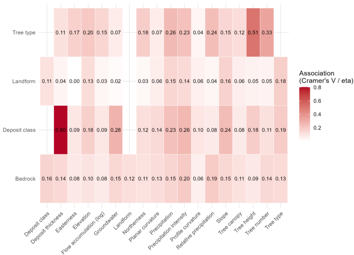
980 Figure D4 Heat map of associations between categorical variables and all other variables retained in the models using the forest dataset. Values between the categorical variables are Cramer's V, and values between categorical and continuous/ordinal variable pairs are correlation ratio ( \eta , derived from one-way ANOVA).
