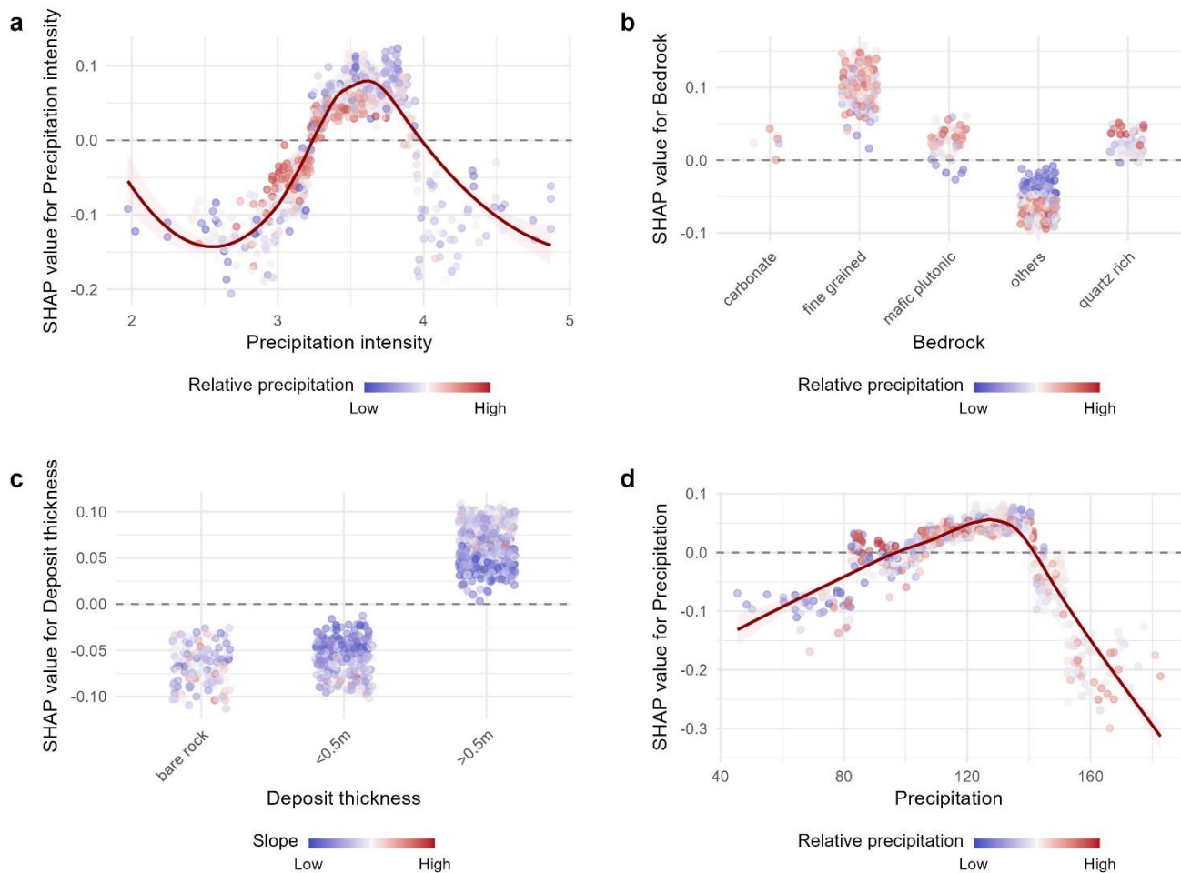
Figure E2 a-d Partial dependence plots for the top four variables of forest-only model 4a (non-spatial model with spatially clustered CV). Precipitation intensity in (a) is square root transformed. Each point represents an observation and is plotted with its feature value on the x-axis and SHAP value (contribution to model output) on the y-axis. SHAP values above 0 indicate that a feature value is likely to make a positive contribution to the probability of a landslide. Points are coloured by a second feature chosen to minimise the variance of the SHAP value given both features and represents the strongest interaction. Solid red lines are LOESS smoothed lines and shading represents 95% confidence intervals.
