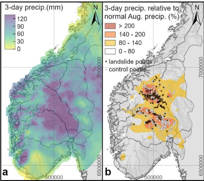
Figure 1 a) 3-day cumulative precipitation from 7 to 10 august, 2023 (6 UTC or 8 am local time) b) cumulative precipitation shown in (a) relative to normal precipitation for the entire month of August (for the standard normal period 1991-2020), and position of landslide and control points. Topographic map:    Kartverket, SeNorge.
