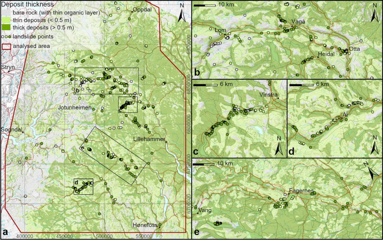
Figure 10 Spatial distribution of the categorical variable deposit thickness and shallow landslide starting points symbolised with corresponding colours for a) the entire study area, b) Ottadalen, c) Skåbudalen, d) inner Hallingdal and e) Valdres. © Kartverket, NGU.
