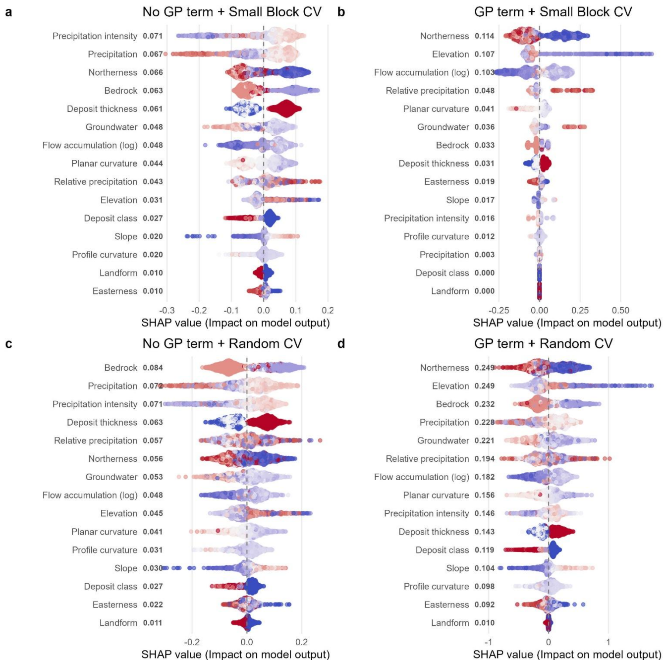
Figure E5 Shapley value summary plots for models on the full dataset: a) small block CV without a spatial term (model 2c), b) small block CV with a spatial term (model 1c), c) random CV without a spatial term (model 2d) and d) random CV with a spatial term (model 1d). The numbers after variable names are mean absolute SHAP values, representing relative importance. Points are coloured by normalised feature value.
