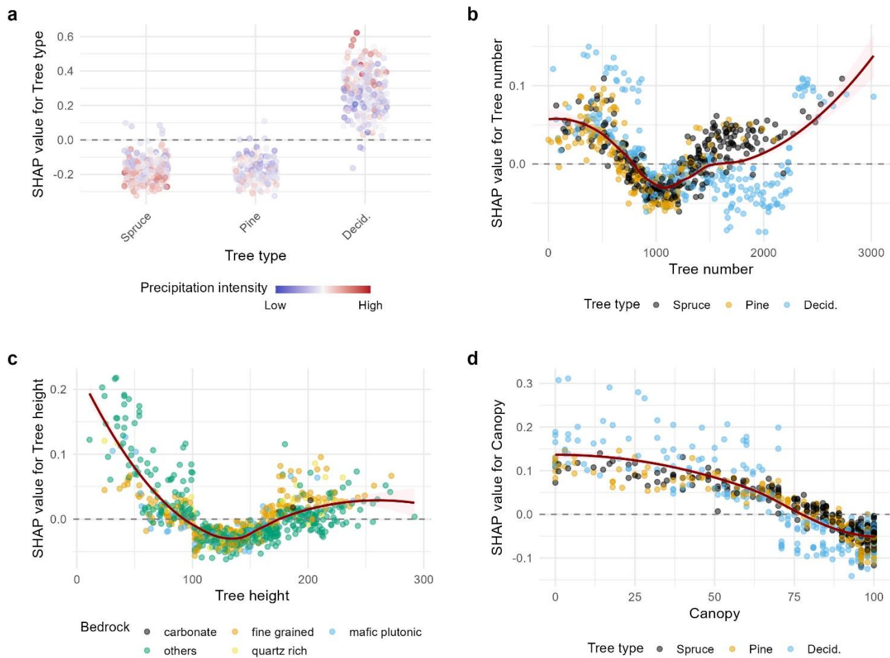
Figure E3 a-d Partial dependence plots for the four included forest variables of forest-only model 4a (non-spatial model with spatially clustered CV). Each point represents an observation and is plotted with its feature value on the x-axis and SHAP value (contribution to model output) on the y-axis. SHAP values above 0 indicate that a feature value is likely to make a positive contribution to the probability of a landslide. Points are coloured by a second feature chosen to minimise the variance of the SHAP value given both features and represents the strongest interaction. Solid red lines are LOESS smoothed lines and shading represents 95% confidence intervals.
