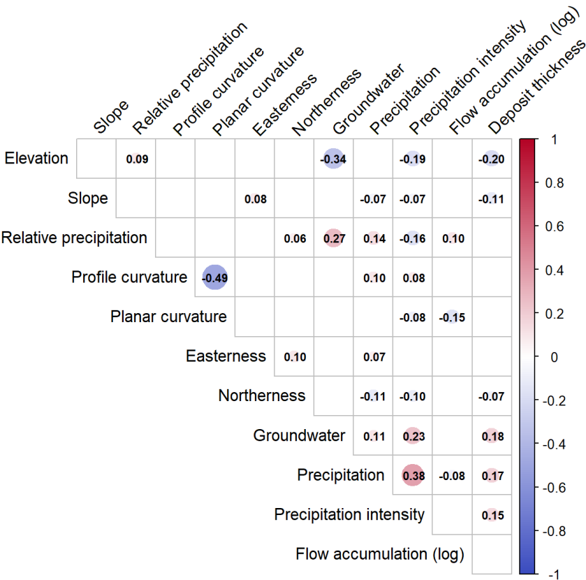
970 Figure D1 Spearman's rank correlation matrix for continuous and ordinal variables retained in the models for the full dataset. Correlations between -0.05 and 0.05 are not shown.
