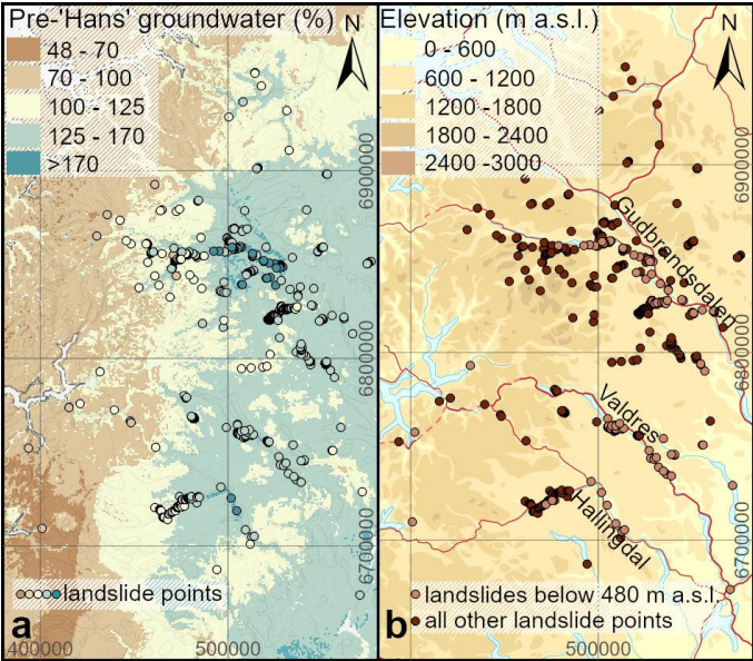
Figure 9 a) Modelled pre-‘Hans’ groundwater level compared to normal (1981-2010) for 7 August 2023, 8 am and shallow landslide starting points symbolised with colours corresponding to groundwater level. b) Shallow landslide starting points in the study area with those under 480 meters a.s.l. highlighted in lighter brown. © SeNorge, Kartverket. 650
