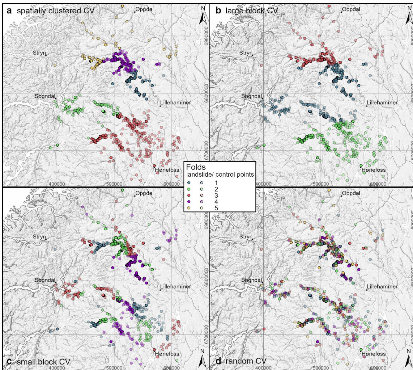
Figure C2 Spatial distribution of the folds assigned for the forest-only models during a) spatially clustered cross-validation, b) large block cross-validation, c) small block cross-validation and d) random cross-validation. Note that the number of folds had to be reduced to three for large block CV and four for small block CV to create folds which contained a relatively balanced number of both landslide and control points.
