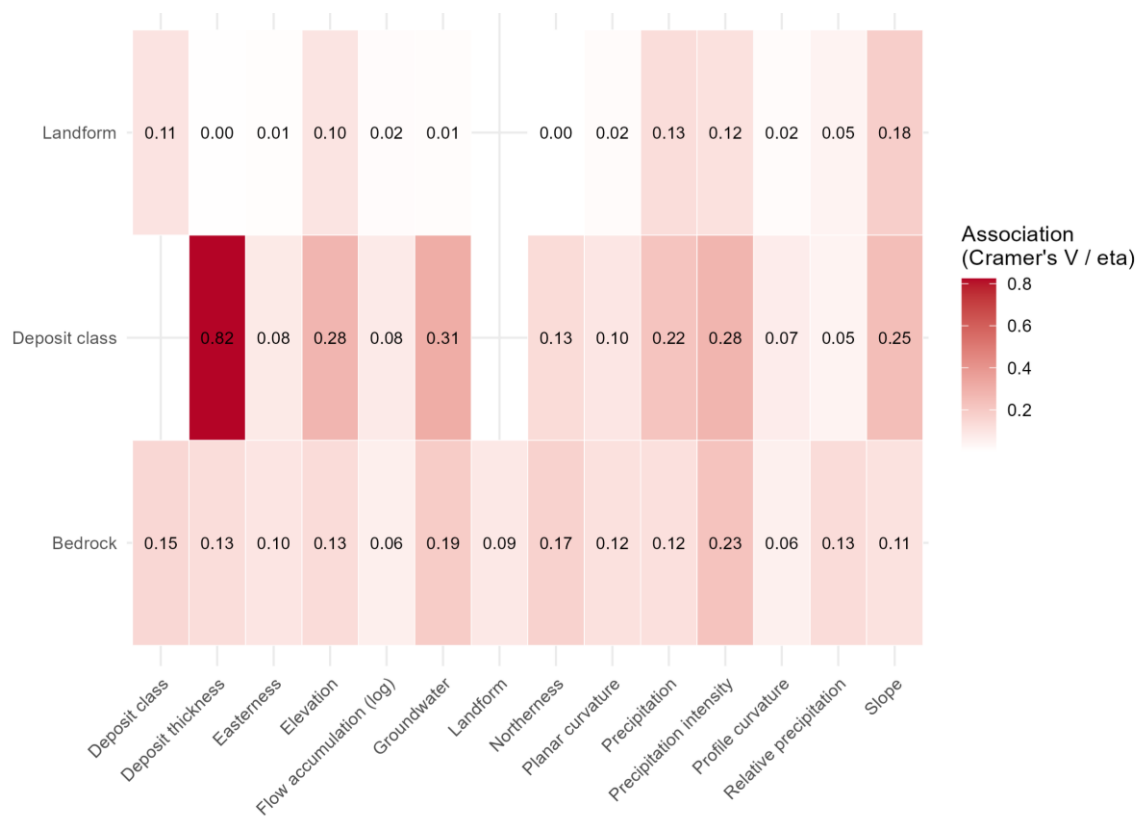
Figure D2 Heat map of associations between categorical variables and all other variables retained in the models using the full dataset. Values between the categorical variables are Cramer's V, and values between categorical and continuous/ordinal variable pairs are correlation ratio ( \eta , derived from one-way ANOVA).
