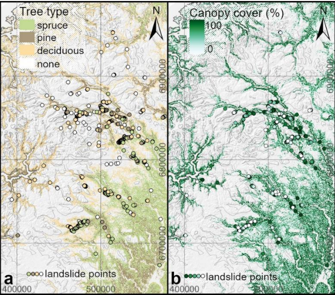
Figure 11 a) Tree type and shallow landslide starting points symbolised according to tree type. b) Canopy cover and shallow landslide starting points symbolised according to canopy cover. © Kartverket, NIBIO.
