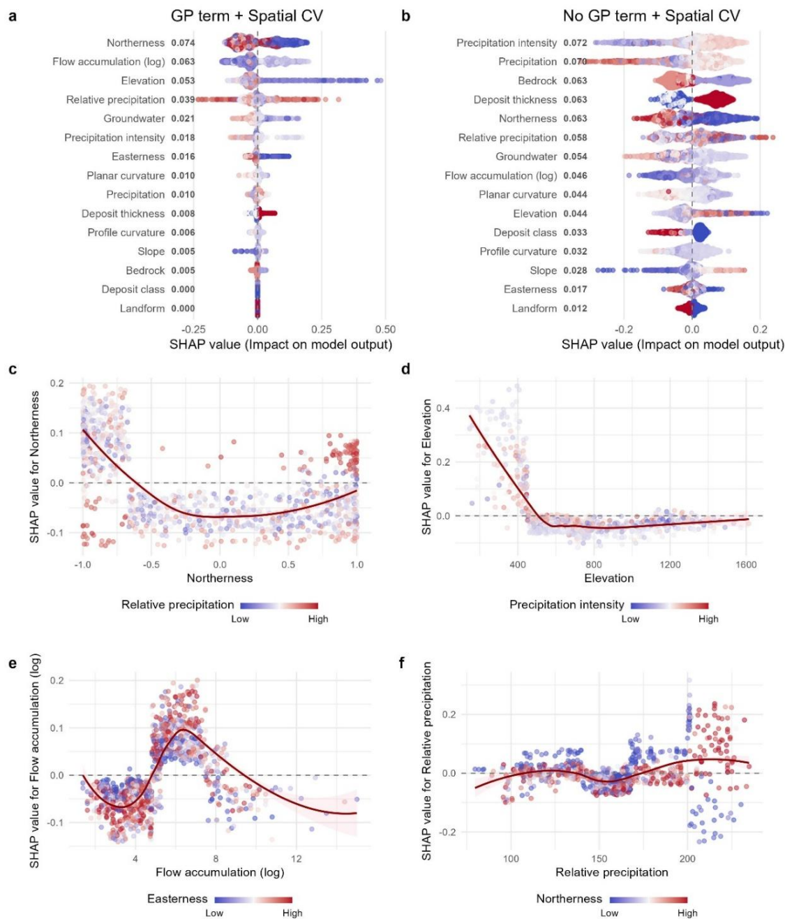
Figure 5 a)-b) Shapley value summary plots for model 1a (spatial model with spatially clustered CV) and model 2a (non-spatial model with spatially clustered CV). Note the dynamic SHAP value ranges on the x-axes. The numbers after variable names are mean absolute SHAP values, representing relative importance. Points are coloured by normalised feature value. c)-f) Partial dependence plots for the top four variables of model 1a. Each point represents an observation and is plotted with its feature value on the x-axis and SHAP value (contribution to model output) on the y-axis. SHAP values above 0 indicate that a feature value is likely to make a positive contribution to the probability of a landslide. Points are coloured by a second feature chosen to minimise the variance of the SHAP value given both features and represents the strongest interaction. Solid red lines are LOESS smoothed lines and shading represents 95% confidence intervals.
