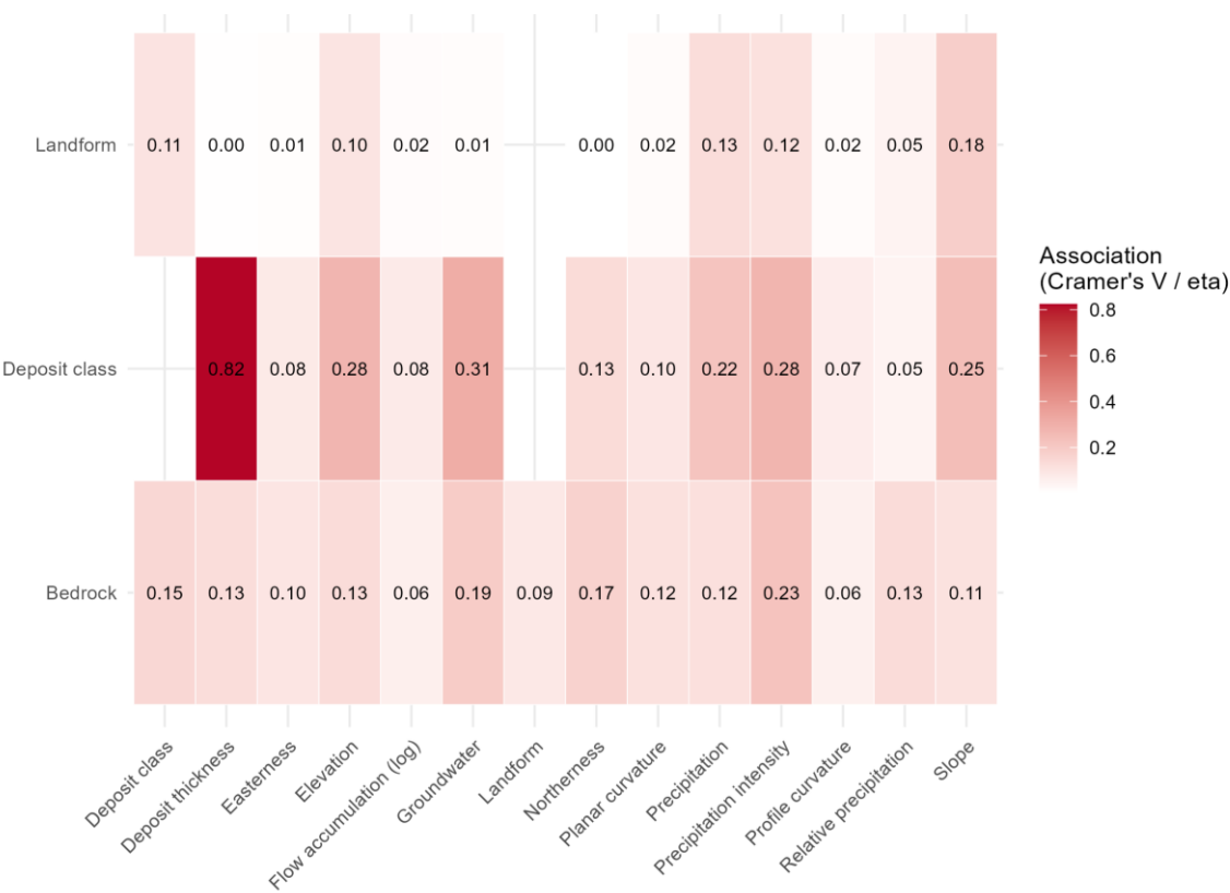
Figure D2 Heat map of associations between categorical variables and all other variables retained in the models using the full dataset. Values between the categorical variables are Cramer’s V, and values between categorical and continuous/ordinal variable pairs are correlation ratio ( \eta , derived from one-way ANOVA).
