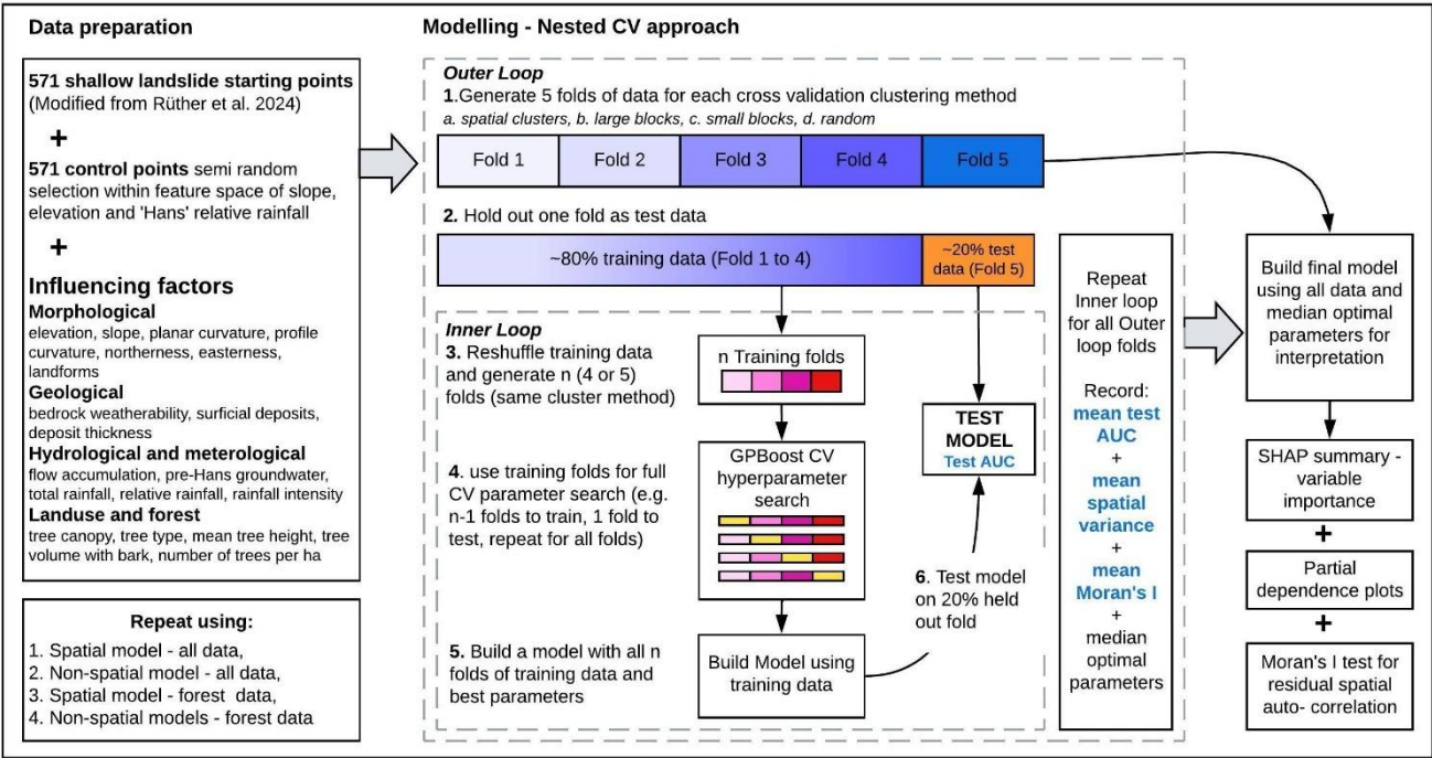
Figure 3 Flowchart summarising data and methods for the nested cross-validation (CV) approach presented in this study. For each of the four model types listed (1. to 4., bottom left), the nested CV workflow was completed using four different CV clustering methods (a. to d., specified under step 1). The methodology for additional modelling runs following a simpler approach is presented in Appendix B.
