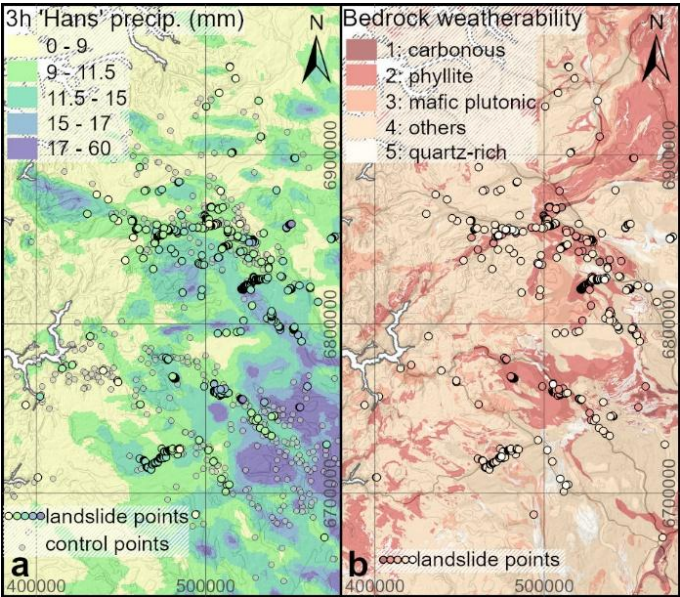
Figure 8 a) Maximum 3h precipitation summed up for the ‘Hans’ time period based on the MET Nordic dataset, shallow landslide starting points symbolised with colours corresponding to rainfall intensity and control points in transparent grey for reference b) Bedrock weatherability classes and shallow landslide starting points symbolised with colours corresponding to weatherability classes. © Kartverket, SeNorge, NGU.
