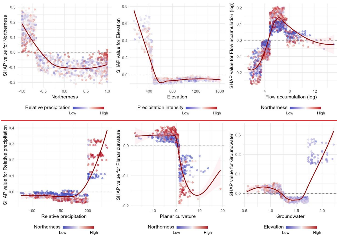
Figure 4 Partial dependence plots for the top six variables of the spatial model with small block nested CV (model 1c). Each point represents an observation and is plotted with its feature value on the x-axis and SHAP value (contribution to model output) on the y-axis. SHAP values above 0 indicate that a feature value is likely to make a positive contribution to the probability of a landslide. Points are coloured by a second feature chosen to minimise the variance of the SHAP value given both features and represents the strongest interaction. Solid red lines are LOESS smoothed lines and shading represents 95% confidence intervals.
