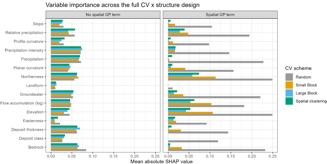
465 Figure 4 Full factorial comparison of variable importance scores for the full dataset, comparing non-spatial (No spatial GP term) with spatial (Spatial GP term) models built with all four cross-validation (CV) schemes. Variable importance was quantified using mean absolute SHAP (SHapley Additive exPlanations) values.
