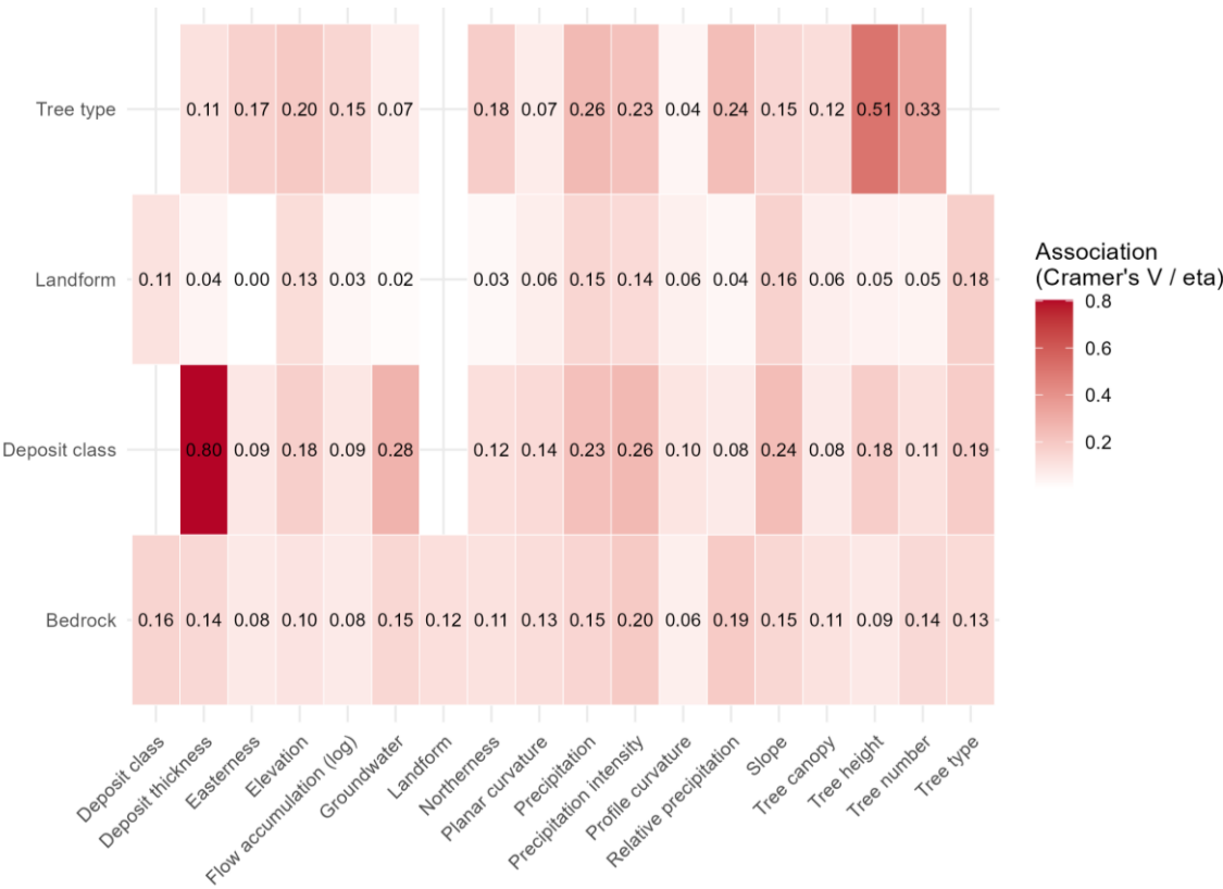
Figure D4 Heat map of associations between categorical variables and all other variables retained in the models using the forest dataset. Values between the categorical variables are Cramer's V, and values between categorical and continuous/ordinal variable pairs are correlation ratio ( \eta , derived from one-way ANOVA).
