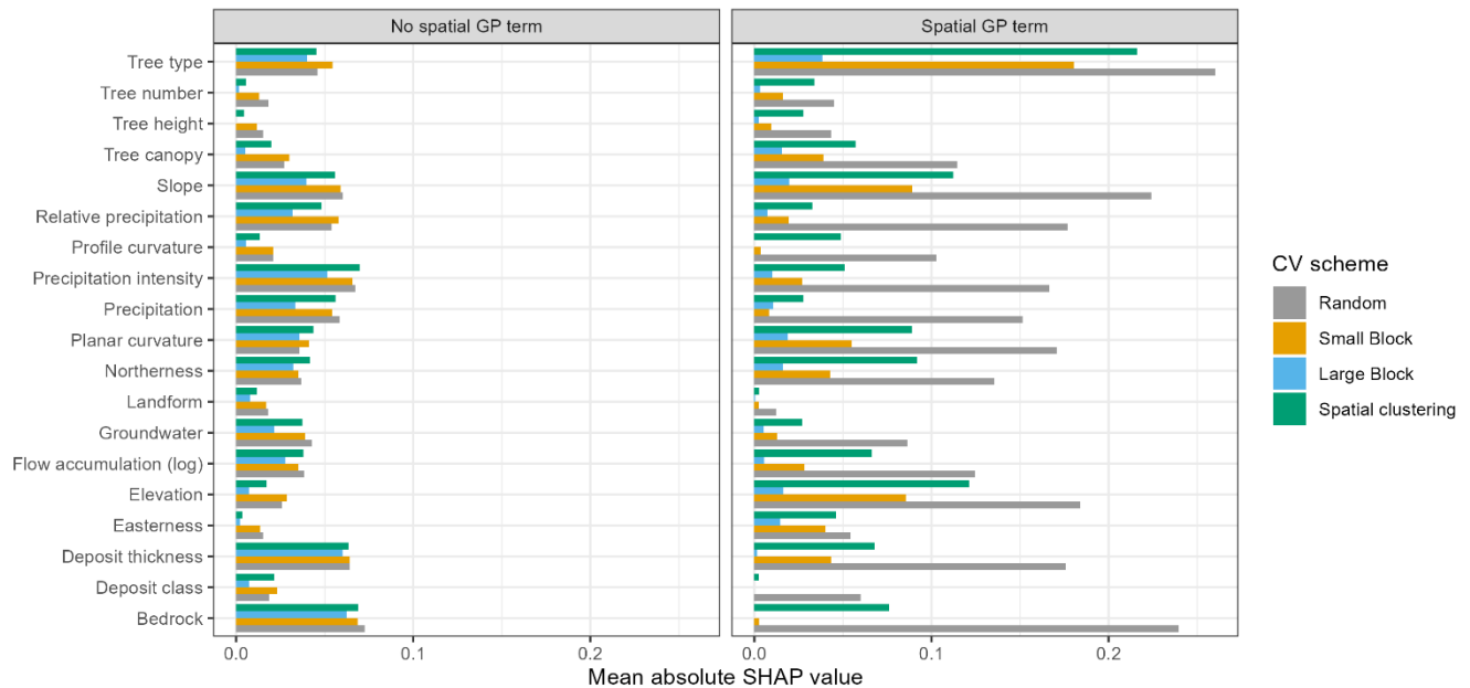
Variable importance across the full CV x structure design
