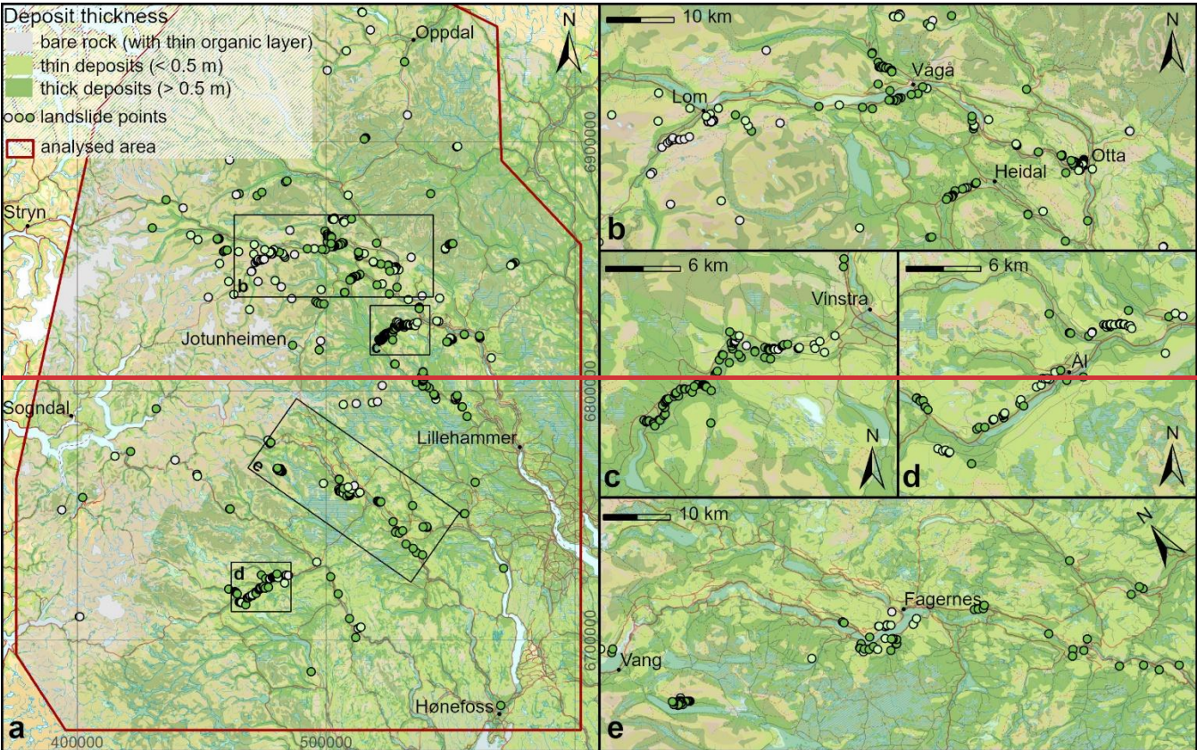
895 Figure 10 Spatial distribution of the categorical variable deposit thickness and shallow landslide starting points symbolised with corresponding colours for a) the entire study area, b) Ottadalen, c) Skåbudalen, d) inner Hallingdal and e) Valdres. © Kartverket, NGU.
