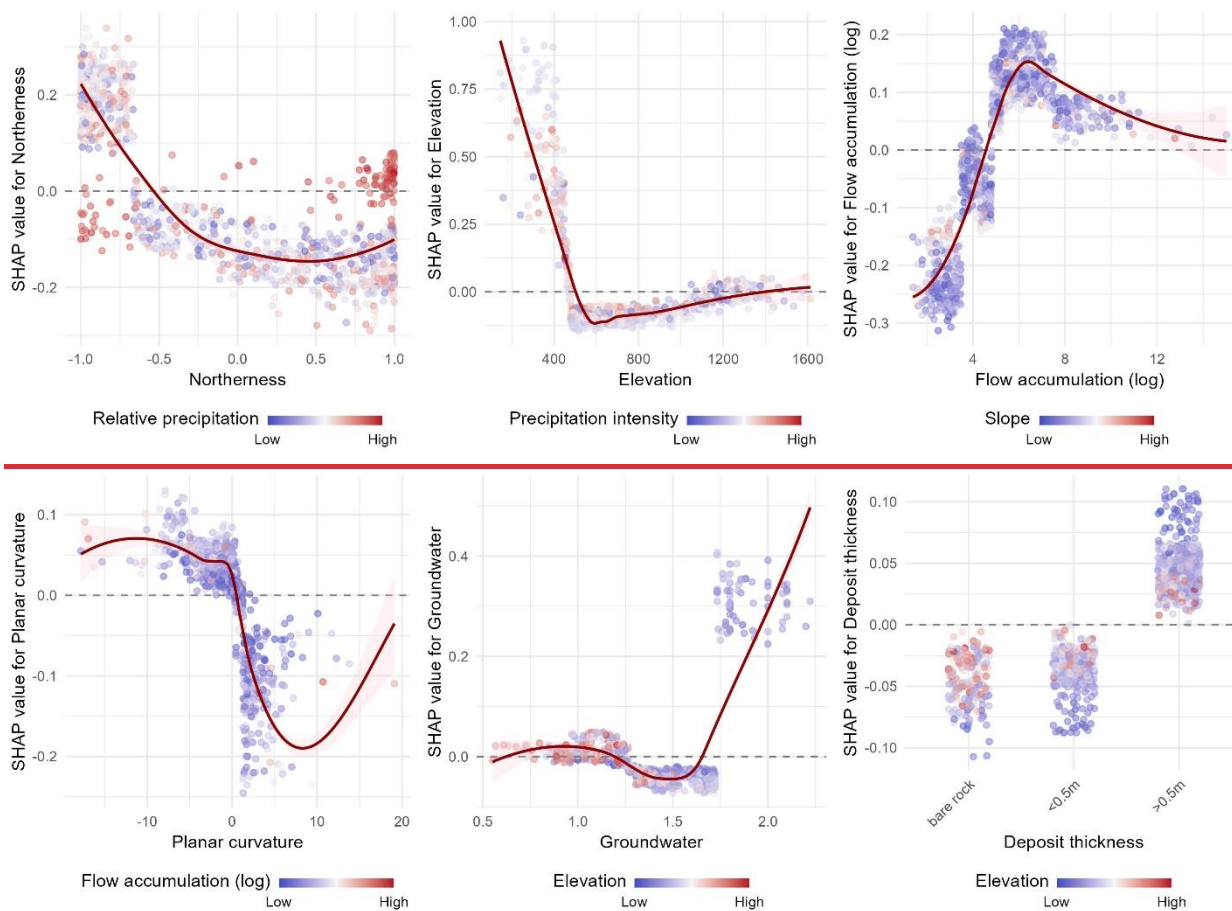
Figure B3 Partial dependence plots for the top six variables of the spatial model S1c with small block CV on the full dataset, using the simple CV approach. Each point represents an observation and is plotted with its feature value on the x axis, and SHAP value (contribution to model output) on the y axis. SHAP values above 0 indicate that a feature value is likely to make a positive contribution to the probability of a landslide. Points are coloured by a second feature chosen to minimise the variance of the SHAP value given both features and represents the strongest interaction. Solid red lines are LOESS smoothed lines.
