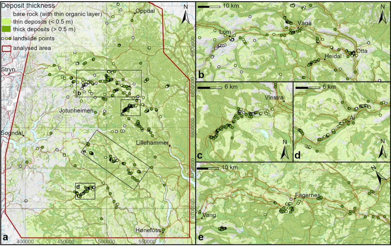
875 Figure 10 Spatial distribution of the categorical variable deposit thickness and shallow landslide starting points symbolised with corresponding colours for a) the entire study area, b) Ottadalen, c) Skåbudalen, d) inner Hallingdal and e) Valdres. © Kartverket, NGU.
