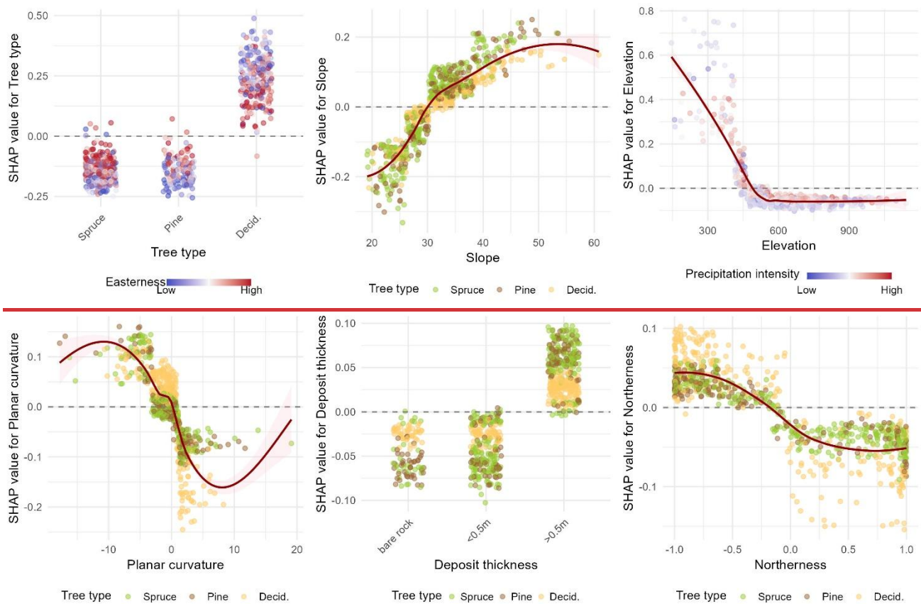
Figure 6 Partial dependence plots for the top six variables of the spatial model with small block nested CV for the forest-only data (model 3c). Each point represents an observation and is plotted with its feature value on the x-axis and SHAP value (contribution to model output) on the y-axis. SHAP values above 0 indicate that a feature value is likely to make a positive contribution to the probability of a landslide. Points are coloured by a second feature chosen to minimise the variance of the SHAP value given both features and represents the strongest interaction. Solid red lines are LOESS smoothed lines.
