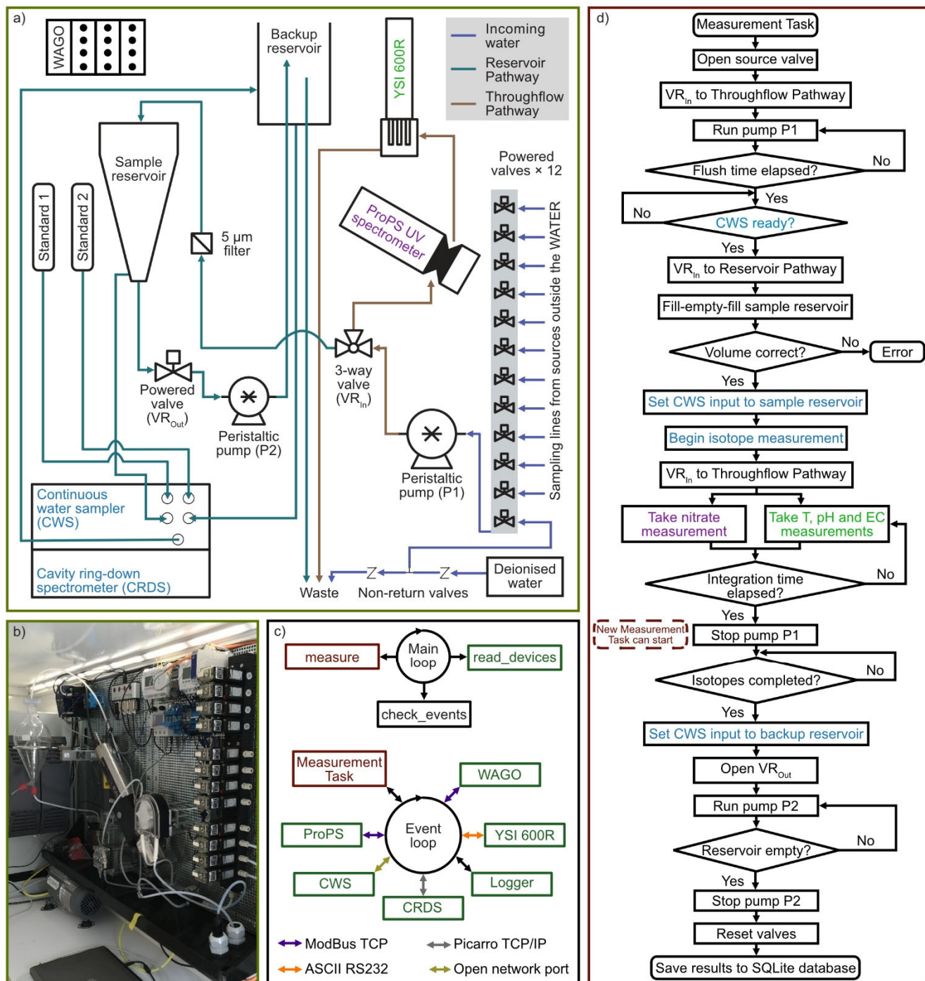
180 Fig 1: a) Schematic of the automated sample acquisition and measurement system in the WATER; b) photo of the valve and pump system, ProPS, YSI600R and sample reservoir; c) schematic of the main software loop and event loop (coloured arrows in the latter denote the method of interfacing with devices whilst a black arrow indicates a software connection); d) flow chart for a Measurement Task (coloured text denotes the device used in measurement acquisition and corresponds to device labelling in a).
