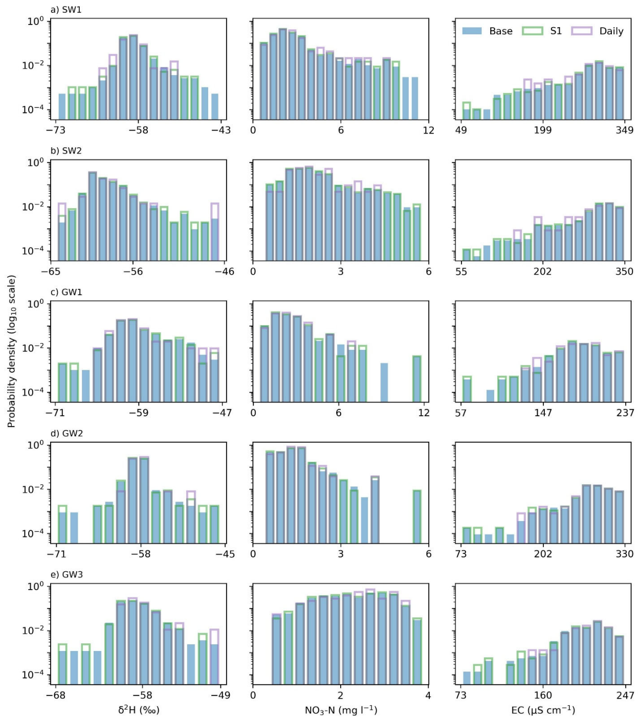
Fig 6: For each water source (a-e), probability density functions estimated via histograms for the deuterium ( \delta^2\text{H} ), nitrate ( \text{NO}_3\text{-N} ), and electrical conductivity (EC) data collected under the Baseline and two alternative sampling scenarios. Note that probability density is on a \log_{10} scale to aid visualisation and x-axes are unique to each site and parameter.
