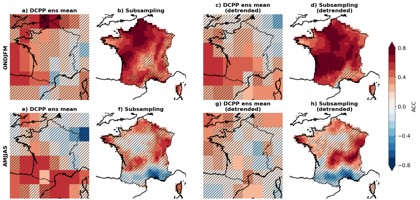
Fig. 11: Precipitation prediction skill for the DCP-P-A ensemble mean and the subsampling method, for extended winter (ONDJFM, a–d) and extended summer (AMJJAS, e–h), evaluated against ERA5 over 1966–2019. Panels (a, e): ACC between the DCP-P-A multi-model ensemble mean and ERA5 remapped to 2°. Panels (b, f): ACC between subsampling predictions (wNAO-based for winter; sNAO+uAMV-based for summer) and ERA5 at 0.25°. Panels (c, g) and (d, h): same as (a, e) and (b, f), respectively, but computed after removal of the linear trend from both predictions and observations, isolating skill arising from internal climate variability rather than the externally forced signal. Note that panels (a, c, e, g) are evaluated on a 2° grid while panels (b, d, f, h) are evaluated on a 0.25° grid, reflecting the respective native or target resolutions of the two systems; a direct gridpoint-by-gridpoint skill comparison is therefore not computed. Hatched areas indicate regions where skill scores are not statistically significant at the 95% confidence level, assessed using a 1,000-sample block bootstrap.
