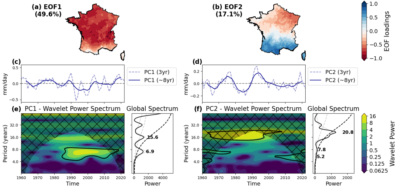
Fig. 4: Spatial and temporal variability of summer (AMJJAS) precipitation over France (1960-2023). Panels (a) and (b) show the spatial patterns of the first two Empirical Orthogonal Function (EOF) modes of 3-year running mean summer precipitation anomalies from SAFRAN observations, with the percentage of total variance explained shown in parentheses. Colors represent the spatial loadings of each mode expressed as correlations with the principal components. Panels (c) and (d) depict the corresponding principal components (PCs) time series in mm/day, with dashed and solid blue lines denoting the raw PCs from 3-year means and the low-frequency filtered PCs of around 8 years, respectively. Panels (e) and (f) present the wavelet power spectra (left) and global wavelet power spectra (right) for EOF1 and EOF2 PCs, respectively. In the wavelet spectra, the x-axis is time, and the y-axis is period in years; warmer colors denote higher power. Black contours in the wavelet spectra indicate the 95% confidence level against a red noise background, while shaded regions depict the cone of influence (COI) where edge effects may influence the results. The global spectra display the time-averaged wavelet power (solid black line) and the Fourier power (solid gray line), with dashed lines corresponding to the 95% significance levels.
