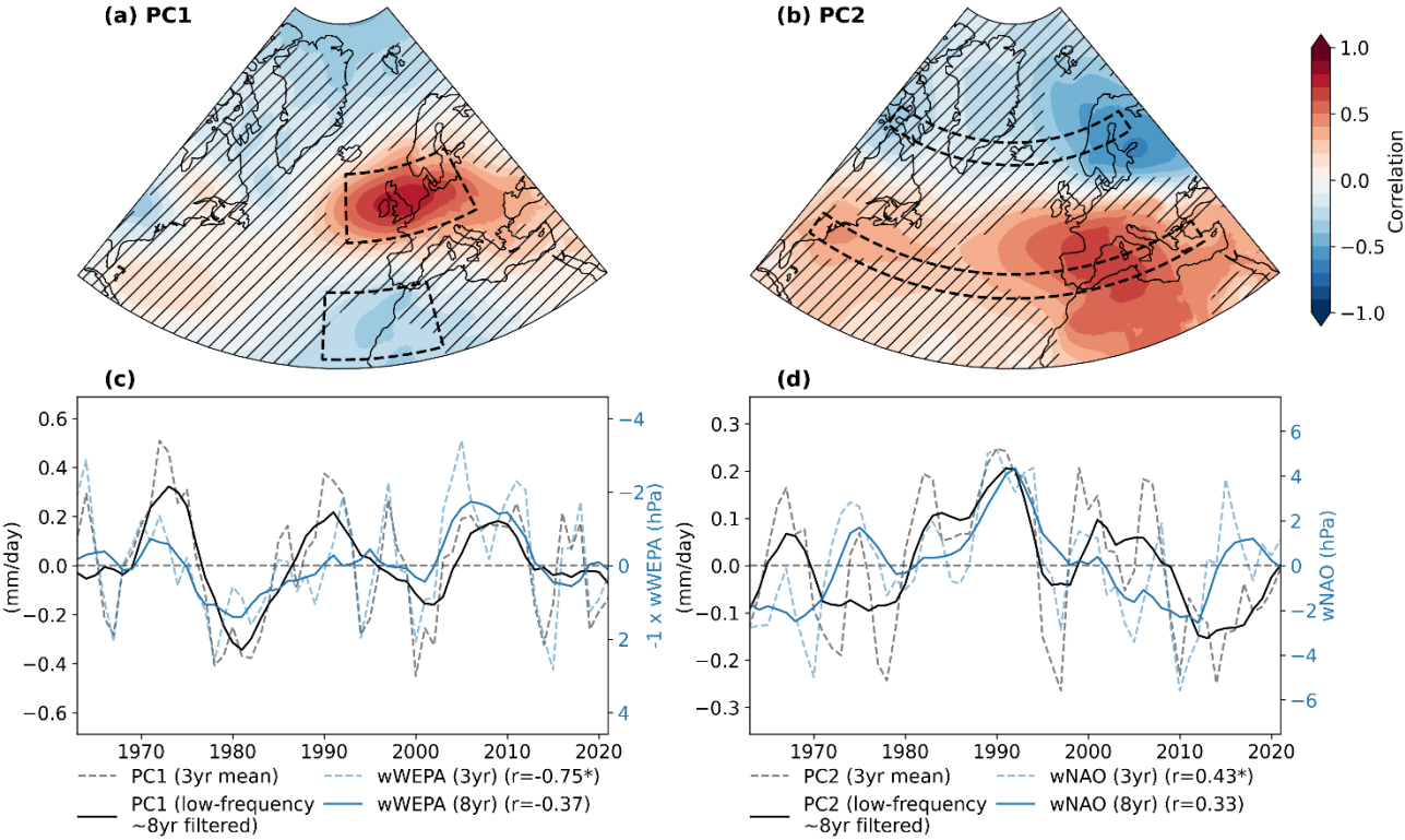
Fig. 3: Relationship between winter (ONDJFM) precipitation variability and large-scale North Atlantic atmospheric circulation. Panels (a) and (b) display spatial maps of correlations between the first two precipitation PCs (PC1 and PC2) and SLP anomalies over the North Atlantic. Hatched areas denote statistically non-significant correlations at the 95% confidence level based on a block-bootstrap test. Black dashed boxes outline the spatial domains used to compute the wWEPA (panel a) and wNAO indices (panel b). Panels (c) and (d) compare the time series of precipitation PCs (black lines) with their corresponding SLP indices (blue lines), including 3-year running mean (dashed) and low-frequency (~8-year) filtered (solid). Reported correlation coefficients ( r ) correspond to both smoothing scales. Units for the precipitation PCs are mm/day, for the SLP indices are hPa.
