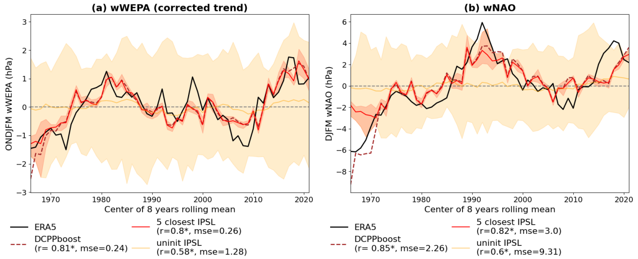
Fig. 6: Observed and predicted decadal variability of winter atmospheric indices. Panels (a) and (b) show 8-year running mean of the wWEPA and wNAO indices for extended winter seasons (ONDJFM and DJFM respectively). The black line represents ERA5 reanalysis, while the burgundy dashed line shows predictions from the boosted DCP method. The red shading indicates the spread of the five subsampled members, best matching DCP indices and selected from the uninitialized IPSL-CM6A-LR ensemble in each 8-year time window, with the bold red line marking their ensemble mean. The yellow line and shading represent the mean and full spread (minimum to maximum) of the entire uninitialized IPSL ensemble, respectively. Correlation coefficients and p-values between predictions and observations are reported in parentheses of each panel's legend.
