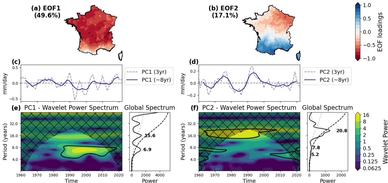
385 Fig. 4: Spatial and temporal variability of summer (AMJJAS) precipitation over France (1960-2023). Panels (a) and (b) show the spatial patterns of the first two Empirical Orthogonal Function (EOF) modes of 3-year running mean summer precipitation anomalies from SAFRAN observations, with the percentage of total variance explained shown in parentheses. Colors represent the spatial loadings of each mode expressed as correlations with the principal components. Panels (c) and (d) depict the corresponding principal components (PCs) time series in mm/day, with dashed and solid blue lines denoting the raw PCs from 3-year means and the low-frequency filtered PCs of around 8 years, respectively. Panels (e) and (f) present the wavelet power spectra (left) and global wavelet power spectra (right) for EOF1 and EOF2 PCs, respectively. In the wavelet spectra, the x-axis is time, and the y-axis is period in years; warmer colors denote higher power. Black contours in the wavelet spectra indicate the 95% confidence level against a red noise background, while shaded regions depict the cone of influence (COI) where edge effects may influence the results. The global spectra display the time-averaged wavelet power (solid black line) and the Fourier power (solid gray line), with dashed lines corresponding to the 95% significance levels.
