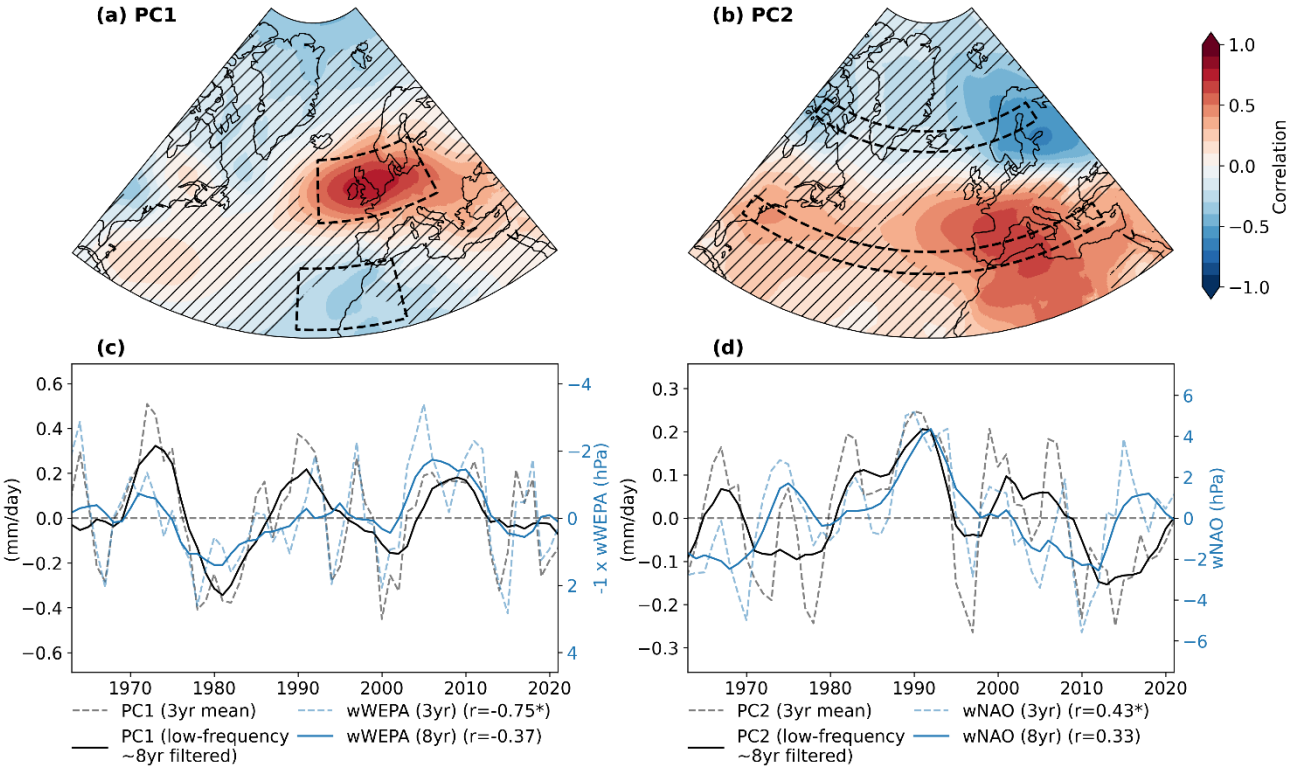
370 Fig. 3: Relationship between winter (ONDJFM) precipitation variability and large-scale North Atlantic atmospheric circulation. Panels (a) and (b) display spatial maps of correlations between the first two precipitation PCs (PC1 and PC2) and SLP anomalies over the North Atlantic. Hatched areas denote statistically non-significant correlations at the 95% confidence level based on a block-bootstrap test. Black dashed boxes outline the spatial domains used to compute the wWEPA (panel a) and wNAO indices (panel b). Panels (c) and (d) compare the time series of precipitation PCs (black lines) with their corresponding SLP indices (blue lines), including 3-year running mean (dashed) and low-frequency (~8-year) filtered (solid). Reported correlation coefficients ( r ) correspond to both smoothing scales. Units for the precipitation PCs are mm/day, for the SLP indices are hPa.
