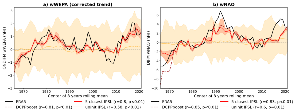
415 Fig. 6: Observed and predicted decadal variability of winter atmospheric indices. Panels (a) and (b) show 8-year running mean of the wWEPA and wNAO indices for extended winter seasons (ONDJFM and DJFM respectively). The black line represents ERA5 reanalysis, while the burgundy dashed line shows predictions from the boosted DCP method. The red shading indicates the spread of the five subsampled members, best matching DCP indices and selected from the uninitialized IPSL-CM6A-LR ensemble in each 8-year time window, with the bold red line marking their ensemble mean. The yellow line and shading represent the mean and full spread (minimum to maximum) of the entire uninitialized IPSL ensemble, respectively. Correlation coefficients and p-values 420 between predictions and observations are reported in parentheses of each panel's legend.
