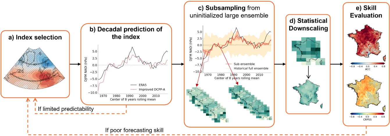
Fig. 1: Schematic workflow of the proposed framework for decadal prediction of hydroclimate variables: (a) identifying the most relevant large-scale index (here, wNAO), showing the strongest correlation with the target hydroclimate variable (here, winter precipitation); (b) predicting the selected index using improved decadal forecasts from the DCP database; (c) selecting ensemble members from an uninitialized climate model that best reproduce the predicted index; (d) aggregating, bias-correcting and downscaling the resulting sub-ensemble predictions to the 8-km spatial resolution; (e) Evaluating forecast skill using temporal metrics (e.g., ACC and CRPSS).
