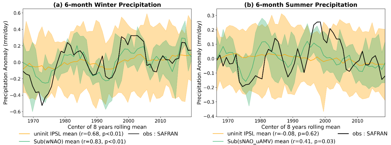
525 Fig. 10: Panel (a) and (b) show 8-year running mean precipitation anomalies for winter (ONDJFM) and summer (AMJJAS), respectively, averaged over the region outlined by dashed boxes in Figs. 8 and 9. The black line shows SAFRAN observations. The green line represents the mean of the five-member sub-ensemble selected based on the wNAO index (panel a) and combined sNAO+uAMV indices (panel b). The yellow line shows the mean of the full uninitialized IPSL ensemble. Shaded areas indicate the 530 ensemble spread, defined as the 5th to 95th percentile range.
