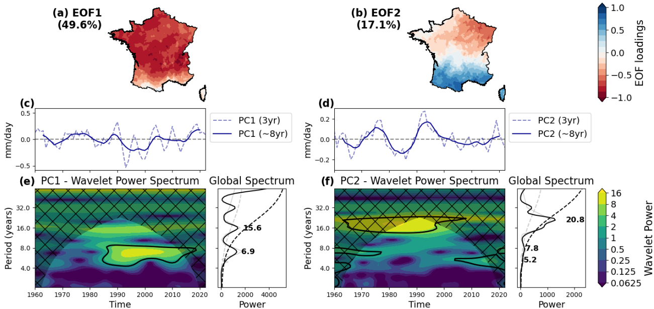
390 Fig. 4: Spatial and temporal variability of summer (AMJJAS) precipitation over France (1960-2023). Panels (a) and (b) show the spatial patterns of the first two Empirical Orthogonal Function (EOF) modes of 3-year running mean summer precipitation anomalies from SAFRAN observations, with the percentage of total variance explained shown in parentheses. Colors represent the spatial loadings of each mode expressed as correlations with the principal components. Panels (c) and (d) depict the corresponding principal components (PCs) time series in mm/day, with dashed and solid blue lines denoting the raw PCs from 3-year means and the low-frequency filtered PCs of around 8 years, respectively. Panels (e) and (f) present the wavelet power spectra (left) and global wavelet power spectra (right) for EOF1 and EOF2 PCs, respectively. In the wavelet spectra, the x-axis is time, and the y-axis is period in years; warmer colors denote higher power. Black contours in the wavelet spectra indicate the 95% confidence level against a red noise background, while shaded regions depict the cone of influence (COI) where edge effects may influence the results. The global spectra display the time-averaged wavelet power (solid black line) and the Fourier power (solid gray line), with dashed lines corresponding to the 95% significance levels.
