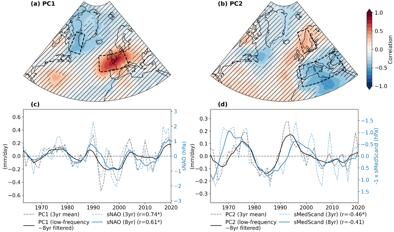
Fig. 5: Relationship between summer (AMJJAS) precipitation variability and large scale North Atlantic circulation. Panels (a) and (b) show the correlation patterns between summer precipitation PCs (PC1 and PC2) and SLP anomalies over the North Atlantic. Hatched areas indicate regions where correlations are statistically significant at the 95% confidence level based on a block-bootstrap test. Black dashed boxes outline the spatial domains used to compute the sNAO (panel a) and sMedScand indices (panel b). Panels (c) and (d) compare the time series of precipitation PCs (black lines) and their corresponding SLP indices (blue lines), including 3-year running mean (dashed) and low-frequency (~8-year) filtered (solid). Reported correlation coefficients (r) correspond to both smoothing scales. Units for the precipitation PCs are mm/day, and for the SLP indices are hPa.
