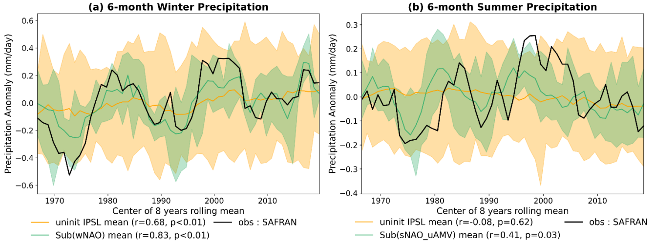
Fig. 10: Panel (a) and (b) show 8-year running mean precipitation anomalies for winter (ONDJFM) and summer (AMJJAS), respectively, averaged over the region outlined by dashed boxes in Figs. 8 and 9. The black line shows SAFRAN observations. The green line represents the mean of the five-member sub-ensemble selected based on the wNAO index (panel a) and combined sNAO+uAMV indices (panel b). The yellow line shows the mean of the full uninitialized IPSL ensemble. Shaded areas indicate the ensemble spread, defined as the 5th to 95th percentile range.
