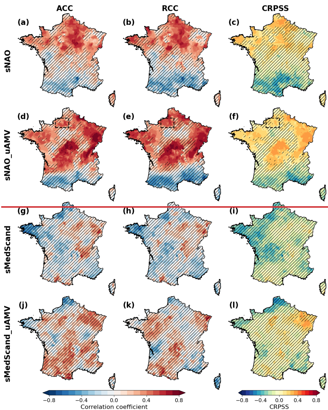
Fig. 9: Forecast skill for 8-year mean summer (AMJJAS) precipitation anomalies over France. Results are derived from subsampled hindcasts based on the sNAO (a–c), sNAO+uAMV (d–f), sMedScand (g–i) and sMedScand+uAMV (j–l) indices. Panels show (a,d) Anomaly Correlation Coefficient (ACC), (b,e) Residual Correlation Coefficient (RCC)—quantifying skill beyond the forced response—and (c,f) Continuous Ranked Probability Skill Score (CRPSS), all computed against SAFRAN precipitation observations over 1966–2019. Hatched regions indicate areas where skill scores are not statistically significant at the 95% confidence level, as assessed using a 1,000 sample block bootstrap. Dashed black boxes indicate a specific region illustrated in Fig. 10.
