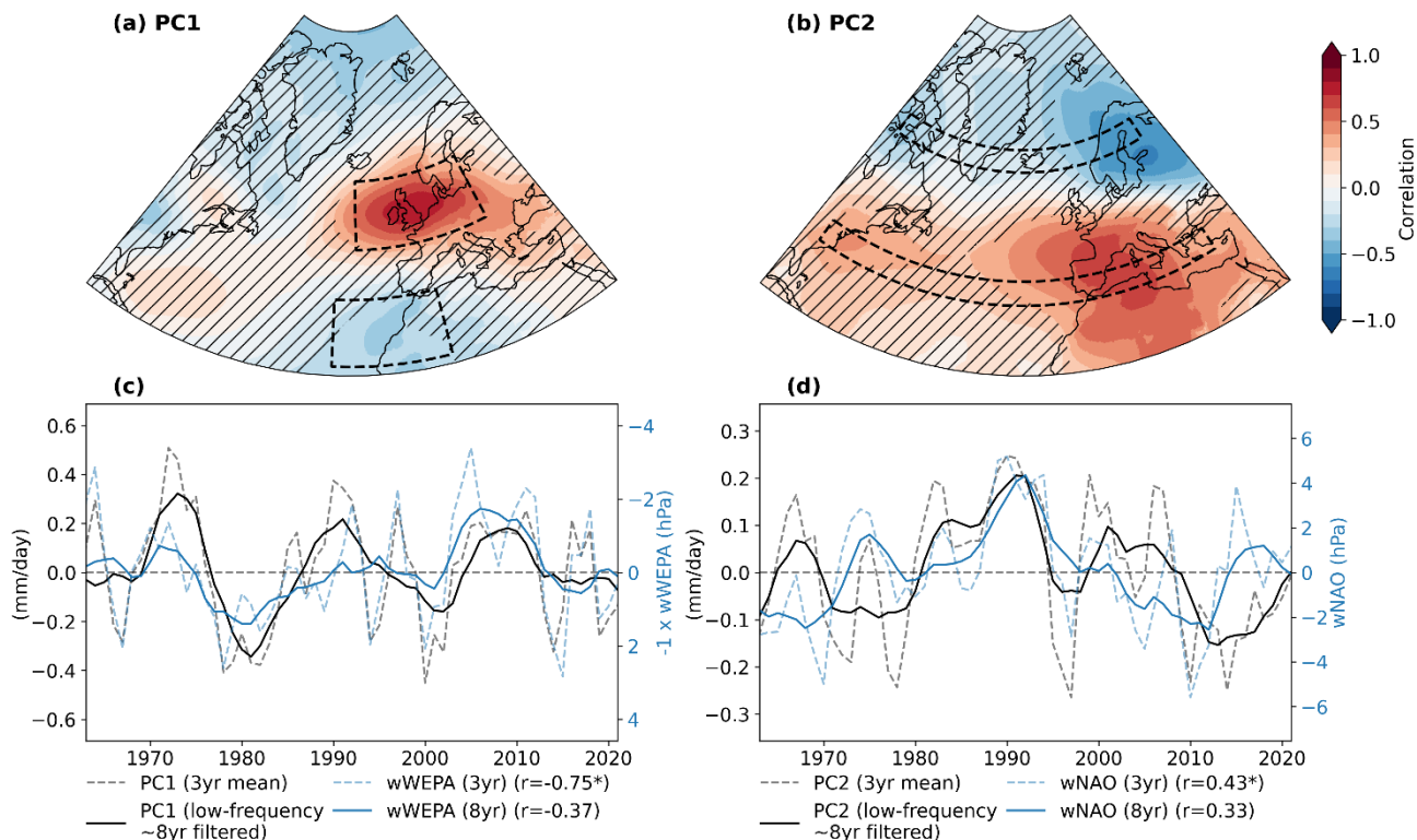
Fig. 3: Relationship between winter (ONDJFM) precipitation variability and large-scale North Atlantic atmospheric circulation. Panels (a) and (b) display spatial correlation maps of correlations between the first two precipitation PCs (PC1 and PC2) and SLP anomalies over the North Atlantic. Hatched areas denote statistically non-significant correlations at the 95% confidence level based on a block-bootstrap test. Black dashed boxes outline the spatial domains used to compute the wWEPA (panel a) and wNAO indices (panel b). Panels (c) and (d) compare the time series of precipitation PCs (black lines) with their corresponding SLP indices (blue lines), including 3-year running mean (dashed) and low-frequency (~8-year) filtered (solid). Reported correlation coefficients ( r ) correspond to both smoothing scales. Units for the precipitation PCs are mm/day, for the SLP indices are hPa.
