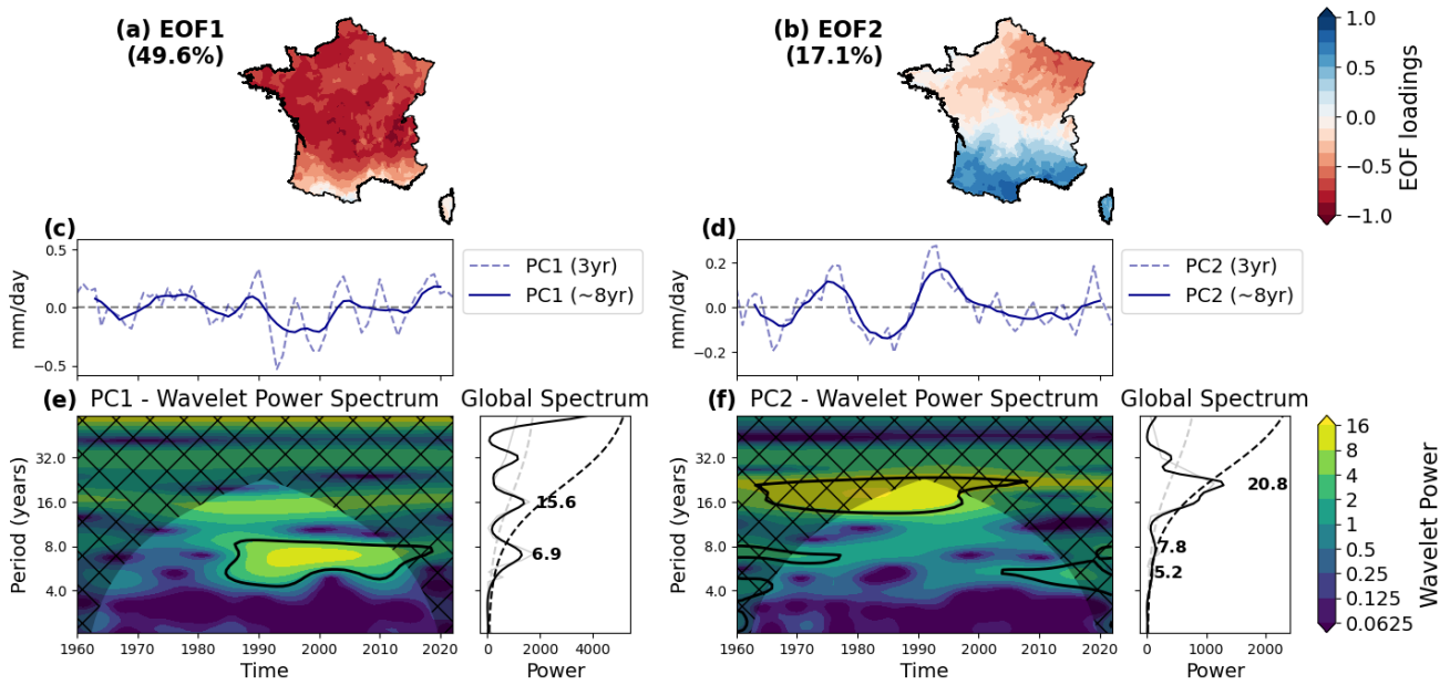
395 Fig. 4: Spatial and temporal variability of summer (AMJJAS) precipitation over France (1960-2023). Panels (a) and (b) show the spatial patterns of the first two Empirical Orthogonal Function (EOF) modes of 3-year running mean summer precipitation anomalies from SAFRAN observations, with the percentage of total variance explained shown in parentheses. Colors represent the spatial loadings of each mode expressed as correlations with the principal components. Panels (c) and (d) depict the corresponding principal components (PCs) time series in mm/day, with dashed and solid blue lines denoting the raw PCs from 3-year means and 400 the low-frequency filtered PCs of around 8 years, respectively. Panels (e) and (f) present the wavelet power spectra (left) and global wavelet power spectra (right) for EOF1 and EOF2 PCs, respectively. In the wavelet spectra, the x-axis is time, and the y-axis is period in years; warmer colors denote higher power. Black contours in the wavelet spectra indicate the 95% confidence level against a red noise background, while shaded regions depict the cone of influence (COI) where edge effects may influence the results. The global spectra display the time-averaged wavelet power (solid black line) and the Fourier power (solid gray line), with dashed lines 405 corresponding to the 95% significance levels.
