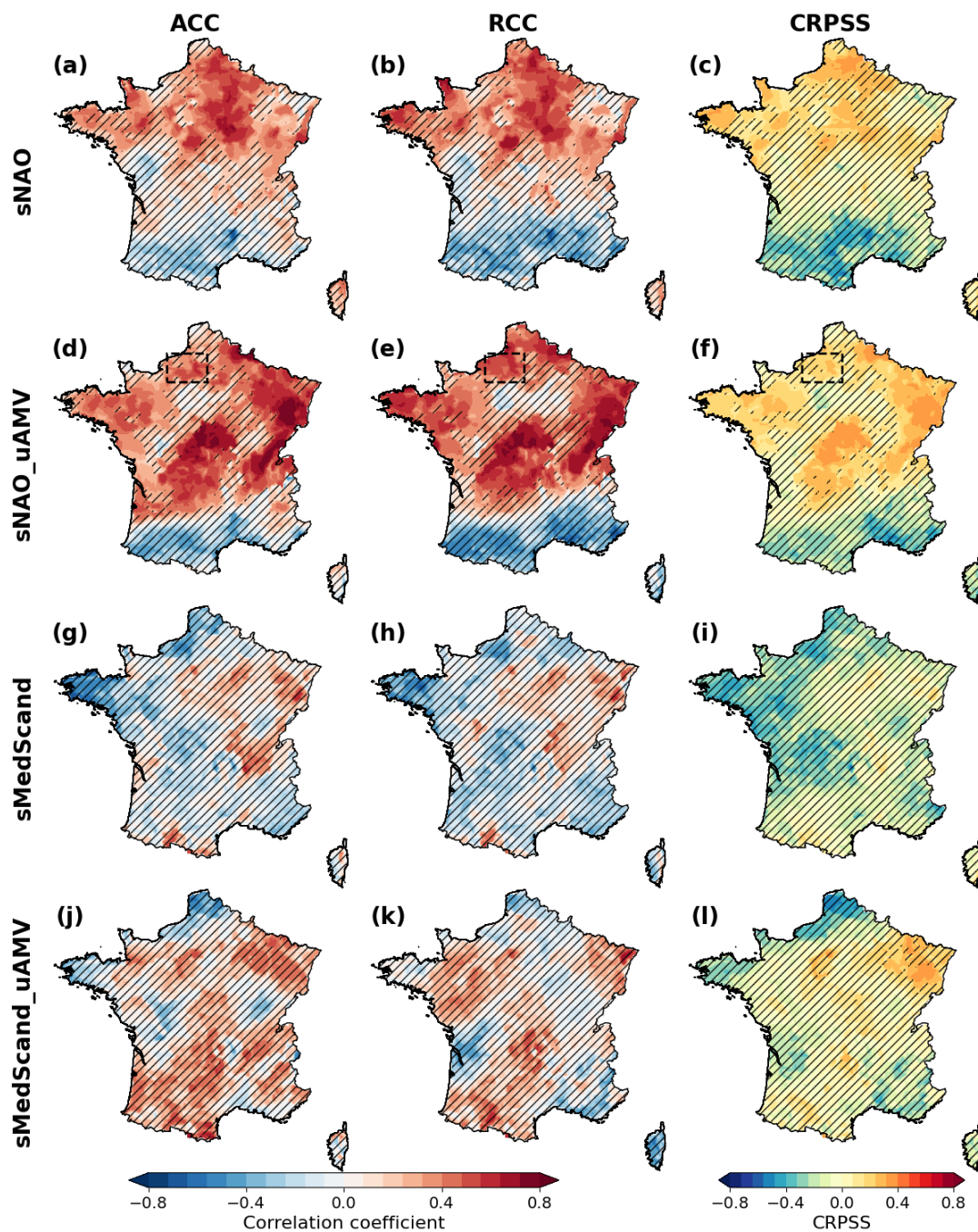
Fig. 9: Forecast skill for 8-year mean summer (AMJJAS) precipitation anomalies over France. Results are derived from subsampled hindcasts based on the sNAO (a–c), sNAO+uAMV (d–f), sMedScand (g–i) and sMedScand+uAMV (j–l) indices. Panels show (a,d) Anomaly Correlation Coefficient (ACC), (b,e) Residual Correlation Coefficient (RCC)—quantifying skill beyond the forced response—and (c,f) Continuous Ranked Probability Skill Score (CRPSS), all computed against SAFRAN precipitation observations over 1966–2019. Hatched regions indicate areas where skill scores are not statistically significant at the 95% confidence level, as assessed using a 1000 1,000 sample block bootstrap. Dashed black boxes indicate a specific region illustrated in Fig. 10.
