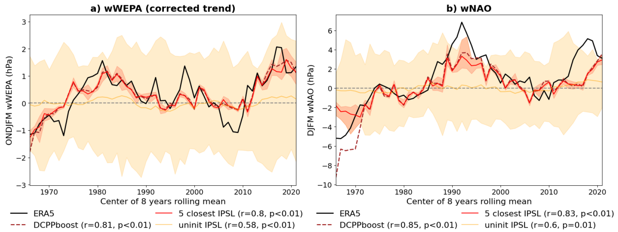
Fig. 6: Observed and predicted decadal variability of winter atmospheric indices. Panels (a) and (b) show 8-year running mean of the wWEPA and wNAO indices for extended winter seasons (ONDJFM and DJFM respectively). The black line represents ERA5 reanalysis, while the burgundy dashed line shows predictions from the boosted DCPM method. The red shading indicates the spread of the five subsampled members, best matching DCPM indices and selected from the uninitialized IPSL-CM6A-LR ensemble in each 8-year time window, with the bold red line marking their ensemble mean. The yellow line and shading represent the mean and full spread (minimum to maximum) of the entire uninitialized IPSL ensemble, respectively. Correlation coefficients and p-values between predictions and observations are reported in parentheses of each panel's legend.
