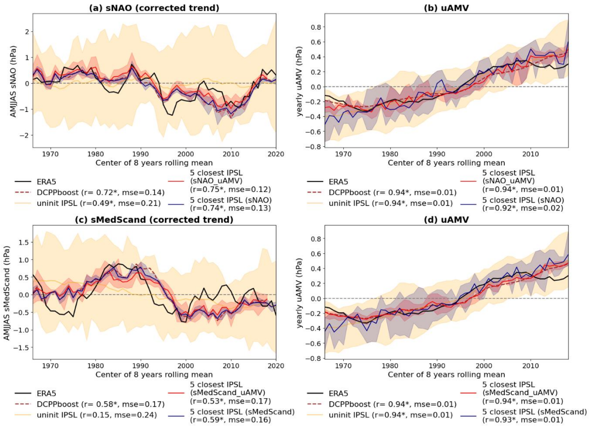
Fig. 7: Observed and predicted decadal variability of summer atmospheric large-scale indices. Panels (a) and (c) show 8-year running means of the sNAO and sMedScand indices for the extended summer season (AMJJAS); panels (b) and (d) show the uAMV index (note that the uAMV is shown twice, as it serves as the joint constraint in both the sNAO+uAMV and sMedScand+uAMV subsampling configurations). The black line represents ERA5 reanalysis, while, and the burgundy dashed line shows predictions from the boosted DCP method. The red shading indicates the spread of the five subsampled members, best matching DCP indices and predictions. In each 8-year sliding window, five members are selected from the uninitialized IPSL-CM6A-LR ensemble in each 8 year time window, with by minimizing the combined MSE loss function (Eq. 2). The red shading and bold red line marking their show the spread and ensemble mean of the five members selected using both indices jointly (sNAO+uAMV in panels a–b; sMedScand+uAMV in panels c–d). The blue shading and bold blue line show the spread and ensemble mean of the five members selected using the atmospheric index alone (sNAO in panels a–b; sMedScand in panels c–d). The yellow line and shading represent the mean and full spread (minimum to maximum) and mean of the entire uninitialized IPSL ensemble, respectively. Pearson correlation coefficients and p-values between predictions and observations (ACC) and mean squared errors (MSE) with ERA5 are reported in parenthesis of each panel's legend; stars indicate statistically significant ACC values at the 95% confidence level.
