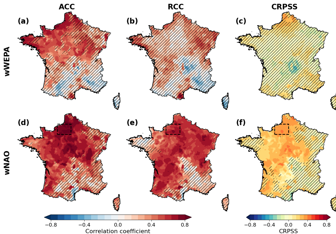
Fig. 8: Forecast skill for 8-year mean winter (ONDJFM) precipitation anomalies over France. Results are derived from subsampled hindcasts based on the wWEPA (a–c) and wNAO (d–f) indices. Panels show (a,d) Anomaly Correlation Coefficient (ACC), (b,e) Residual Correlation Coefficient (RCC)—quantifying skill beyond the forced response—and (c,f) Continuous Ranked Probability Skill Score (CRPSS), all computed against SAFRAN precipitation observations over 1966–2019. Hatched areas indicate regions where skill scores are not statistically significant at the 95% confidence level, as assessed using a 1000 sample block bootstrap. Dashed black boxes indicate a specific region illustrated in Fig. 10.
