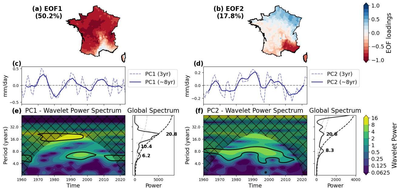
Fig. 2: Spatial and temporal variability of winter (ONDJFM) precipitation over France (1960-2023). Panels (a) and (b) show the spatial patterns of the first two Empirical Orthogonal Function (EOF) modes of 3-year running mean winter precipitation anomalies
