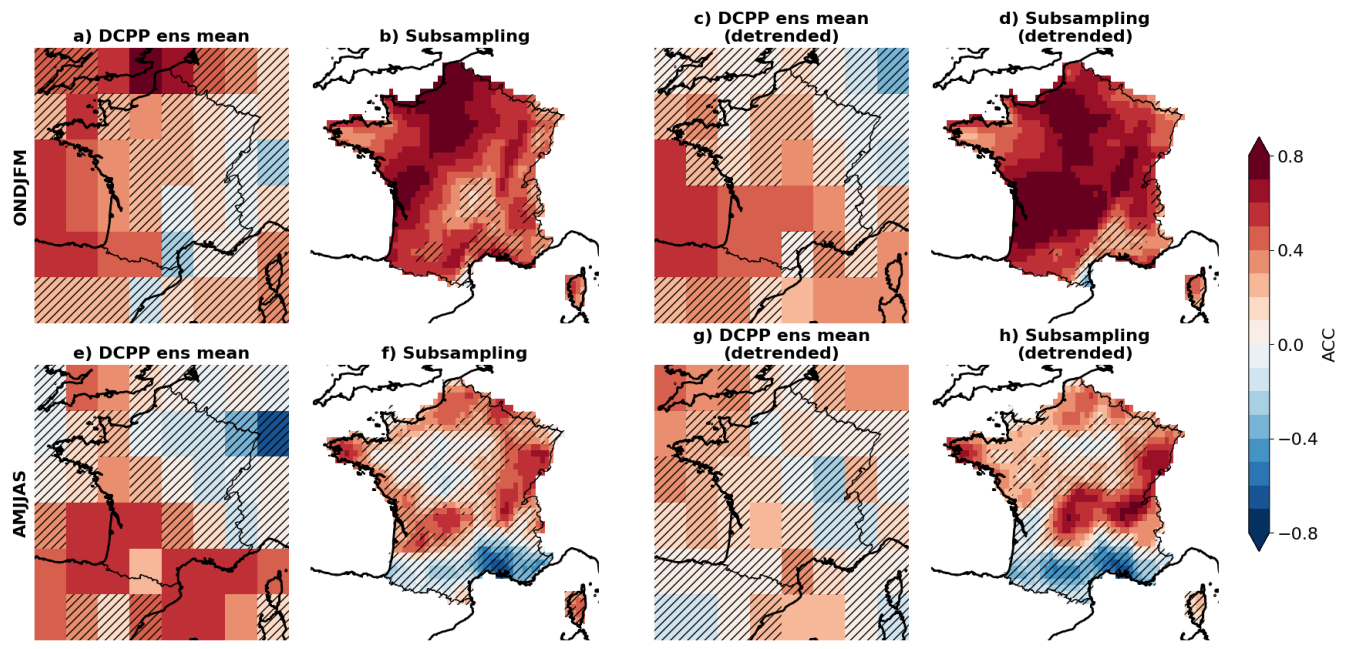
Fig. 11: Precipitation prediction skill for the DCP-A ensemble mean and the subsampling method, for extended winter (ONDJFM, a–d) and extended summer (AMJJAS, e–h), evaluated against ERA5 over 1966–2019. Panels (a, e): ACC between the DCP-A multi-model ensemble mean and ERA5 remapped to 2°. Panels (b, f): ACC between subsampling predictions (wNAO-based for winter; sNAO+uAMV-based for summer) and ERA5 at 0.25°. Panels (c, g) and (d, h): same as (a, e) and (b, f), respectively, but computed after removal of the linear trend from both predictions and observations, isolating skill arising from internal climate variability rather than the externally forced signal. Note that panels (a, c, e, g) are evaluated on a 2° grid while panels (b, d, f, h) are evaluated on a 0.25° grid, reflecting the respective native or target resolutions of the two systems; a direct gridpoint-by-gridpoint skill comparison is therefore not computed. Hatched areas indicate regions where skill scores are not statistically significant at the 95% confidence level, assessed using a 1,000-sample block bootstrap.
