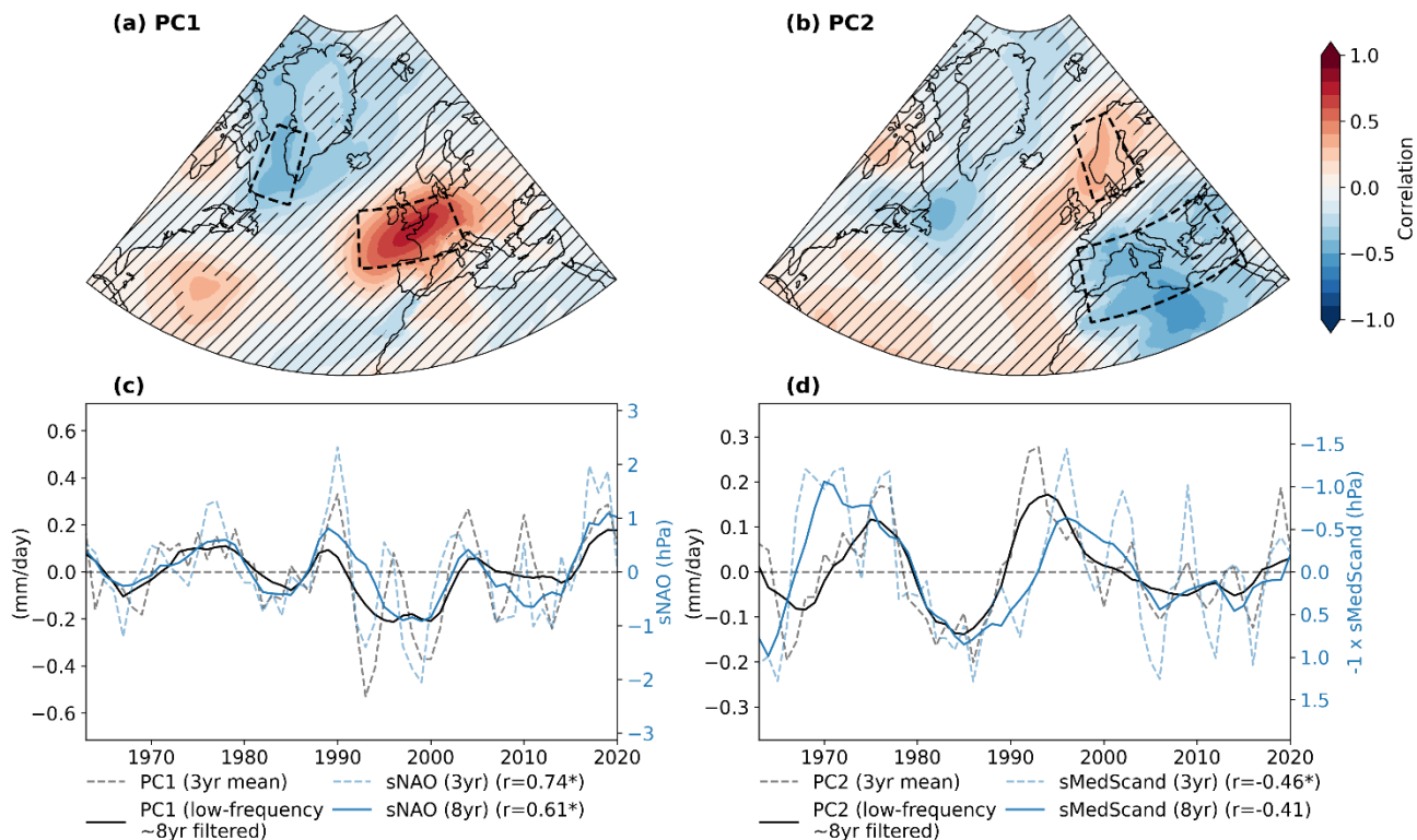
Fig. 5: Relationship between summer (AMJJAS) precipitation variability and large scale North Atlantic circulation. Panels (a) and (b) show the correlation patterns between summer precipitation PCs (PC1 and PC2) and SLP anomalies over the North Atlantic. Hatched areas indicate regions where correlations are statistically significant at the 95% confidence level based on a block-bootstrap test. Black dashed boxes outline the spatial domains used to compute the sNAO (panel a) and sMedScand indices (panel b). Panels (c) and (d) compare the time series of precipitation PCs (black lines) and their corresponding SLP indices (blue lines), including 3-year running mean (dashed) and low-frequency (~8-year) filtered (solid). Reported correlation coefficients (r) correspond to both smoothing scales. Units for the precipitation PCs are mm/day, and for the SLP indices are hPa.
