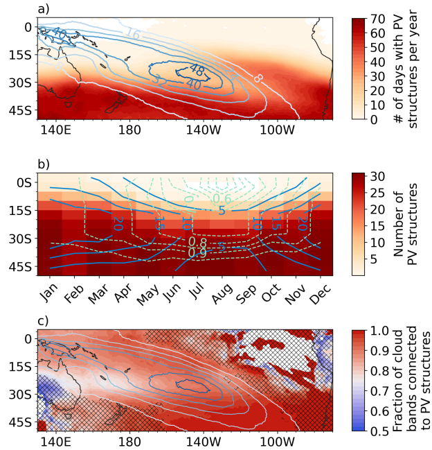
Figure 2. Climatologies of cloud bands and deep PV structures averaged between 1959–1979 and 2021 across the South Pacific. (a) Annual average frequency of PV structures (shading) and cloud bands (contours) in days per year. The contours represent the average number of days with cloud bands per year during the same period (representing local spatial density). (b) Seasonal cycle as a function of latitude, where PV structures (shading) and cloud bands (solid contours) are integrated zonally across the domain and expressed as the average number of occurrences per month. The dashed contours show the fraction of cloud bands connected to deep PV structures (interval: 0.1). (c) Annual average fraction of cloud bands connected to deep PV structures; when 0% of cloud bands are linked to PV structures, values are masked out (white shading). Hatching indicates areas where the 5% significance level is not met, according to a Monte Carlo test. Contours are the same as in panel a.
