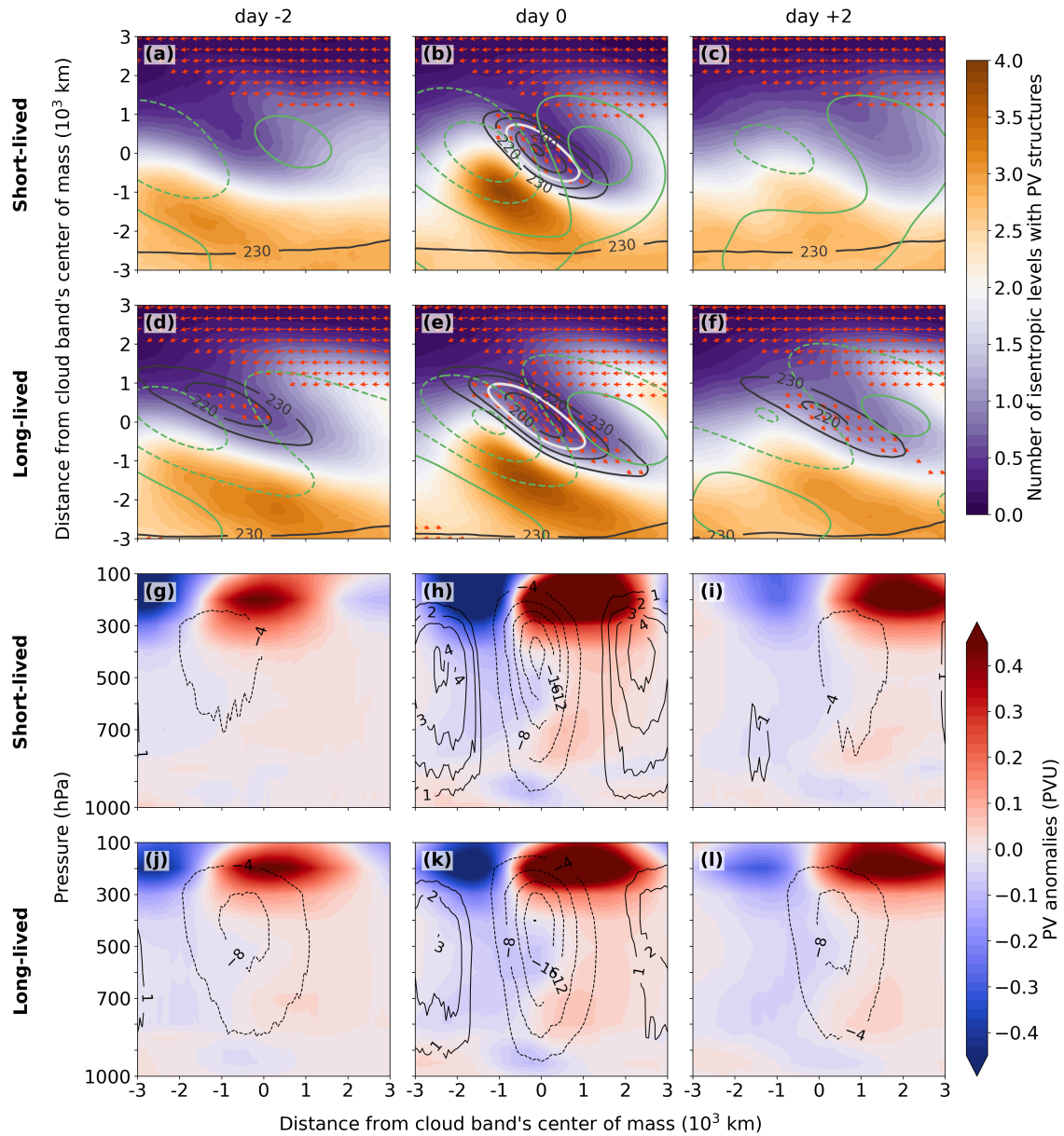
Figure 4. Same as Figure 3a–c but stratified by cloud band duration. (a)–(c) and (g)–(i) : short-lived cloud bands (duration 1–2 days), and (d)–(f) and (j)–(l) : persistent long-lived cloud bands (duration \geq 4 days).
