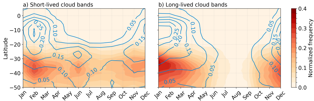
Figure 5. Seasonal cycle of zonal mean frequency for (a) short-lived and (b) persistent long-lived cloud bands (contours) and their connected PV structures (shading). Frequencies are normalized by the maximum value within each respective duration category (short-lived and persistent long-lived , respectively) to facilitate phase comparison.
