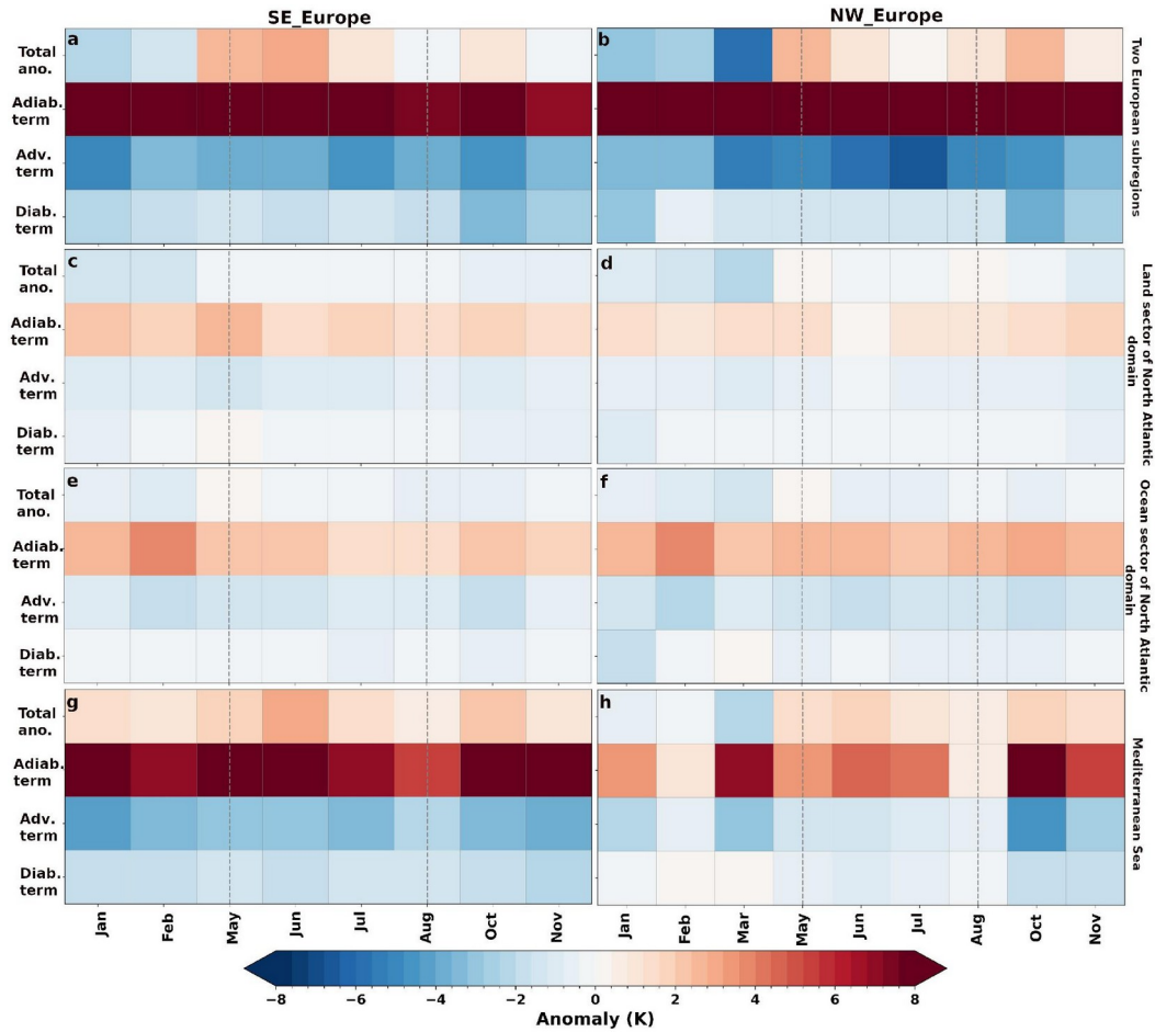
Figure 3: Monthly series of temperature anomaly sources during the 2022 European drought |
