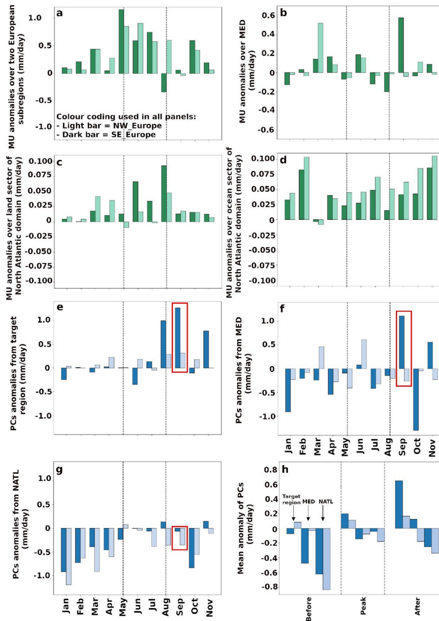
Figure 2: Moisture uptake (MU) and precipitation contributions (PCs) associated with the 2022 European drought | Colour bar intensity indicates each European subregion: higher intensity for SE_Europe and lower intensity for NW_Europe. The framed period highlights the peak drought months (May–August 2022). a–d MU monthly anomalies (in mm/day, green plots) computed over: a, each European subregion; b, the Mediterranean Sea; c, land; and d, ocean sectors of the North Atlantic domain. e–h Monthly anomalies of PCs (mm/day, blue bars) from: f, the Mediterranean (MED) moisture source; g, the NATL; and e, the two European subregions. The red rectangle indicates the month considered the drought-breaking month, September 2023. h Average PCs anomaly for each source for the periods Before (January–April), Peak (May–August), and After (September–November). The framed period highlights the active hydro-
