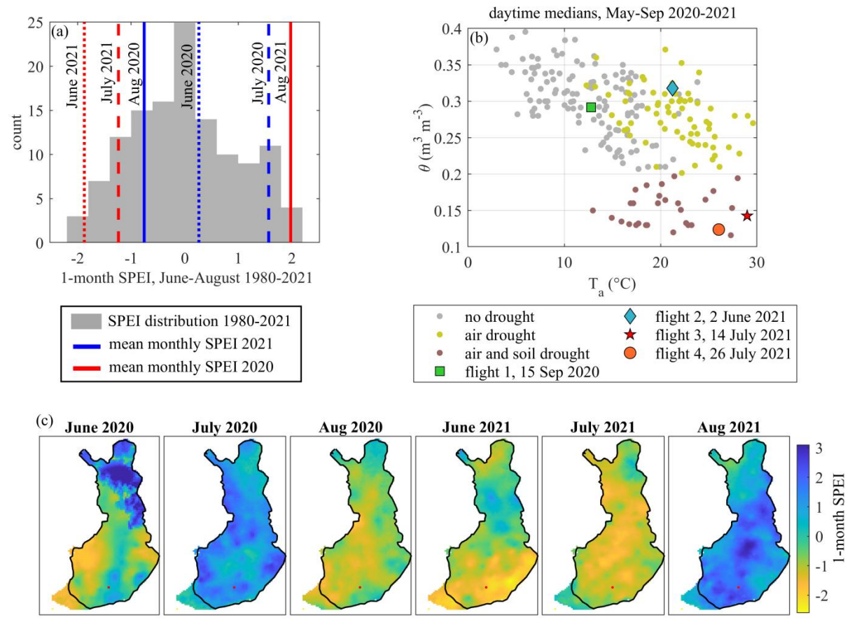
Figure 2. Meteorological characteristics of the 2020-2021 growing seasons (May-September) at the Ränskälänkorpi site. (a) Monthly SPEI drought index for the summer months of 2020 and 2021 for the location of Ränskälänkorpi site, with the 40-year distribution of monthly SPEI values for June-August shown with grey shading; the mean SPEI for the individual summer months in 2020 and 2021 is shown with blue and red lines, respectively; (b) daytime median soil moisture at 5 cm depth in the Harvest block versus air temperature; the UAV flight days are marked with special symbols; (c) monthly SPEI spatial distribution over the territory of Finland; the location of the Ränskälänkorpi site is marked with a red dot. Negative SPEI values indicate dry conditions.
