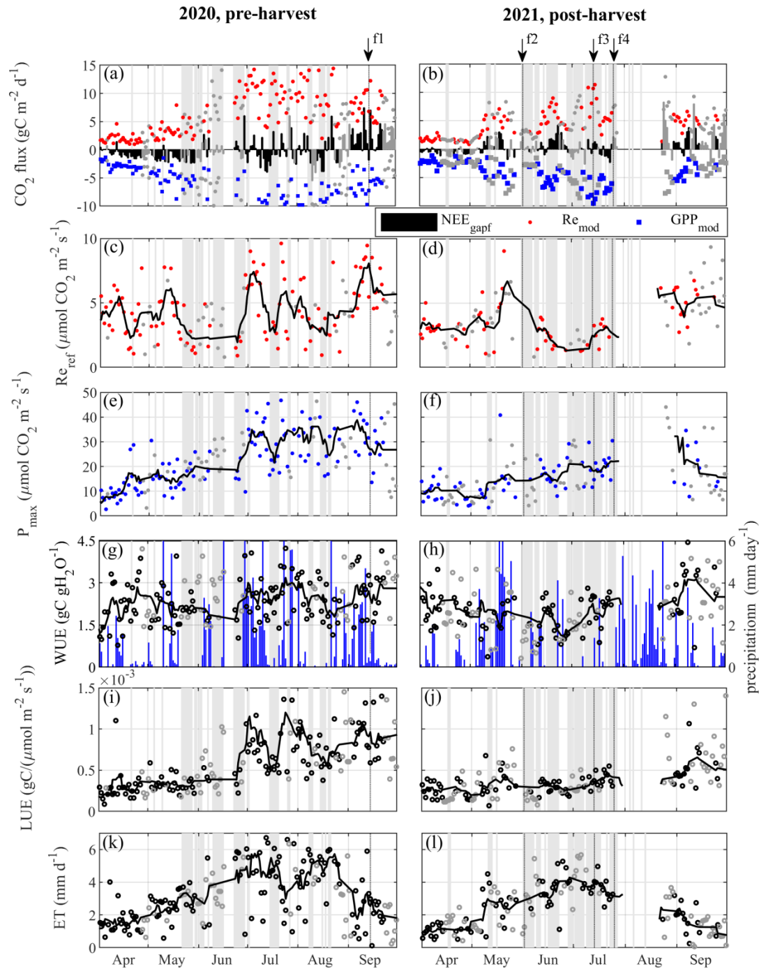
Figure 4. Time series of eddy-covariance derived fluxes in April-September of 2020 and 2021. (a,b) daily NEE, Re and GPP; (c,d) reference respiration ( Re_{ref} ); (e,f) light-saturated photosynthesis P_{max} ; (g-h) water use efficiency (WUE); (i-j) light use efficiency (LUE); (k-l) daily median eddy-covariance evapotranspiration (ET). The UAV flights are marked with arrows f1-f4. The shading is for the periods of VPD > 1 kPa. The coloured markers (a-f) and black markers (g-j) show the days of easterly wind (from the Harvest block), while the grey markers correspond to easterly winds (from the Control block). The smoothing averages (black bold lines) are calculated only using the days with the winds from the direction of the Harvest block.
