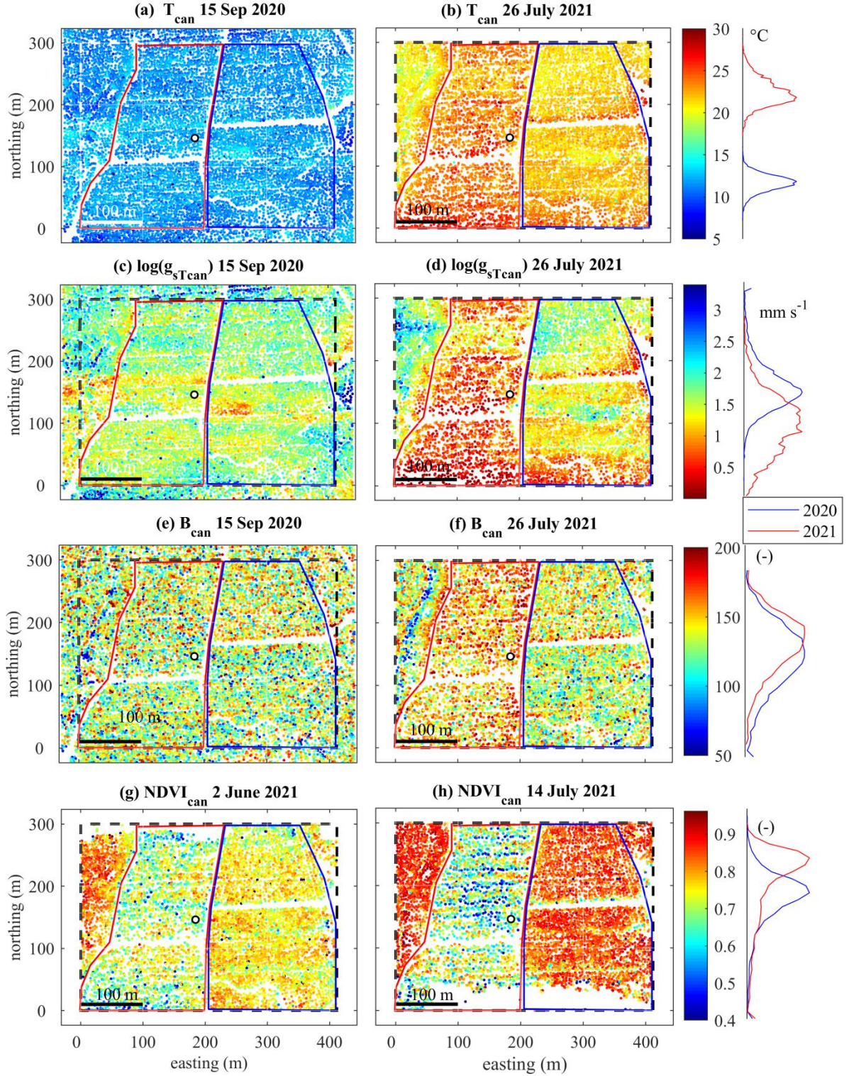
Figure 10. Spatial distributions of the tree-mean vegetation indices based on canopy temperature and multispectral imagery. (a,b) tree canopy temperature in the surveys of 15 September 2020 and 26 July 2021; (c,d) logarithm of temperature-derived stomatal conductance ( g_{sTcan} , dates as above); (e,f) canopy brightness (dates as above); (g,h) NDVI_{can} of the trees in pre-drought conditions (2 June 2021) and peak drought conditions (14 July 2021). The plots to the right of the main panels show the tree value distribution comparisons. The boundaries of the Harvest and Control blocks are shown as in Fig. 1. Note that the colour scale in (c,d) is
