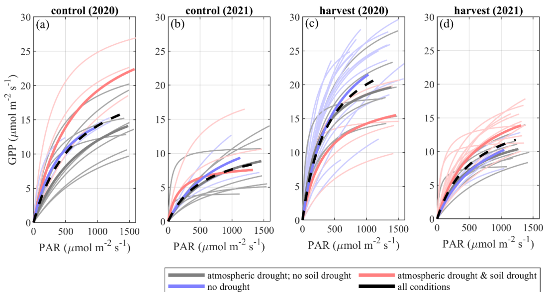
Figure 6. Light response curves for individual days in June-July of 2020 and 2021. (a) control, 2020; (b) control, 2021; (c) harvest, 2020; (d) harvest, 2021. The bold curves are the light response curves calculated from
