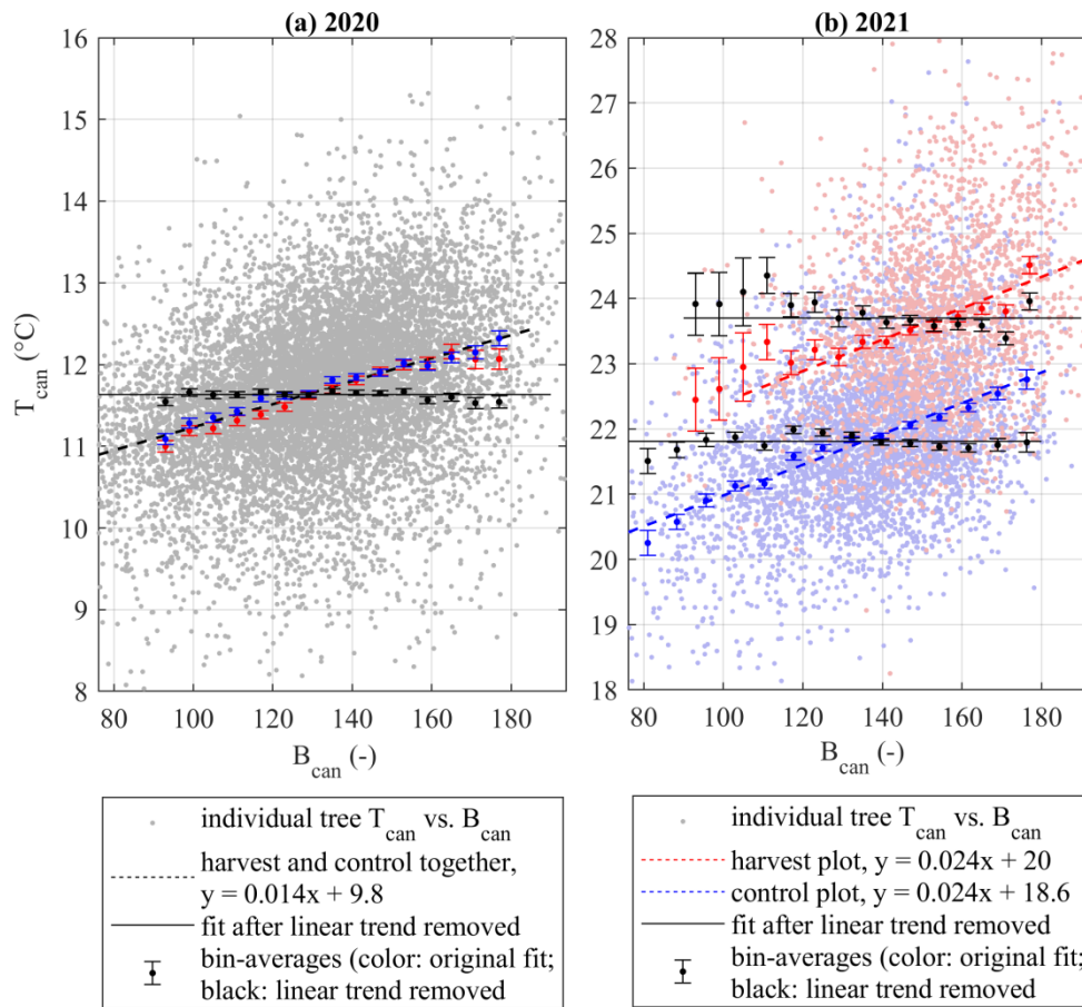
Figure G1. Individual tree canopy temperature versus canopy brightness for the UAV flight data of 15 Sep 2020 (a) and 26 July 2021 (b).
