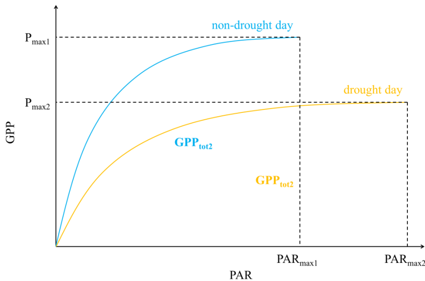
1170 Figure I1. Comparison of daily light response curves on a drought day (yellow) and non-drought day (cyan).
