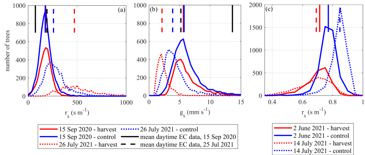
Figure 11. Distributions of individual canopy temperature-derived stomatal resistance r_{sTcan} (a), conductance g_{sTcan} (b) and NDVI_{can} (c). The mean EC-derived and median remotely sensed individual tree resistance and conductance values for the time of the respective UAV flights are shown with vertical lines. The presented EC-based values are the means for the time of the UAV flights.
