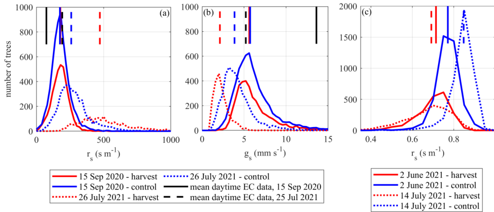
760 | Figure 11. Distributions of individual canopy temperature-derived stomatal resistance ( r_{sTcan} (a), and conductance g_{sTcan} (b) and NDVI can (c). The eddy covariance-mean EC-derived and median remotely sensed individual tree resistance and conductance values for the time of the respective UAV flights are shown as-with vertical lines. The presented EC-based values are the means for the time of the UAV flights.
