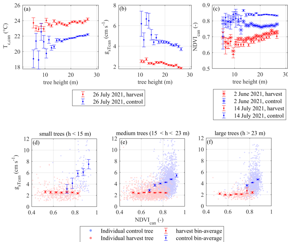
Figure 12. Tree indices plotted against tree height: (a) mean T_{c,can} canopy temperature T_{c,can} ; (b) corrected temperature-based stomatal conductance ( g_{sT} ). (d-f) temperature-based stomatal conductance vs. NDVI can shown separately for small (d), medium (e) and large (f) trees. In (a-c), the values are bin-averaged over 30 bins evenly distributed over the tree height range of [0..30], while in (d-f) 12 bins over the NDVI can range [0.4..1] are used.
