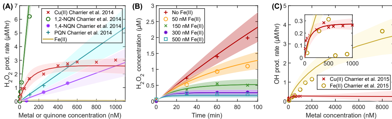
Figure 3. Production of reactive oxygen species in surrogate lung lining fluid. Production rate of H_2O_2 as a function of Cu(II), 1,2-NQN, 1,4-NQN, PQN (A), H_2O_2 concentration over time at different Fe concentrations (B), and OH production rate as a function of Cu(II) and Fe(II) (C). The markers are experimental data (for H_2O_2 (Charrier et al., 2014) and OH (Charrier and Anastasio, 2015)), and the lines depict the mean of the fit ensemble, while the shadings denote two standard deviations around the mean of the fit ensemble.
