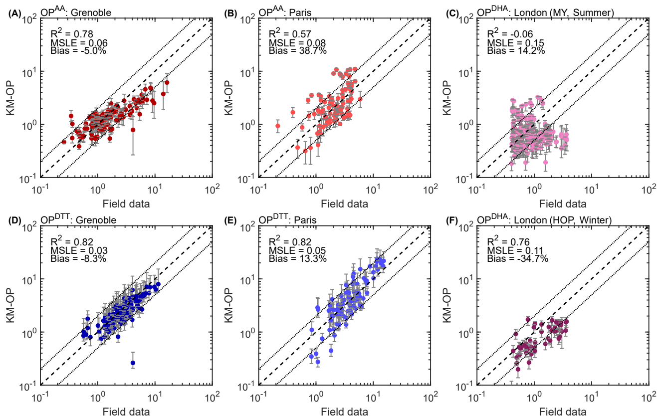
Figure 7. Correlation scatter plots of model-predicted and measured OP for particulate matter samples collected in three different sites across Europe: Grenoble (OP AA : panel A, and OP DTT : panel D), Paris (OP AA : panel B, and OP DTT : panel E), and OP DHA in London during the summer (C) and during the winter (F). Data shown in blue indicate OP DTT (in units of \text{nmol min}^{-1} \text{m}^{-3} ), while the red and pink data show OP AA (in units of \text{nmol min}^{-1} \text{m}^{-3} ) and OP DHA (in units of \text{nmol min}^{-1} \text{m}^{-3} ). The dashed lines indicate the 1:1 line. The dotted lines indicate the 2:1 and 1:2 lines. The error bars indicate the maximum and minimum values from the ensemble fits.
