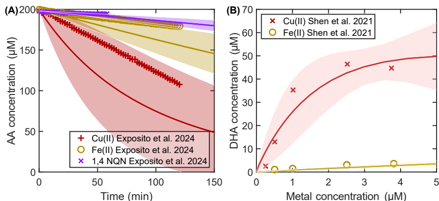
Figure 4. Ascorbic acid concentration as a function of time at different concentrations of 1,4-NQN, Fe(II) and Cu(II) ions (A). DHA concentration as a function of Fe(II) and Cu(II) concentration (B). The markers are measurement data points (Shen et al., 2021; Expósito et al., 2024), and the dark-colored lines depict the mean of the fit ensemble, while the shadings denote two standard deviations around the mean.
