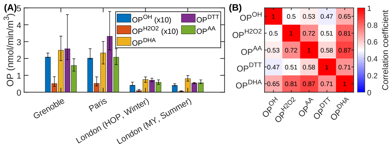
Figure 9. Comparison and correlation of different simulated OP assays. (A) Simulations of different OP assays explored in this study using average chemical composition data from measurements in Grenoble, Paris and London (Tab. 1). OP OH and OP H 2 O 2 results are multiplied by 10. (B) Pearson correlation matrix between intrinsic OP assays explored in this study using data from all study sites.
