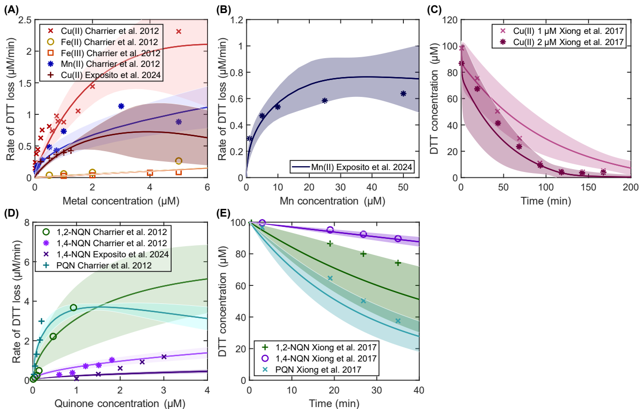
Figure 5. Rate of DTT loss as a function of different concentrations of transition metal ions (A and B) and quinones (D). DTT concentration as a function of time at different Cu(II) (C) and quinone (E) concentrations. The symbols are measurement data (Charrier and Anastasio, 2012; Xiong et al., 2017; Expósito et al., 2024), and the dark-colored lines depict the mean of fit ensembles from the model; shadings denote two standard deviations around the mean. The DTT concentration in Charrier and Anastasio (2012) and Xiong et al. (2017) data is 100 \mu\text{M} , while Expósito et al. (2024) use 50 \mu\text{M} of DTT.
