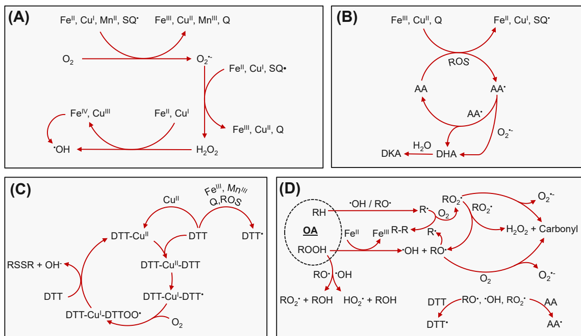
Figure 1. Chemical reaction mechanism used in KM-OP. TMIs, quinones, and Org can produce and convert ROS. Panel A shows the main reaction pathways for ROS formation and interconversion in the presence of TMIs and quinones. Panels B and C show the main reaction pathways for ascorbic acid and dithiothreitol oxidation through the reaction with ROS, TMIs, and quinones. Panel D shows the main reaction pathways for ROS formation and interconversion in the presence of organic aerosol.
