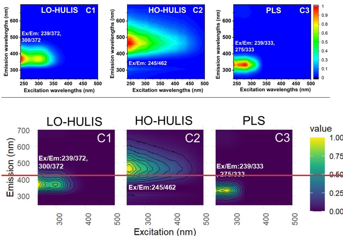
Figure 2. The three chromophores were identified by the PARAFAC model analysis of the excitation–emission spectra from all filter extracts collected from combustion of beech wood, straw, cow dung, and plastic.
