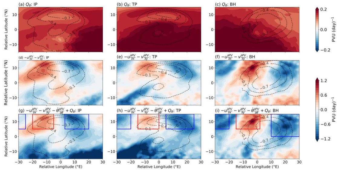
Figure S8. The same as Fig. S7, but for MERRA2.
