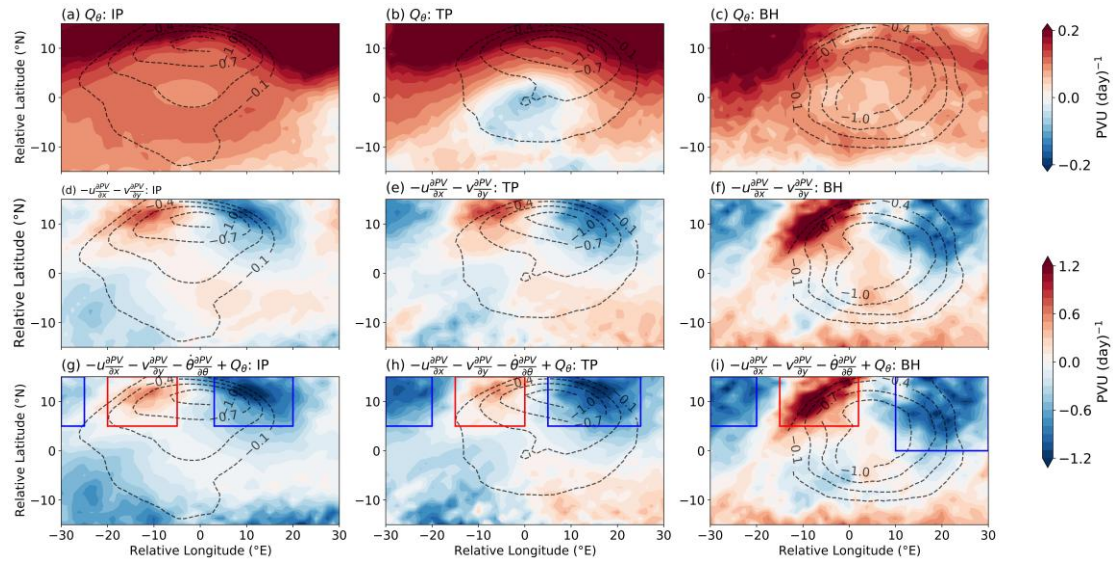
Figure S7. PV tendencies from ERA5 due to (a)-(c) the vertical divergence of diabatic heating, (d)-(f) horizontal advection, and (g)-(i) their sum along with vertical advection on the 370 K isentropic surface. Black dashed contours show PV anomalies at 370 K ranging from -1 to -0.1 PVU at an interval of 0.3 PVU. The horizontal and vertical axes indicate longitude and latitude relative to the vortex center, respectively. The red boxes in the lower row indicate the main areas of net positive PV tendencies, while the blue boxes indicate regions of net negative PV tendencies.
