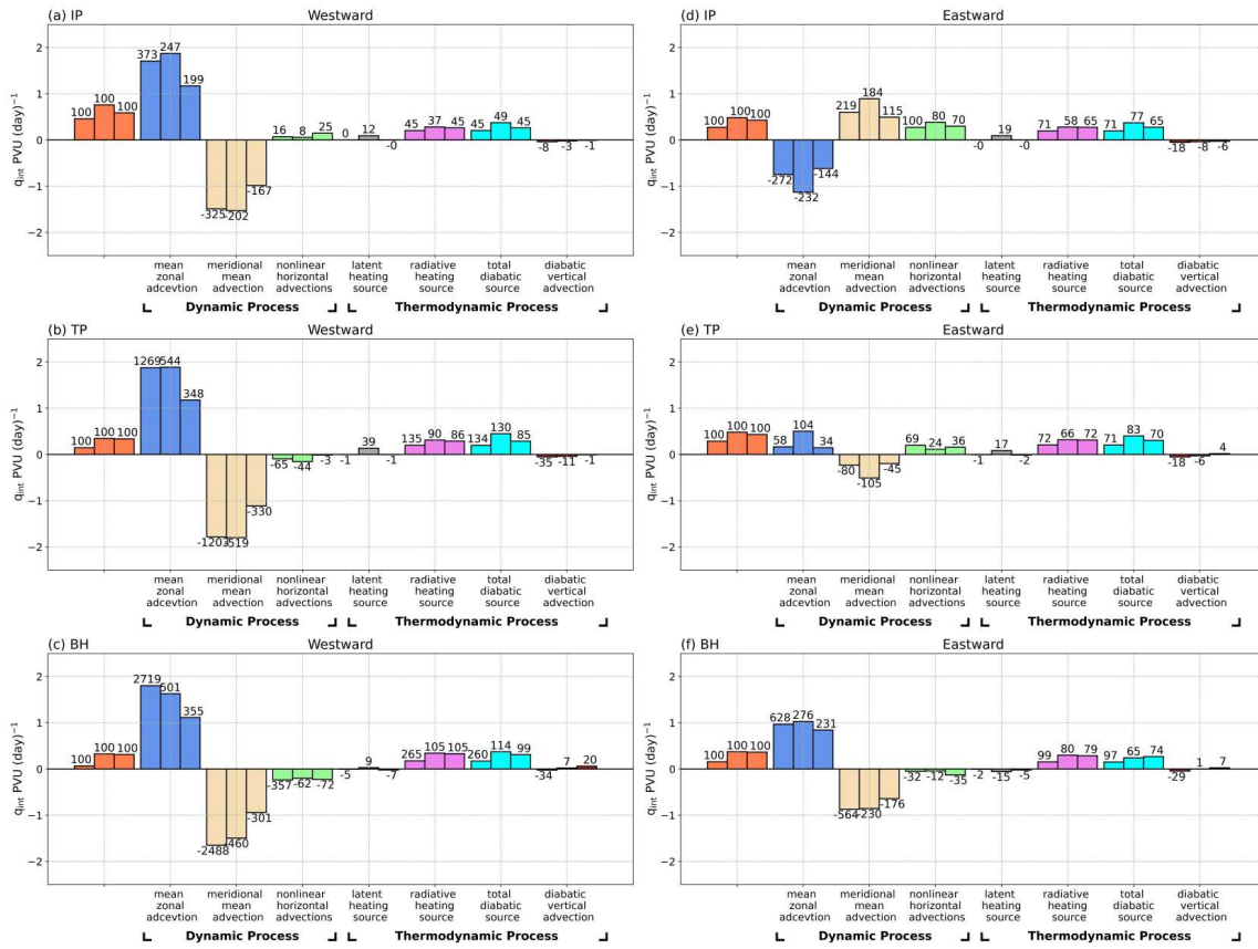
Figure 13. Contributions of dynamical and thermodynamic processes in Eq. (5) to mean PV tendencies to the (a–c) west of the vortex center and (d–f) east of the vortex center on the 370 K isentropic surface. From left to right, each group of three bars corresponds to JRA-3Q, ERA5, and MERRA-2. Numbers on bars denote the percentage contribution of each term. Terms include mean zonal advection, meridional mean advection, nonlinear horizontal advections, vertical advection, and the vertical divergence of latent, radiative, and diabatic heating. See section 3.2 for definitions.
