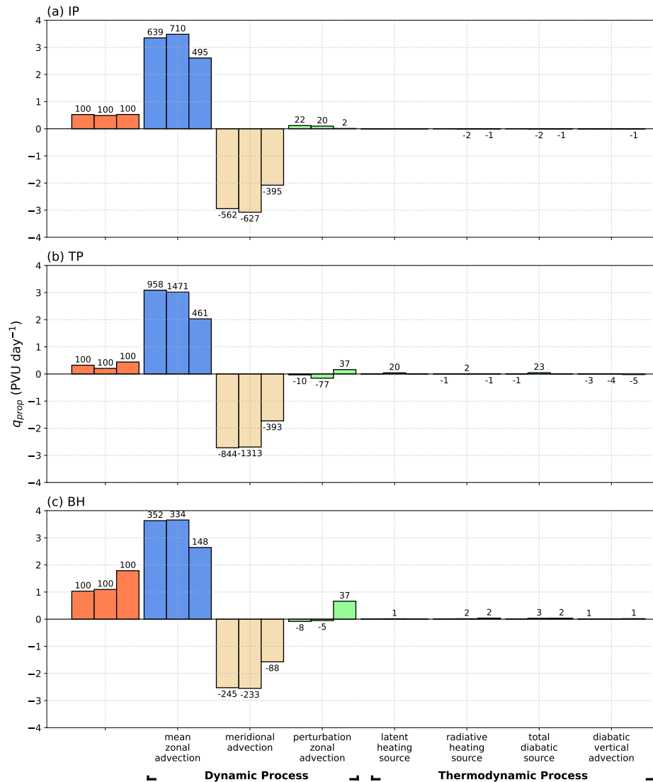
Figure 14. Relative As in Fig. 13, but for contributions (%) of dynamical and thermodynamic processes to the propagation-oriented PV tendency at 370 K during anticyclone intensification for tendencies in the northern dipole (a–e) westward propagation \dot{q}_{\text{PROP}} ; red and (d–f) blue boxes in Fig. 12g–i). Positive contributions indicate eastward propagation. Each group of three bars corresponds to JRA-3Q, ERA5, and MERRA-2 (left to right). Numbers on bars denote the percentage contribution of each term. Terms include mean zonal advection, mean meridional advection, nonlinear horizontal advection, vertical advection, and total diabatic heating.
