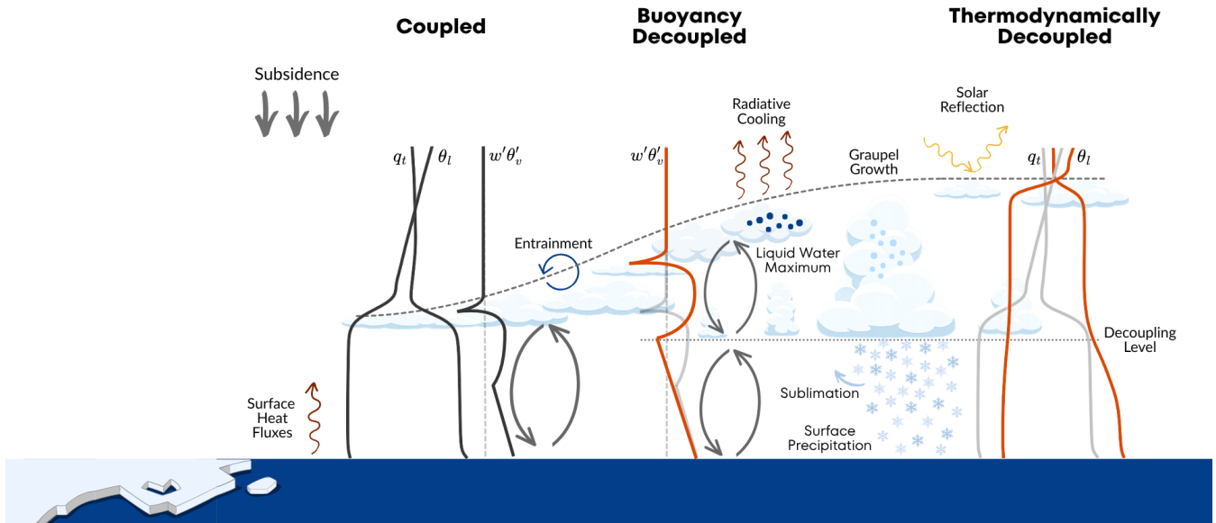
Figure 13. Conceptual evolution of the atmospheric boundary layer during the modelled Arctic marine cold air outbreak. Black and grey profiles of liquid water potential temperature \theta_l , total humidity q_t and buoyancy flux w'\theta'_v indicate a coupled boundary layer, whereas the orange profiles illustrate decoupling with respect to buoyancy-based ( w'\theta'_v ) and thermodynamic ( \theta_l , q_t ). The top of the boundary layer is indicated as a dashed line.
