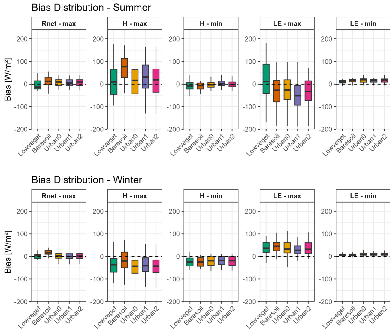
555 Figure 4: Distribution of mean bias in simulated daily maximum and minimum surface energy fluxes (sensible heat H, latent heat LE, and maximum net radiation Rnet) during summer (first row) and winter (second row) months (DJF/JJA based on hemisphere) across the 20 urban sites. For each boxplot, the central horizontal line indicates the median, the lower and upper edges of the box indicate the 25th and 75th percentiles, respectively, and the whiskers extend to the most extreme values within 1.5 times the interquartile range (IQR). The dashed horizontal line indicates zero bias.
