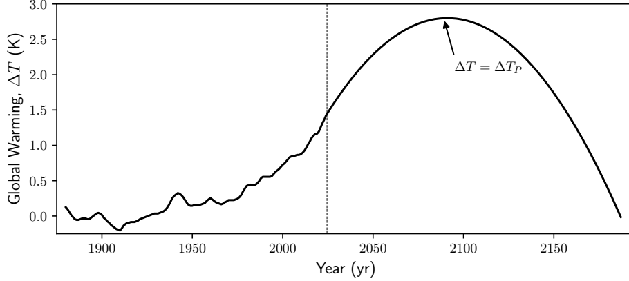
Figure 3. Historical record of global warming up to the year 2024, normalised so that the average of the first 21 years (1880 to 1900 inclusive) is zero. From the year 2024 onwards, a quadratic “overshoot” profile is derived, corresponding to setting an upper level of global warming of \Delta T_P = 2.8 K (as annotated). The vertical dotted line marks the year 2024. The future scenario is designed to transition smoothly from the historical measurement record in the year 2024.
