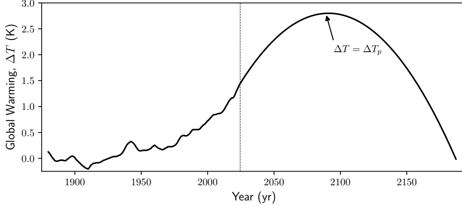
Figure 3. Historical record of global warming up to the year 2024, normalised so that the average of the first twenty years (1880 to 1899 inclusive) is zero. From the year 2024 onwards, a quadratic “overshoot” profile is derived, corresponding to setting an upper level of global warming of \Delta T_P = 2.8 K (as annotated). The vertical dotted line marks the year 2024. The future scenario is designed to transition smoothly from the historical measurement record in the year 2024.
