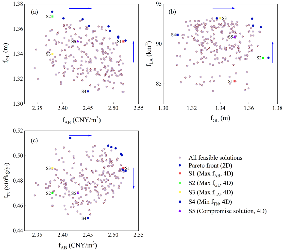
Figure 6. Scatter plots for optimization in a dry year exhibiting the correlation between each pair of objectives, (a) f_{AB} and f_{GL} ; (b) f_{GL} and f_{LA} ; and (c) f_{AB} and f_{TN} . Each dot represents a feasible solution. The representative solutions for dry scenario (S1-S5) can be identified by rectangles with different color. The navy-blue arrow indicates the direction of Pareto optimality.
