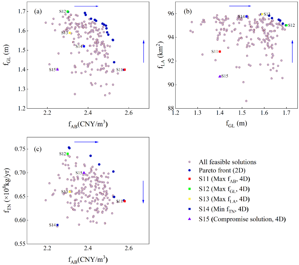
445 Figure 8. Scatter diagrams depicting correlations among objective pairs under a wet year, (a) f_{AB} and f_{GL} ; (b) f_{GL} and f_{LA} ; and (c) f_{AB} and f_{TN} . Representative wet-year solutions (S11-S15) are marked using colored rectangles.
