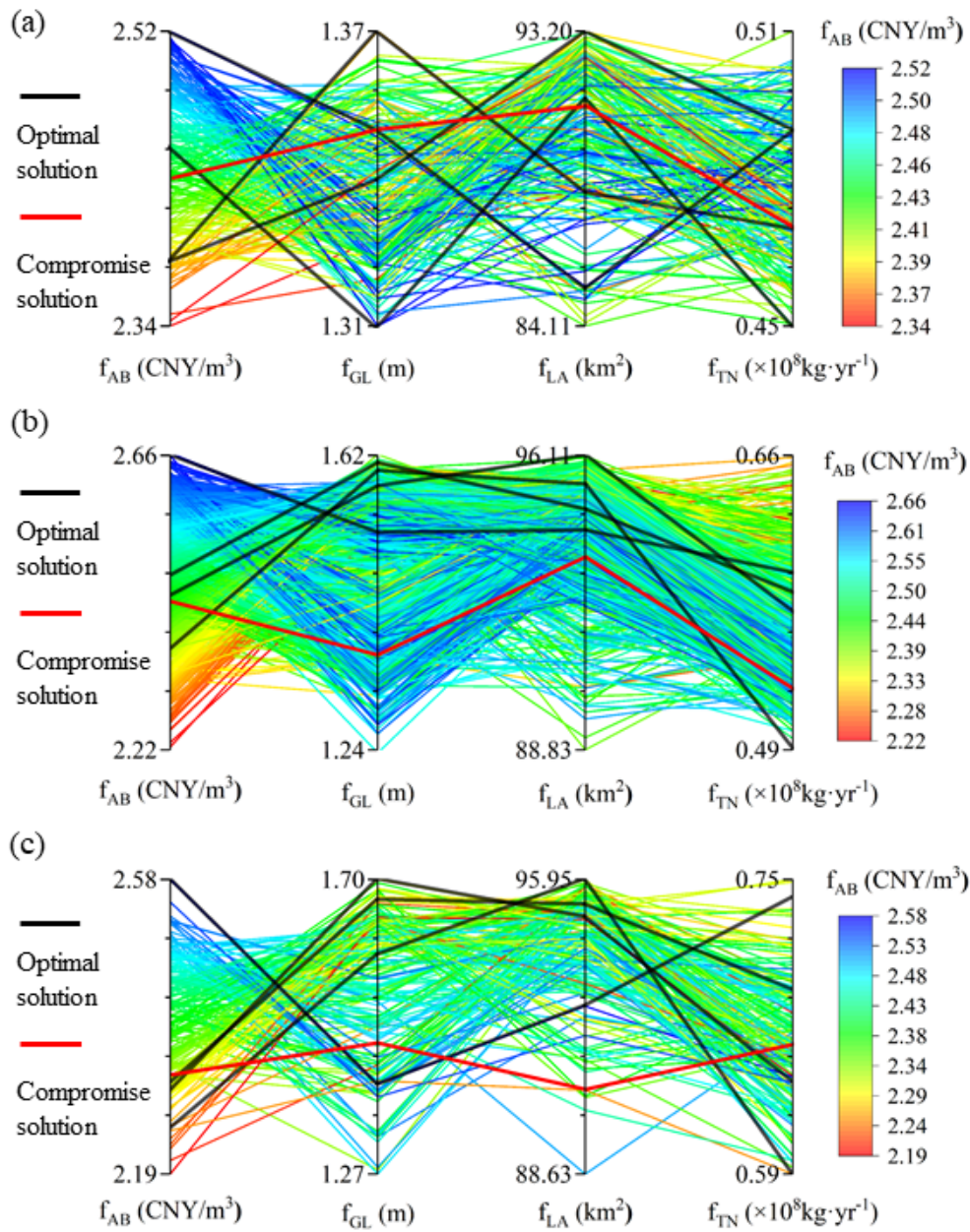
Figure 5. Objective values (y axis) plotted against management objectives f_{AB} , f_{GL} , f_{LA} and f_{TN} , with panels (a, b, c) representing dry, normal, and wet years, respectively.
