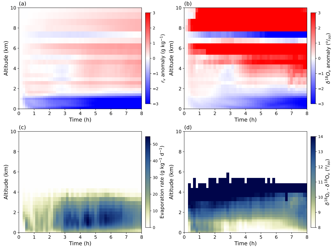
Figure 4. Evolution of some vertical profiles along the course of the simulation: (a) water vapor mixing ratio ( r_v , \text{g kg}^{-1} ) anomaly with respect to the initial vertical profile, (b) isotopic composition of water vapor ( \delta^{18}\text{O}_v , ‰) anomaly with respect to the initial vertical profile, (c) rain evaporation rate ( \text{g kg}^{-1} \text{ day}^{-1} ), (d) difference between the isotopic composition of rain and that of the water vapor ( \delta^{18}\text{O}_r - \delta^{18}\text{O}_v ).
