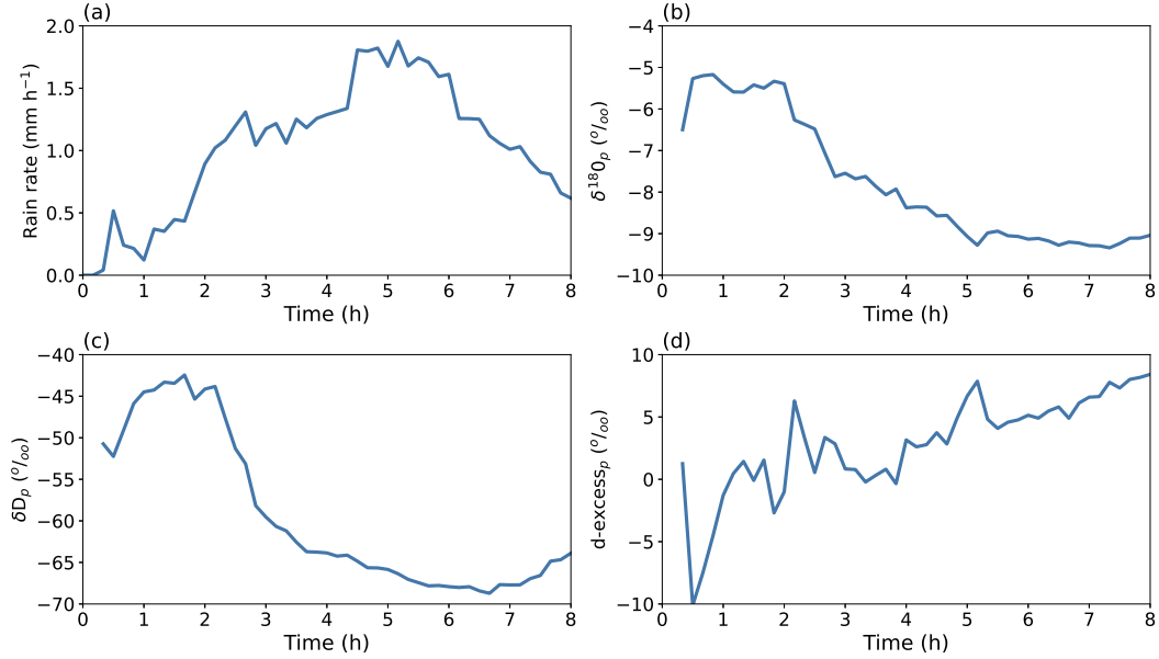
Figure 2. Temporal evolution of (a) the instantaneous surface rain rate ( \text{mm h}^{-1} ), and the isotopic composition of the rain (‰): (b) \delta^{18}\text{O} , (c) \delta\text{D} and (d) d-excess. Variables are averaged over the whole domain every 10 min.
