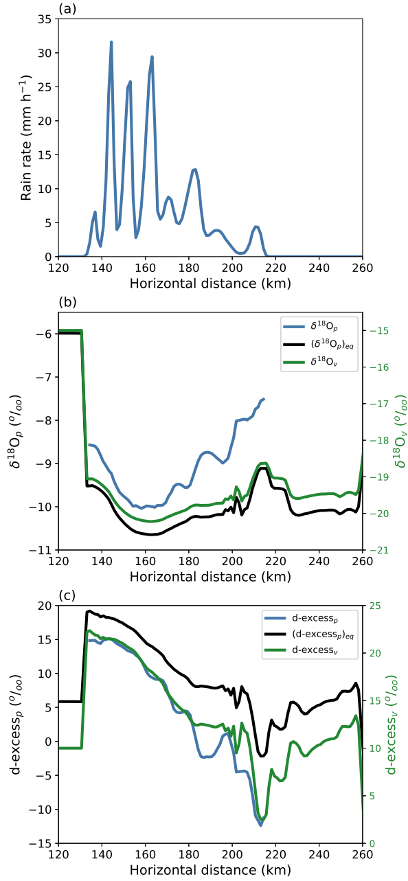
Figure 8. Evolution of the surface rain rate (a), \delta^{18}\text{O} (b), and d-excess (c) along the x-direction after 6 hours of simulation. In (b) and (c), the blue, black and green lines correspond to the isotopic composition of rain, rain in isotopic equilibrium with water vapor, and water vapor, respectively. In (b) and (c), the isotopic composition of rain (water vapor) is on the left-y (right-y) axis.
