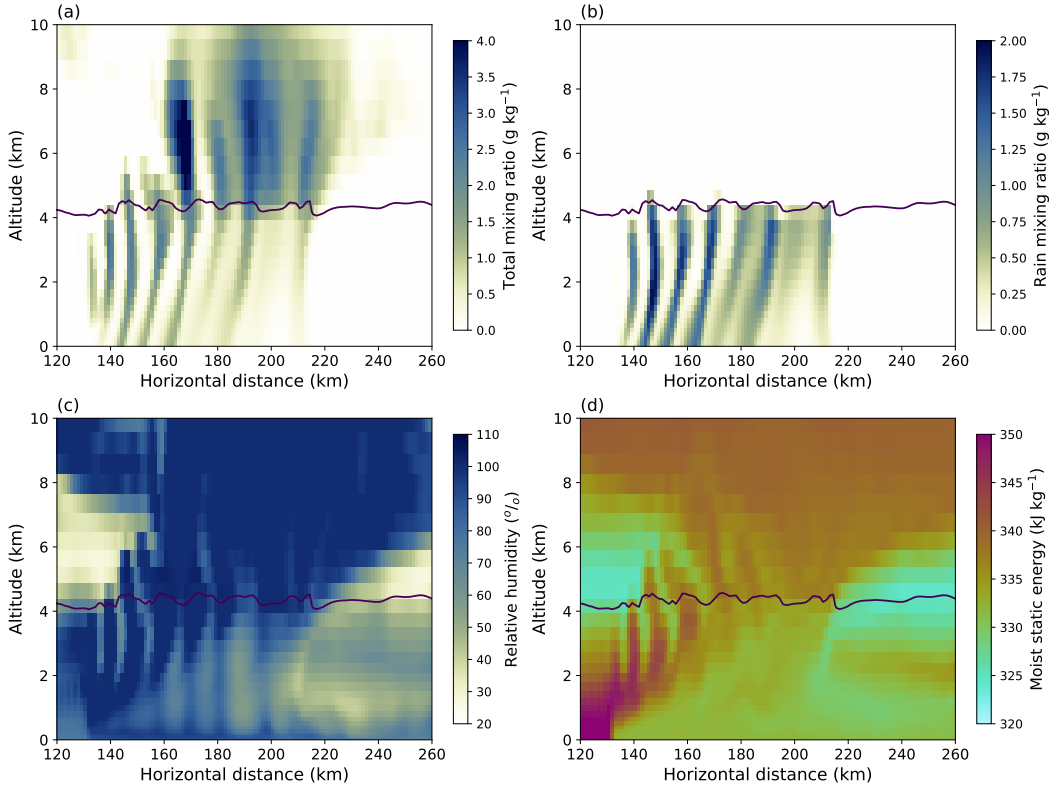
Figure 5. Vertical cross section of the (a) total condensed water mixing ratio ( \text{g kg}^{-1} ), (b) rain mixing ratio ( \text{g kg}^{-1} ), (c) relative humidity (%) and (d) moist static energy ( \text{kJ kg}^{-1} ) after 6 hours. The total water condensed mixing ratio is the sum of the mixing ratio of all hydrometeors (cloud droplets, rain, cloud ice, snow/aggregates and graupel). The relative humidity is calculated for saturation over water for temperatures over 0^\circ\text{C} , and for saturation over ice for temperatures below 0^\circ\text{C} . The black line corresponds to the 0^\circ\text{C} isotherm.
