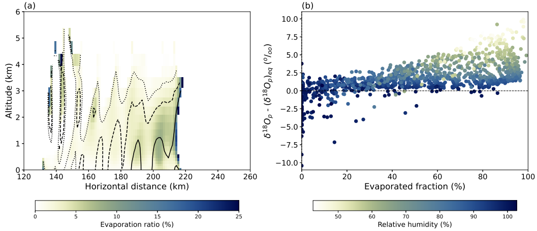
Figure 10. (a) Vertical cross section of the fraction of rain that evaporates (colors; %) at after 6 hours of simulation. The dotted, dashed and solid lines show respectively the 30%, 60 % and 90% isolines of vertically integrated evaporated fraction ( f_{\text{EVA}} ). The estimate of the vertically integrated evaporated fraction assumes a drop fall velocity of 20 \text{ km h}^{-1} . Similar results are obtained for a lower ( 10 \text{ km h}^{-1} ) and a higher ( 30 \text{ km h}^{-1} ) drop fall velocity. (b) Scatter plot of the isotopic disequilibrium ( \delta^{18}\text{O}_p - (\delta^{18}\text{O}_p)_{\text{eq}} ) as a function of the vertically integrated evaporated fraction ( f_{\text{EVA}} ), for all x-values and altitudes where rain occurs. Markers are colored by relative humidity (%).
