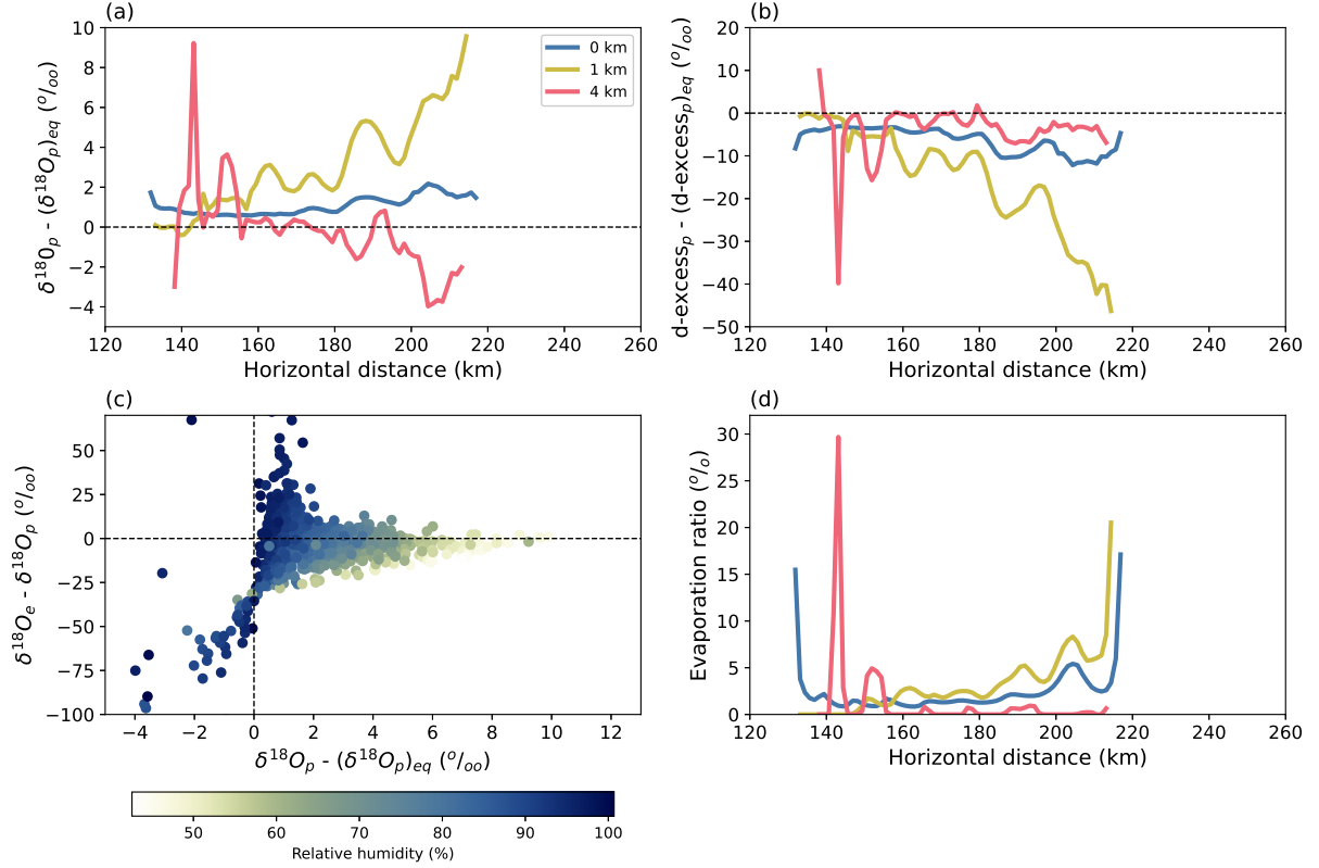
Figure 9. Difference between the isotopic composition of the rain and of the rain at isotopic equilibrium with the vapor at different altitudes for \delta^{18}\text{O} (a) and d-excess (b) along the x-direction after 6 hours of simulation. (c) Scatter plot of the difference between the \delta^{18}\text{O} in the evaporation flux and in the rain ( \delta^{18}\text{O}_e - \delta^{18}\text{O}_p ), as a function of the \delta^{18}\text{O} in the rain and in the vapor at isotopic equilibrium ( \delta^{18}\text{O}_p - (\delta^{18}\text{O}_p)_{eq} ), for all x-values and altitudes where rain occurs. Markers are colored by relative humidity. (d) Fraction of rain that evaporates along the x-direction after 6 hours of simulation at different altitudes. The blue, golden and red lines correspond to the isotopic composition at the surface, 1 km altitude and 4 km altitude, respectively.
