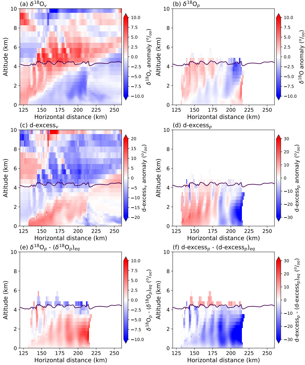
Figure 7. Vertical cross section after 6 hours of (a) \delta^{18}\text{O}_v , (b) \delta^{18}\text{O}_p , (c) \text{d-excess}_v , (d) \text{d-excess}_p , (e) \delta^{18}\text{O}_p - (\delta^{18}\text{O}_p)_{eq} and (f) \text{d-excess}_p - (\text{d-excess}_p)_{eq} . Panels (a) to (d) are anomalies calculated by subtracting the average value of the variable at a given altitude from the local value of the variable. The black line corresponds to the 0^\circ\text{C} isotherm. Similar panels with absolute values can be seen on Fig. S1.
