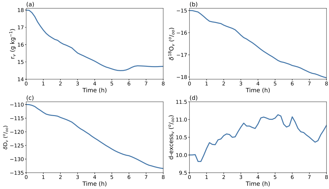
Figure 3. Temporal evolution of (a) the near-surface water vapor mixing ratio ( \text{g kg}^{-1} ), and the isotopic composition of water vapor (‰): (b) \delta^{18}\text{O} , (c) \delta\text{D} and (d) d-excess. Variables are averaged over the whole domain every 10 min.
