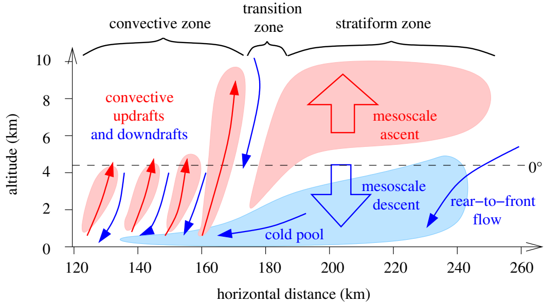
Figure 6. Schematic of the main structural components of a squall line moving from right to left with the three convective, transition and stratiform zones along with horizontal and vertical dynamic.
