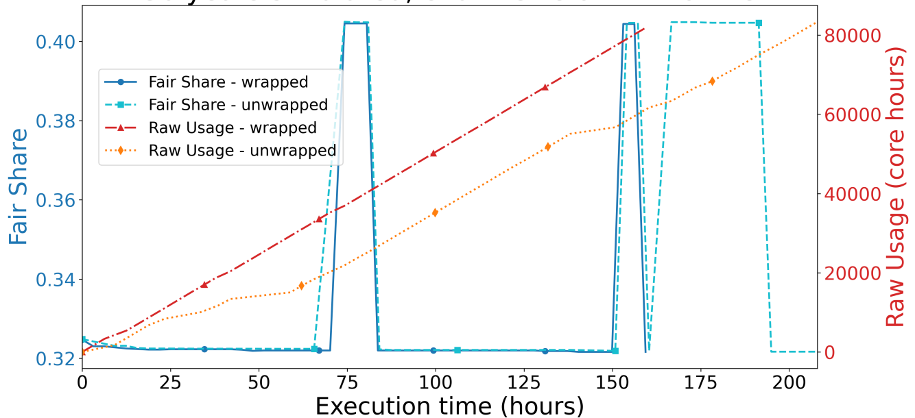
Figure 4. Fair Share and Raw Usage of Auto-EC-Earth3 50 years simulated with the T255L91-ORCA1L75-LIM3-PISCES-LPJG-TM5 configuration. 50 years simulated with a chunk size of 12 months. Results for MareNostrum 4.
