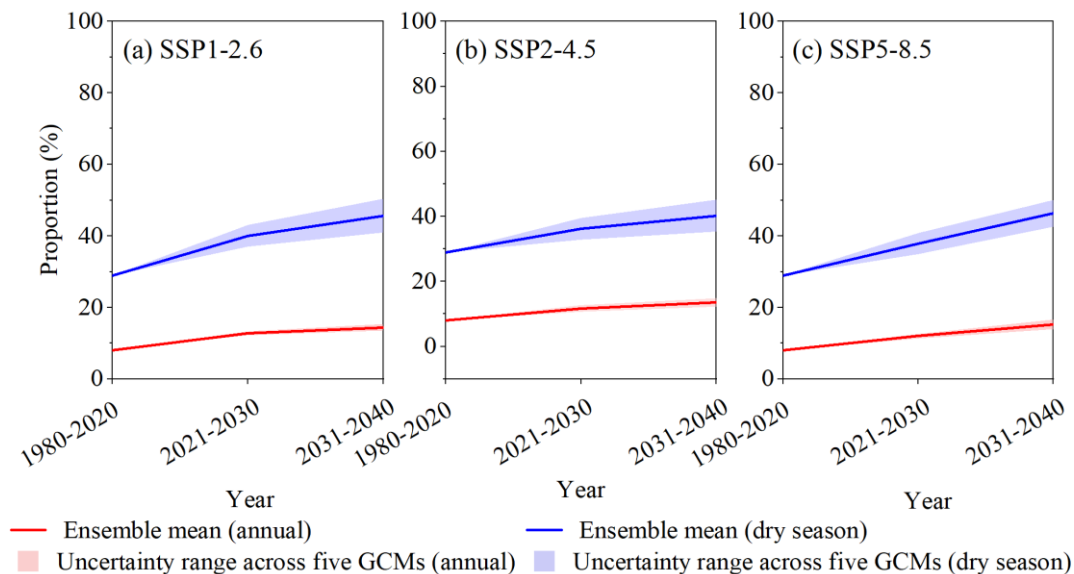
325 Figure 6 Ratios of irrigation water withdrawal to available water under three climate scenarios of the basin: (a) SSP1–2.6, (b) SSP2–4.5, and (c) SSP5–8.5. The ratios are calculated for the historical baseline period 1980–2020 and two future periods 2021–2030 and
