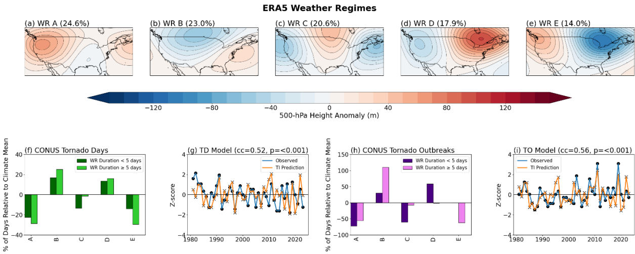
Figure 1: 500H anomaly patterns of WRs A-E with long-term frequency indicated in panel title (a-e). ERA5 tornado day (f) and tornado outbreak (h) CONUS probability anomalies for persistent ( \geq 5 days; light green, pink) and nonpersistent ( < 5 days; dark green, indigo) WRs. Time series of standardized tornado days (g) and tornado outbreak days (i) from the observation (blue) and estimation of the empirical modeling (red). Spearman rank correlation and p-value are indicated in panels g and i.
