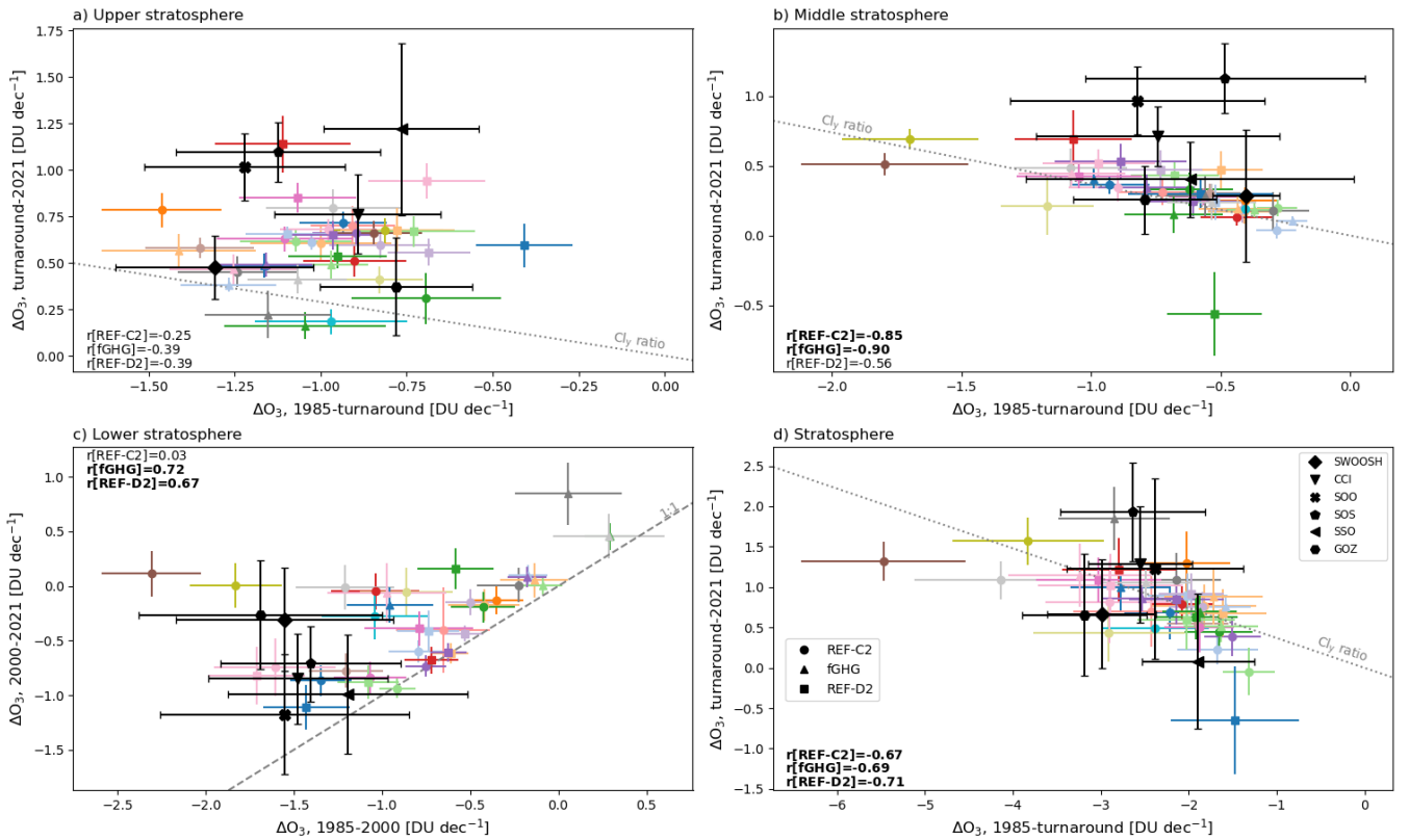
Figure 9. Scatter plots of the tropical partial column ozone depletion (horizontal axes) and early recovery (vertical axes) trends from models and observations. Each model marker shows the DLM-inferred trend from a single model realization, with different symbols for different model experiments (see legend) and different colors for each model (see legends in Figs. 4 and 6). Horizontal and vertical error bars indicate \pm 1 standard deviation about the mean DLM change, as in previous figures. The inter-model correlation coefficients for each multi-model experiment are shown in each panel (significant correlations are in bold). The dotted gray lines in (a,b,d) show the multi-model mean value of the Cl_2 recovery/depletion trend ratio calculated over the same latitude ( 30^\circ S– 30^\circ N) and vertical region from the REF-C2 experiment. The dashed gray line in (c) is the 1:1 line, indicating values for which the LS PCO trends are the same both before and after 2000.
