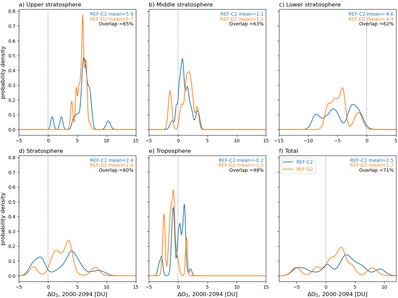
538 Figure 7: Kernel density estimates (KDEs) of DLM-based tropical ozone column change over 2000–2094 from REF-C2 (blue) and 539 REF-D2 (orange) model simulations. The multi-model mean changes and overlap between the two experiments are indicated in each 540 panel. 541 542
