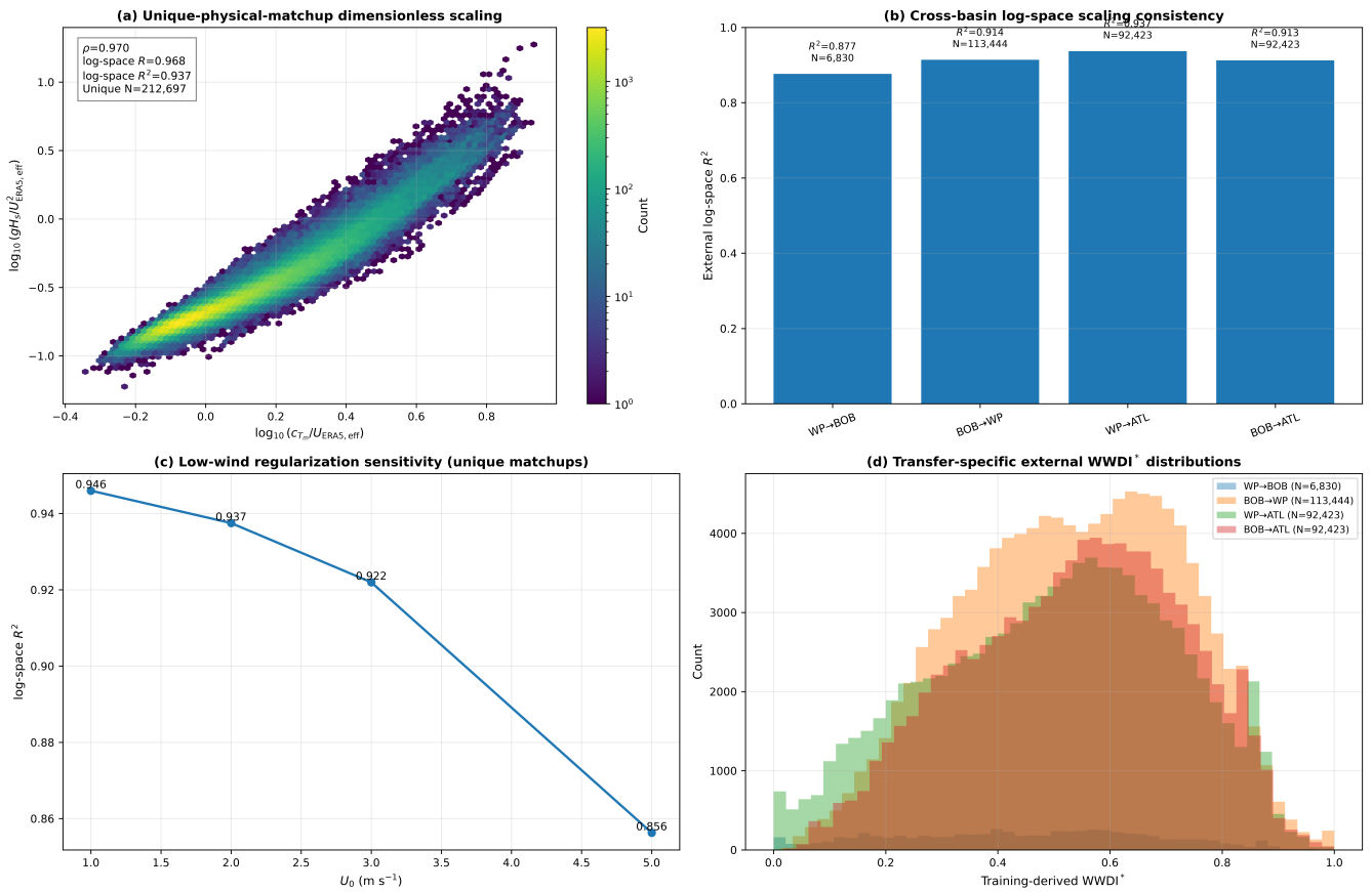
Figure 3. Dimensionless wave scaling and low-wind regularization diagnostics. Panel (a) shows the log-space relationship between effective wave age A_w = c_{T_m}/U_{ERA5,eff} and dimensionless wave height H_w^* = gH_s/U_{ERA5,eff}^2 . Panel (b) shows cross-basin consistency of the training-derived log-space scaling. Panel (c) summarizes sensitivity to the low-wind regularization parameter U_0 , and panel (d) shows external distributions of the frozen training-derived WWDI* formulations.
