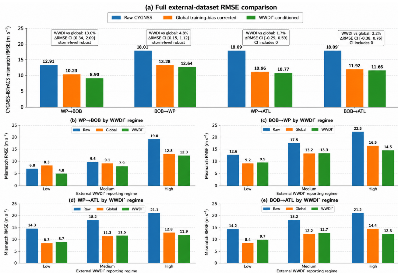
Figure 13. Training-only diagnostic mismatch adjustment under strict cross-basin transfer. Panel (a) compares external RMSE for the raw CYGNSS–IBTrACS mismatch, the global training-bias correction, and the WWDI*-conditioned adjustment. Panels (b–e) summarize performance across low-, medium-, and high-WWDI* external reporting regimes. The global correction uses a single mean signed mismatch estimated from the training basin, whereas the WWDI* adjustment uses mean signed mismatch within 10 training-defined WWDI* quantile bins. All calibration quantities are frozen before external evaluation. The low-, medium-, and high-WWDI* categories are used only for visualization and reporting and do not define the adjustment itself.
