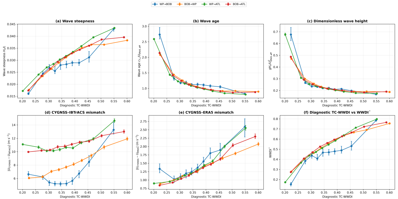
Figure 4. Physical regime behaviour of diagnostic TC-WWDI across the four strict external-transfer experiments. Panels show the regime evolution of (a) wave steepness, (b) wave age, (c) dimensionless wave height, (d) absolute CYGNSS–IBTrACS mismatch, (e) absolute CYGNSS–ERA5 mismatch, and (f) WWDI*. Each transfer is evaluated independently. Points denote quantile-bin medians, and error bars represent asymmetric distribution-free 95 % confidence intervals for the median.
