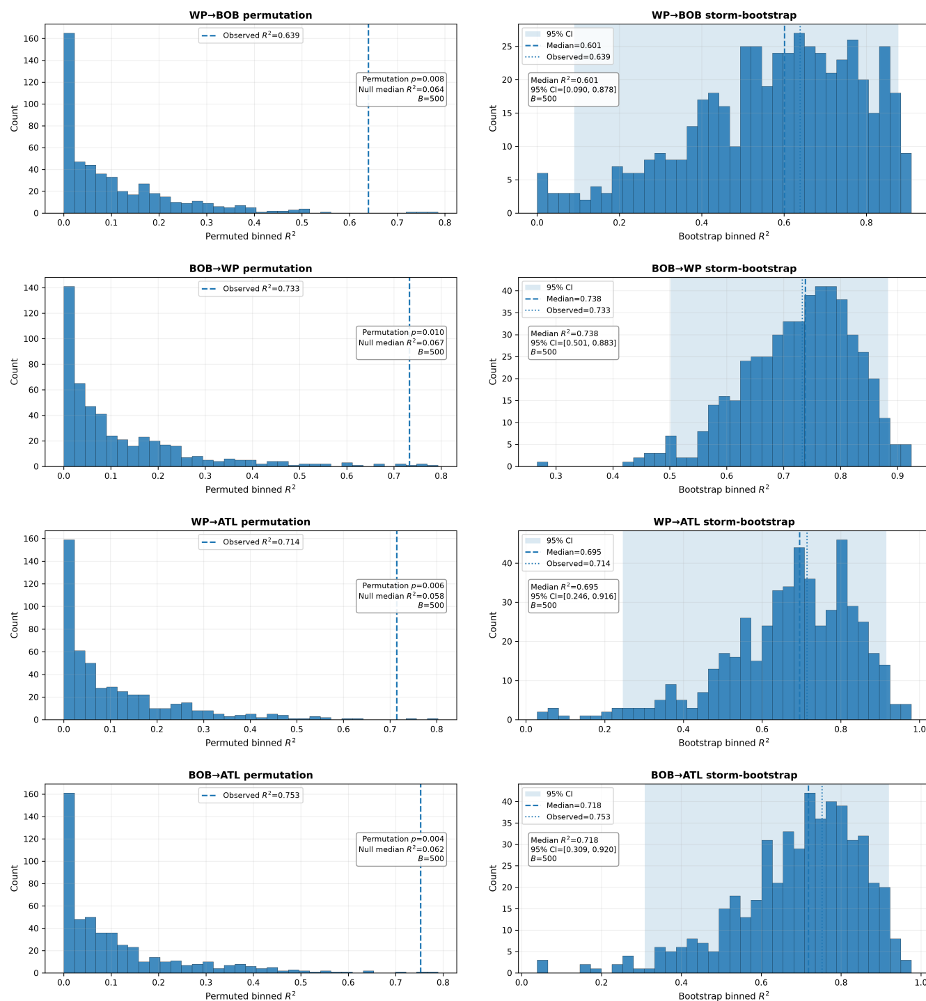
Figure 8. Permutation and storm-wise bootstrap assessment of the external WWDI* regime relationships. Left-column panels show null distributions of the 10-bin R^2 obtained from 500 random permutations, with the observed external value marked for comparison. Right-column panels show the corresponding distributions from 500 storm-wise bootstrap resamples together with the bootstrap median, observed R^2 , and 95 % percentile interval.
