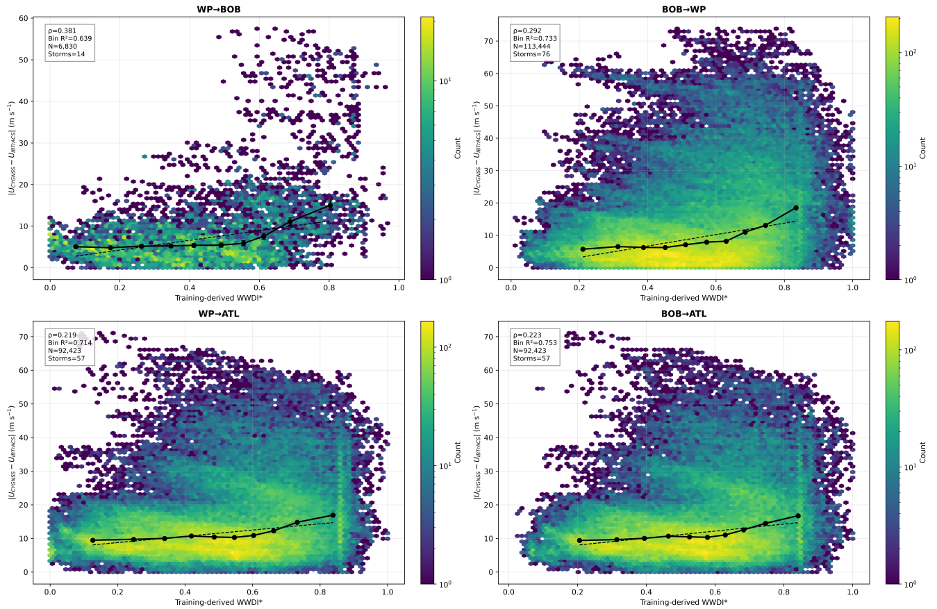
Figure 5. Strict cross-basin external evaluation of WWDI*. Each panel shows the relationship between the frozen training-derived WWDI* and absolute CYGNSS-IBTrACS mismatch. Background density represents individual external observations, while the overlaid points show the 10-bin regime-scale response.
