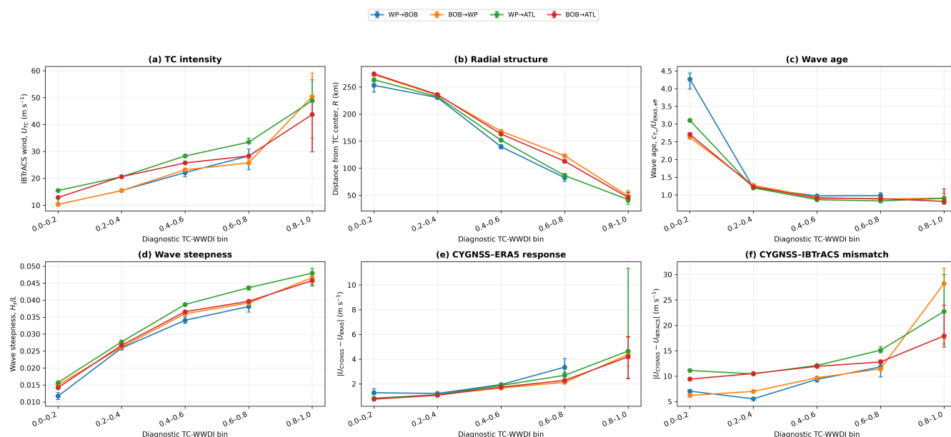
Figure 11. Physical regime transition across fixed diagnostic TC-WWDI intervals. Points denote bin medians, and error bars represent asymmetric distribution-free 95 % confidence intervals for the median. Each strict transfer experiment is shown independently.
