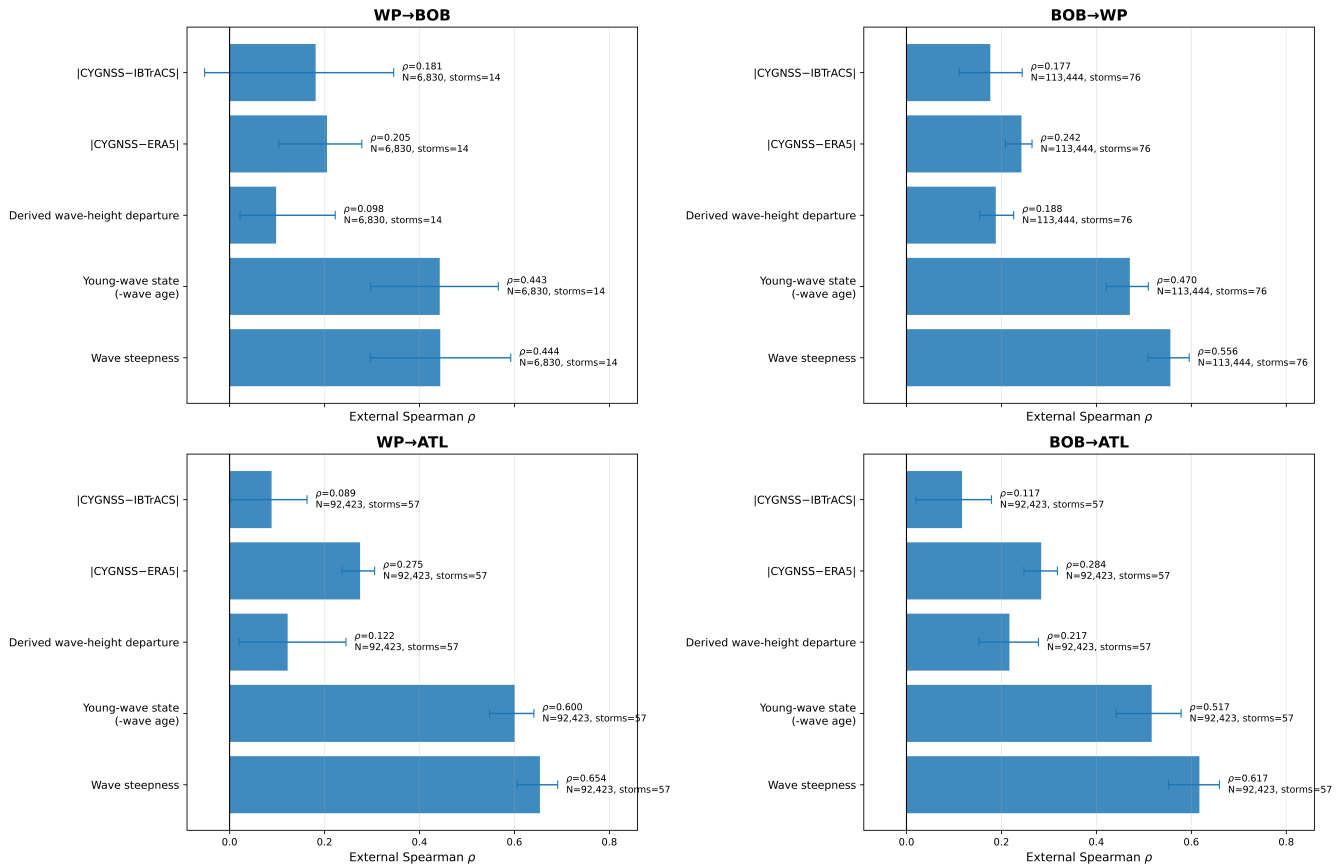
Figure 7. Cross-basin consistency of the external physical relationships. Bars show Spearman rank associations for the two reference-relative CYGNSS mismatch measures and the principal wind–wave descriptors under each strict external-transfer configuration. Wave steepness and young-wave state show the most persistent cross-basin structure, whereas the derived wave-height-departure term exhibits weaker and more transfer-dependent behaviour. Each transfer is evaluated independently.
