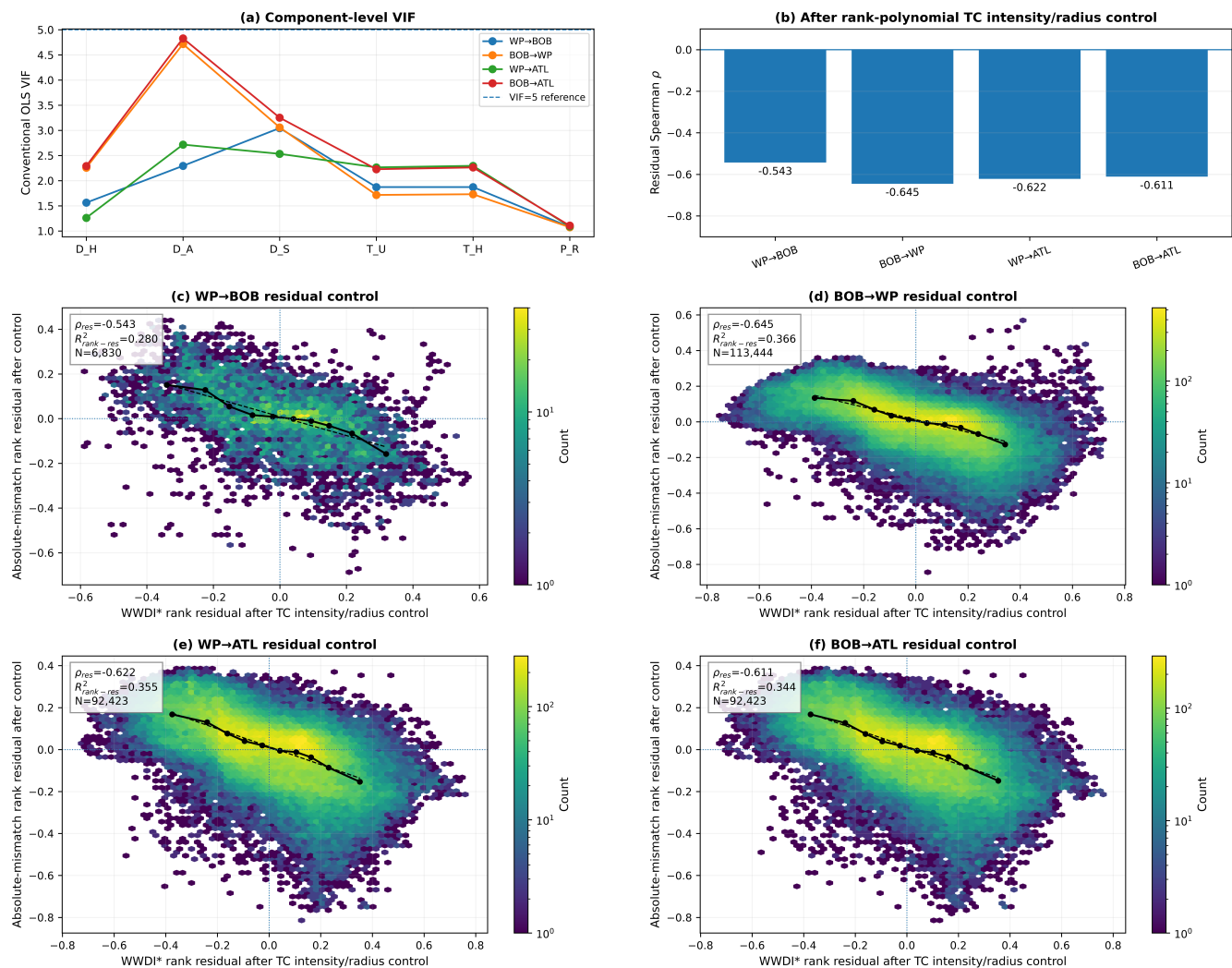
Figure 6. Confounder-aware diagnostic analysis across the four strict external-transfer experiments. Panel (a) shows conventional OLS variance-inflation factors for the six normalized candidate components. Panel (b) shows the residual Spearman association between WWDI* and E_{TC} after controlling for ranked TC intensity, ranked storm-relative radius, their quadratic terms, and their interaction. Panels (c–f) show the corresponding rank-residual relationships. Negative conditional associations persist in all four transfers and are interpreted as conditional diagnostics rather than causal effects.
