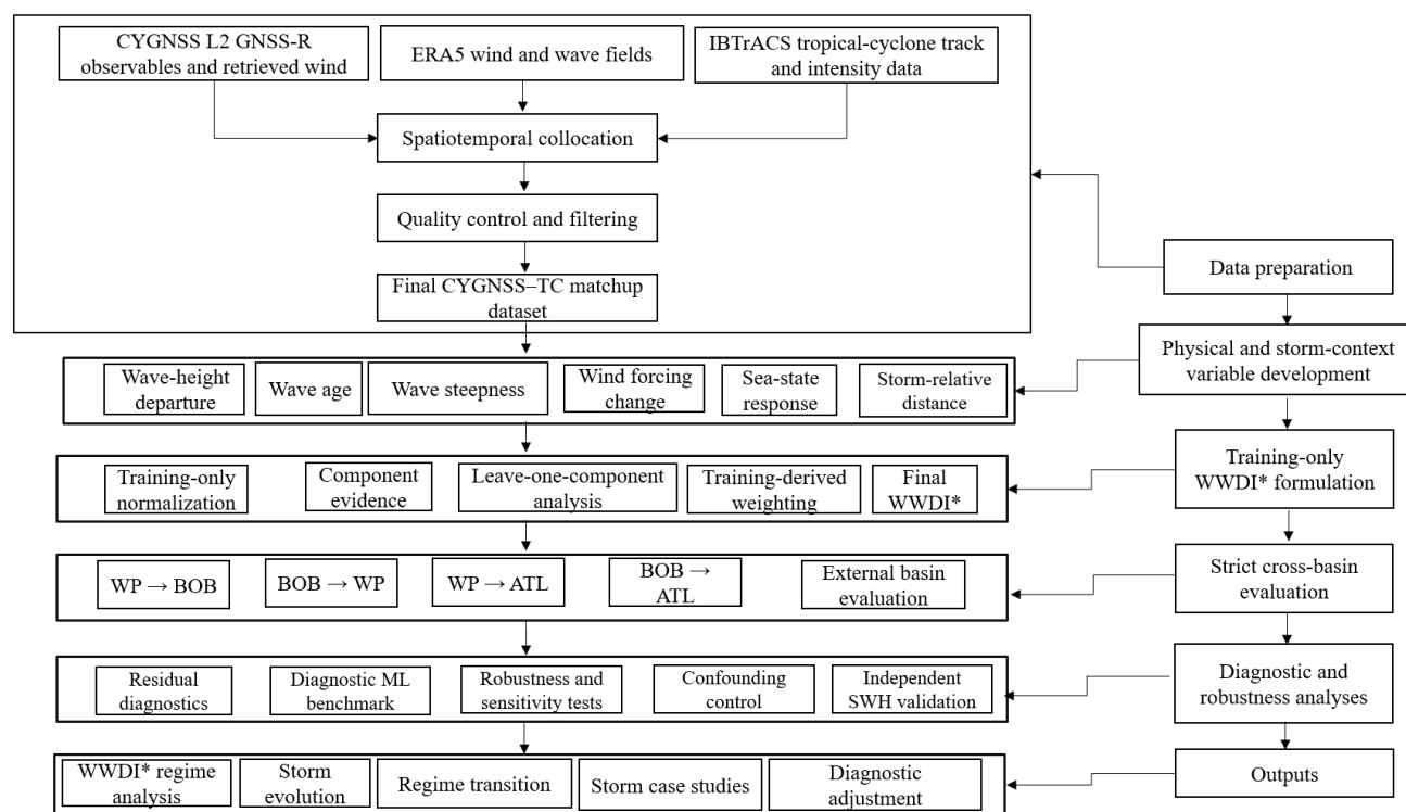
Figure 2. Methodological workflow of the physics-guided tropical-cyclone wind-wave disequilibrium framework. CYGNSS observations are combined with ERA5 atmospheric and wave fields and IBTrACS tropical-cyclone information. Physical and storm-context descriptors are derived from the collocated observations and normalized using training-only statistics. The complete component set is first examined through the equal-weight diagnostic TC-WWDI, after which the supervised WWDI* formulation is constructed from training-derived evidence weights. Evaluation comprises strict temporal and cross-basin transfer, confounder and multicollinearity diagnostics, permutation testing, storm-wise bootstrap resampling, sensitivity analysis, independent ERA5–CMEMS wave validation, diagnostic machine-learning experiments, and training-calibrated mismatch adjustment.
