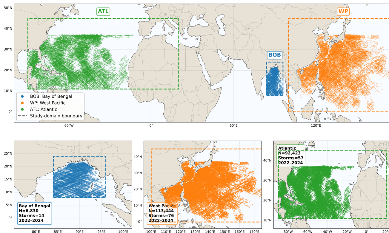
Figure 1. Study regions and spatial distribution of the final unique CYGNSS–tropical-cyclone matchups. The Bay of Bengal (BOB), western North Pacific (WP), and North Atlantic (ATL) domains are shown together with the retained CYGNSS specular-point locations. The final multi-basin dataset contains 212,697 unique physical matchups associated with 147 tropical cyclones during 2022–2024. Geographic base-map features are obtained from Natural Earth and rendered using Cartopy.
