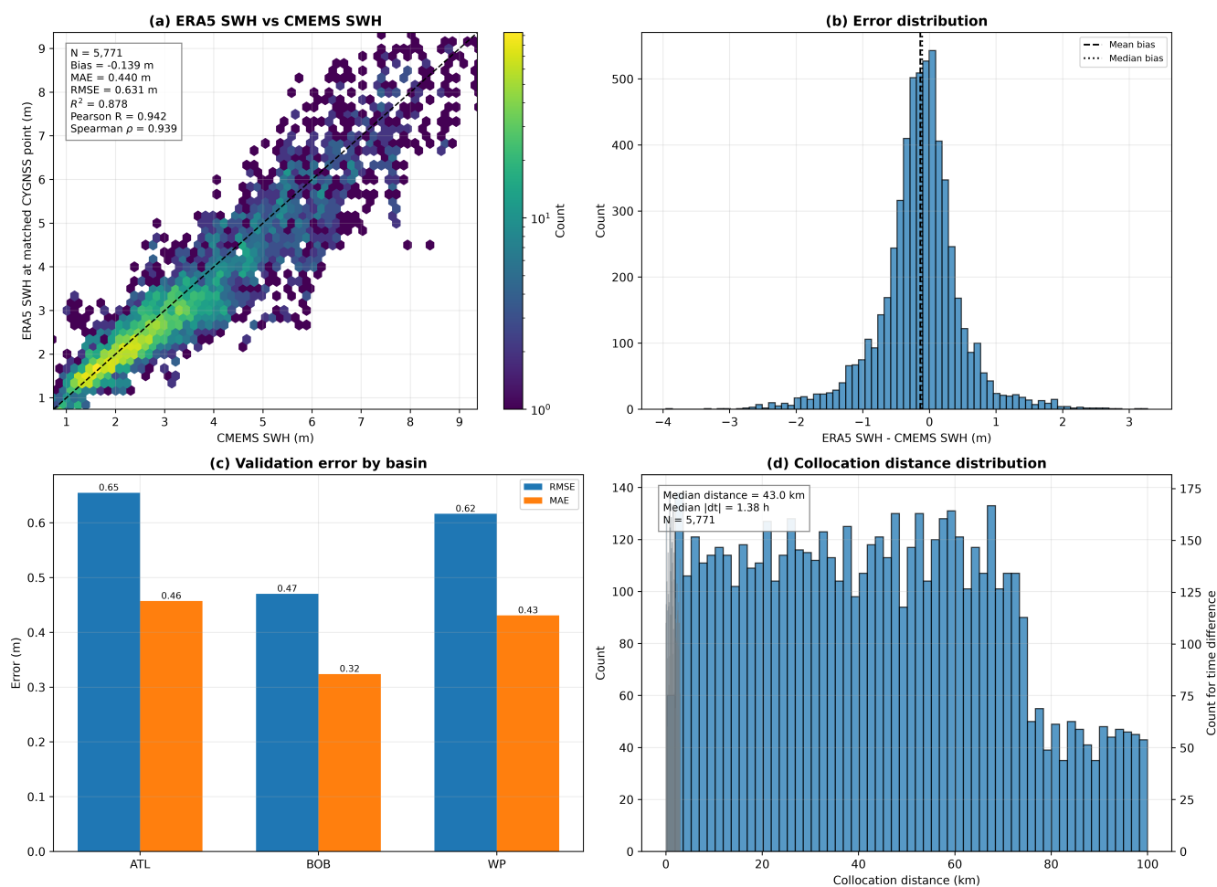
Figure 9. Independent validation of ERA5 significant wave height against CMEMS satellite-altimeter observations under the primary 100-km/3-h collocation criteria. Panels summarize the ERA5–CMEMS SWH relationship, SWH-difference distribution, regional validation statistics, and collocation-distance characteristics. The temporal separation of the retained matchups is reported together with the collocation diagnostics. Sensitivity to stricter space–time criteria is evaluated separately in the accompanying text.
