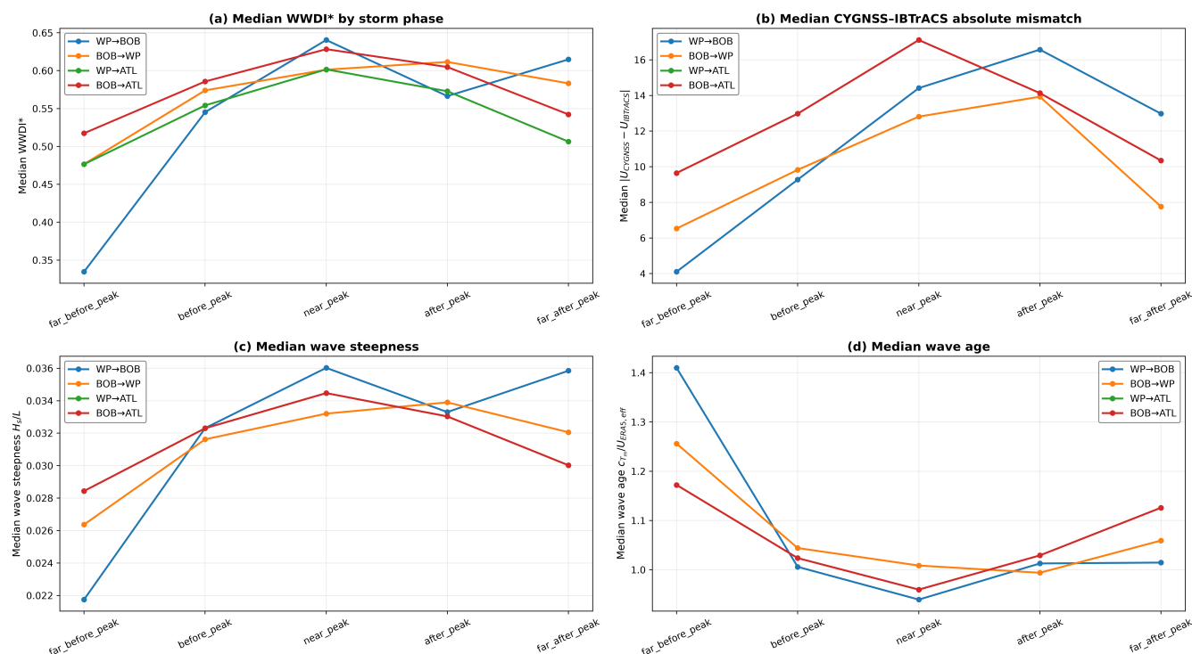
Figure 10. Storm-centred evolution of WWDI*, absolute CYGNSS–IBTrACS mismatch, wave steepness, and wave age relative to the tropical-cyclone intensity peak.
